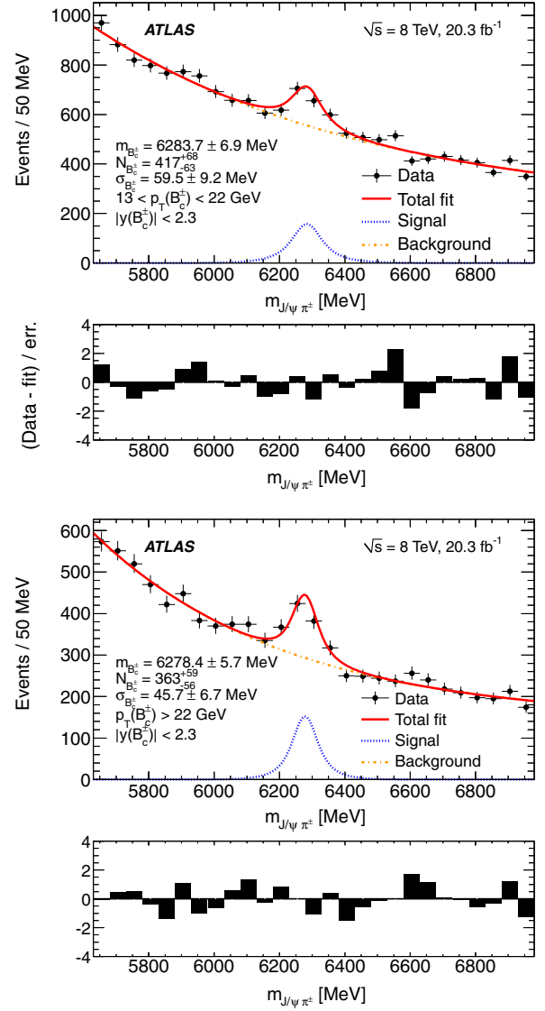
FIG. 4. The projection of the fit of the invariant mass distribution for the B_c^\pm meson. “Signal” stands for the signal component of the fit, “Background” stands for the combinatorial background component of the fit, and “Total fit” stands for the fit to the sum of the signal and background components. The fit for the low transverse momentum bin ( 13 \text{ GeV} < p_T(B_c^\pm) < 22 \text{ GeV} ) is shown at the top, and that for the high transverse momentum bin ( p_T(B_c^\pm) > 22 \text{ GeV} ) at the bottom. The rapidity requirement is |y(B_c^\pm)| < 2.3 . The fits are used to extract N^{\text{reco}}(B_c^+) + N^{\text{reco}}(B_c^-) and its uncertainty in each bin. The inset below each plot shows the bin-by-bin difference between the data point and the value obtained from the fit function divided by the quadrature sum of the statistical uncertainty and the systematic uncertainties obtained from varying the fit model.
