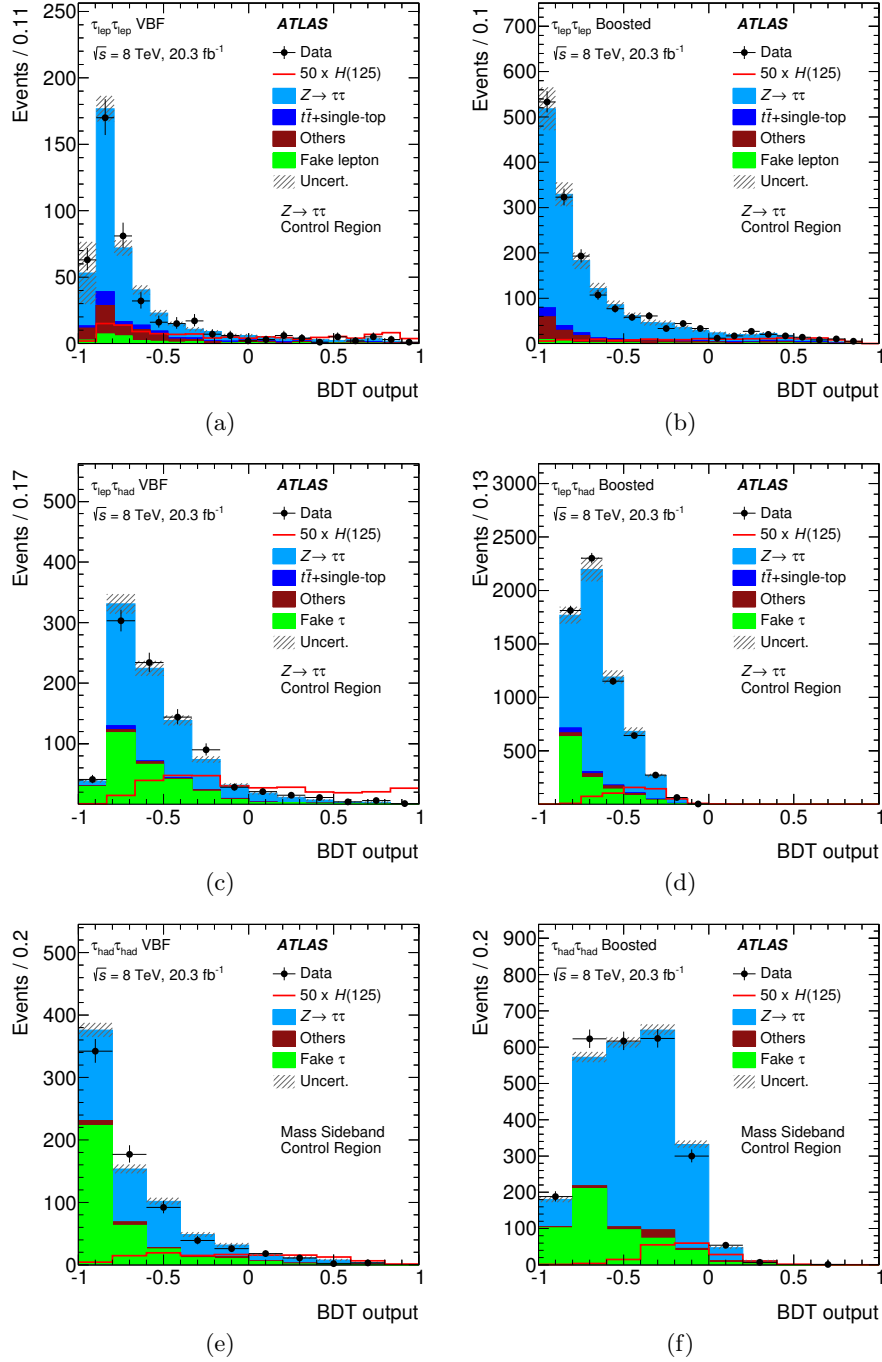
Figure 7. Distributions of the BDT output for data collected at \sqrt{s} = 8 TeV, compared to the expected background contributions in ATLAS. The distributions are shown for the VBF (left) and boosted (right) categories (a,b) for the Z \rightarrow \tau\tau -enriched control region in the \tau_{\text{lep}}\tau_{\text{lep}} channel, (c,d) for the Z \rightarrow \tau\tau -enriched control region in the \tau_{\text{lep}}\tau_{\text{had}} channel and (e,f) for the \tau\tau invariant mass sideband control region in the \tau_{\text{had}}\tau_{\text{had}} channel. The contributions from a Standard Model Higgs boson with m_H = 125 GeV are superimposed, multiplied by a factor of 50. These figures use background predictions made without the global fit defined in section 8. The error band includes statistical and pre-fit systematic uncertainties.
