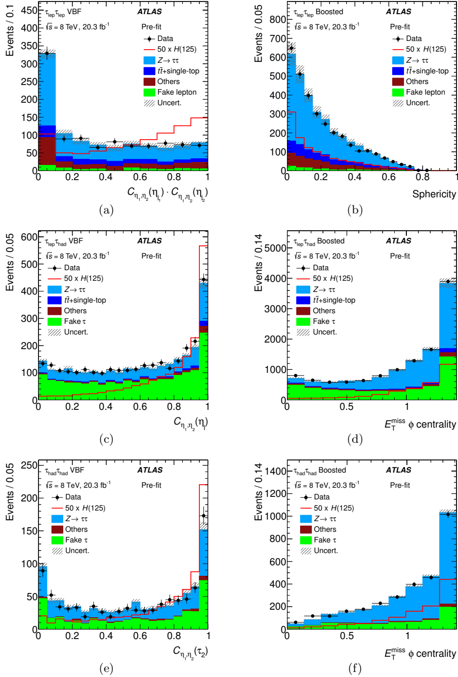
Figure 3. Distributions of important BDT input variables for the three channels and the two categories (VBF, left) and (boosted, right) for data collected at \sqrt{s} = 8 \text{ TeV} . The distributions are shown for (a) the product of the lepton centralities, C_{\eta_1, \eta_2}(\eta_{\ell_1}) \cdot C_{\eta_1, \eta_2}(\eta_{\ell_2}) , and (b) the sphericity in the \tau_{\text{lep}}\tau_{\text{lep}} channel, for (c) the centrality of the lepton, C_{\eta_1, \eta_2}(\eta_{\ell}) , and (d) the E_T^{\text{miss}} \phi centrality in the \tau_{\text{lep}}\tau_{\text{had}} channel, and for (e) the centrality of the subleading tau, C_{\eta_1, \eta_2}(\eta_{\tau_2}) , and (f) the E_T^{\text{miss}} \phi centrality in the \tau_{\text{had}}\tau_{\text{had}} channel. The contributions from a Standard Model Higgs boson with m_H = 125 \text{ GeV} are superimposed, multiplied by a factor of 50. These figures use background predictions made without the global fit defined in section 8. The error band includes statistical and pre-fit systematic uncertainties.
