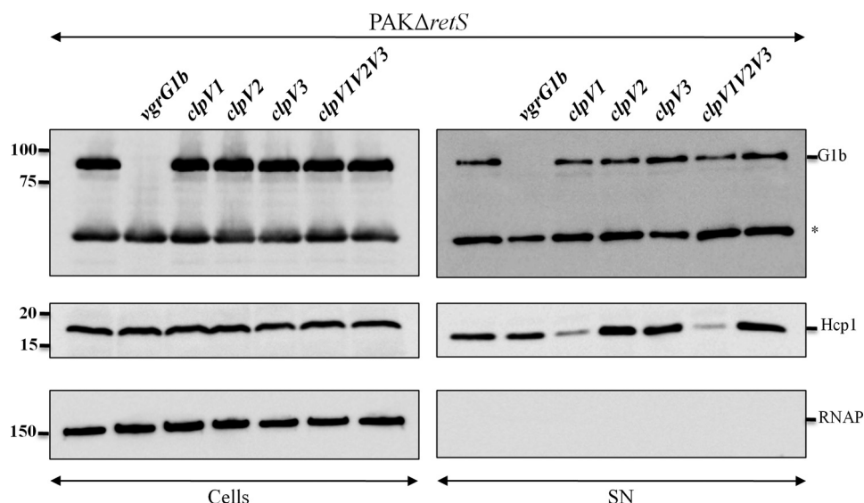
FIGURE 5. T6SS-independent secretion of VgrG1b. Whole cell extracts ( Cells ) and proteins from culture supernatants ( SN ) of PAK \Delta retS, vgrG1b , and clpV mutant derivatives ( clpV1 , clpV2 , clpV3 , or triple clpV1V2V3 ; indicated above each lane) were analyzed by immunoblotting. VgrG1b proteins were detected using antibodies directed against VgrG1b. Hcp1 was detected with anti-Hcp1 antibodies. Cytoplasmic RNAP was detected using an antibody directed against its \beta subunit. The positions of VgrG1b ( G1b ), Hcp1, and RNAP are indicated on the right. The band marked with an asterisk represents an uncharacterized protein recognized by antibodies directed against VgrG1b. Molecular mass standards (kDa) are indicated on the left.
