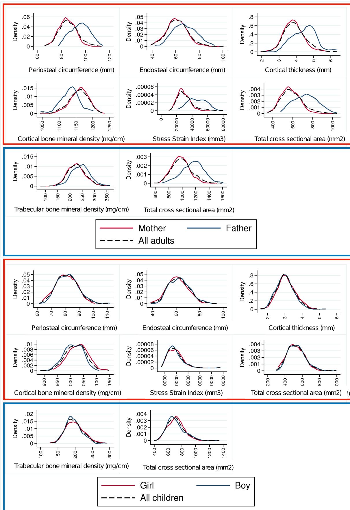
Figure 2 Density plots of adult and child peripheral quantitative CT parameters. Females (red), males (blue) and both sexes (thin dotted black line) plotted on the same graph for each outcome. X and Y scales common between child and parent.
