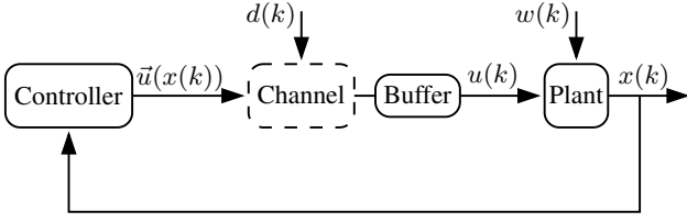
Fig. 1. NCS Architecture with Packet Dropouts and Buffering
