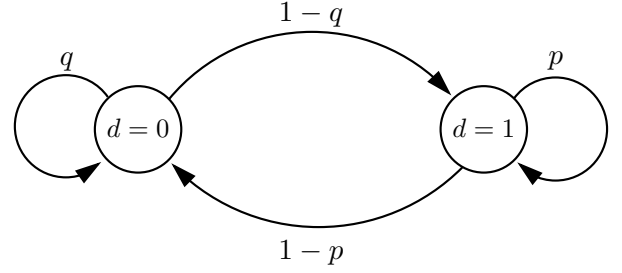
Fig. 2. Markov Packet Dropout Model
