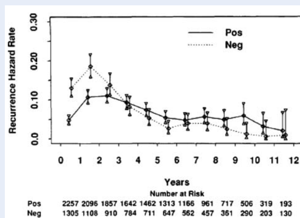
Figure 1 Annual hazard of recurrence of 3563 patients separated by ER status. ER, estrogen receptor.
