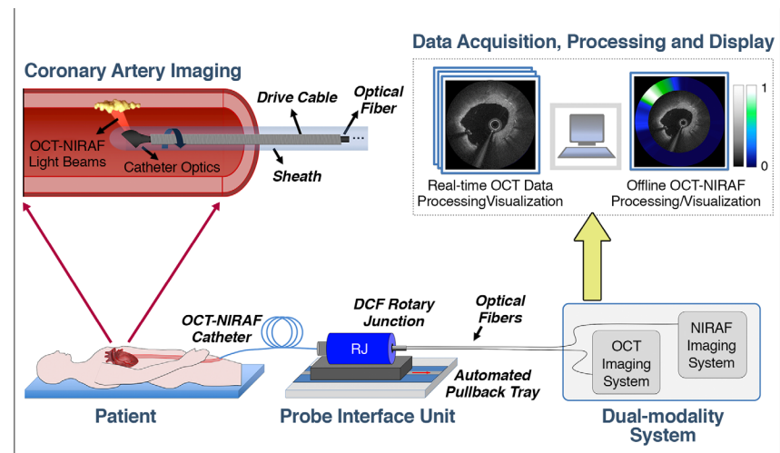
Figure 22. Schematic of the OCT-NIRAF system. OCT-NIRAF imaging was performed using a dual OCT-NIRAF catheter placed into the coronary artery of patients undergoing percutaneous coronary intervention (PCI). The mechanical procedure is fundamentally the same as standalone OCT. Dual imaging is accomplished by focusing OCT and NIRAF excitation light from the catheter tip to the arterial wall. The probe can image at 100 frames per second and NIRAF is detected using an excitation wavelength of 633 nm with signal acquisition in the 675-900 nm window. Three-dimensional OCT and NIRAF images are obtained simultaneously, collected by computer and processed. OCT data is displayed in real time whereas NIRAF data is processed and displayed offline as two dimensional NIRAF maps and as dual-modality OCT-NIRAF images. Reprinted from Ughi et al., 2016, JACC. Cardiovascular Imaging, 9(11), 1304–1314, with permission from Elsevier.
