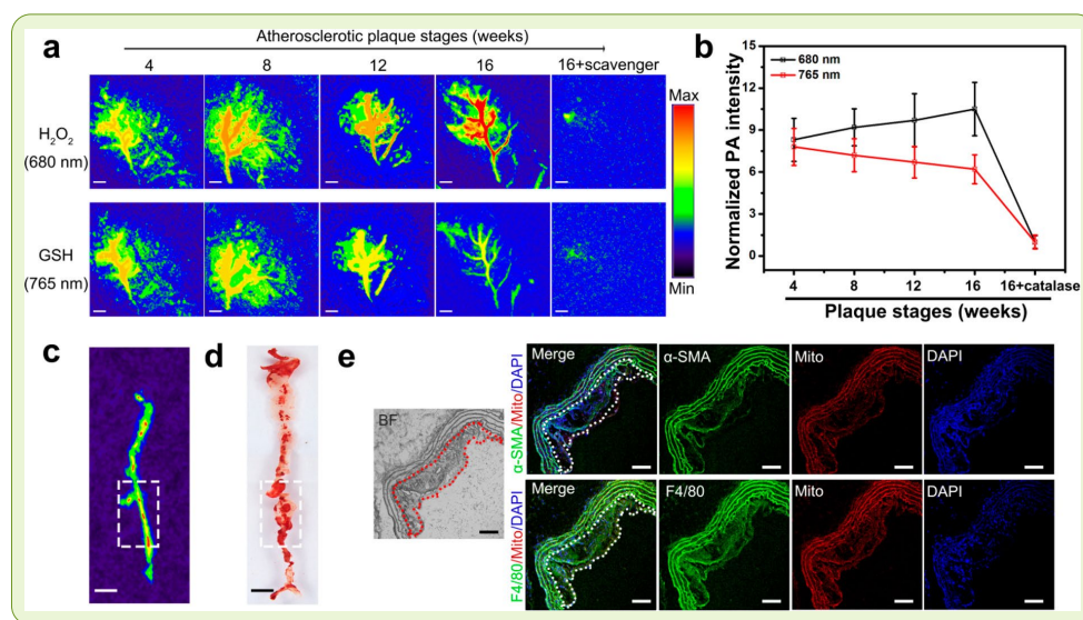
Figure 26. In vivo PAI of atherosclerotic plaque in apoE -/- mice. (A) PAI of abdominal aortas at different stages of pathology following BSA-Cy-Mito injection (10 mg/kg). Some mice were also treated with scavengers (catalase for H 2 O 2 and BSO for GSH). Scale bar = 2 mm. (B) Normalized photoacoustic (PA) signal derived from (A). Data shown as mean ± SD (n = 3). (C) Representative ex vivo PAI of the aorta from 16 weeks high fat diet fed mice. Scale bar = 5 mm. (D) Representative images of atherosclerotic lesions stained with Oil-Red-O. White dashed lines represent abdominal aorta. Scale bar = 5 mm. (E) Bright field and immunofluorescent images of aortic plaque cross sections in mice fed high fat diet for 16 weeks. Dashed line indicates lesion border. Scale bar = 100 μm. Reproduced from Gao et al., 2019, Analytical chemistry, 91(1), 1150–1156. Copyright American Chemical Society.
