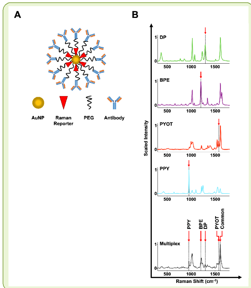
Figure 29. Design and characterisation of biofunctionalized SERS nanoparticles. (A) Schematic depicting a solid gold NP core (AuNP) conjugated to Raman reporter molecules; this Raman reporter covered core was then conjugated with antibody-functionalized polyethylene glycol (PEG) to increase biocompatibility and increase circulating residence times. (B) Raman spectrum from 4 distinct SERS NPs. From top to bottom: Isotype labelled NPs with DP Raman reporter; anti-ICAM-1 NPs with BPE Raman reporter; anti-VCAM-1 NPs with PYOT Raman reporter; anti-P-selectin NPs with PPY Raman reporter and an example of a SERS multiplex spectra containing each distinct combination. Red arrows indicate peaks unique to each Raman reporter and also a common peak present in each (1605 cm -1 ). Reproduced from: Noonan et al., 2018, distributed under the terms of a Creative Commons Attribution (CC BY) license ( https://creativecommons.org/licenses/by/4.0/ ).
