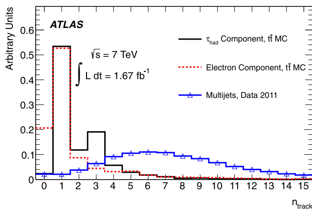
Fig. 1 Distribution of n_{\text{track}} for \tau_{\text{had}} from MC t\bar{t} events (solid black line), electrons from MC t\bar{t} events (dashed red line), and for jets from multijet events from data (blue triangles). The multijet event selection uses a S_{E_T^{\text{miss}}} sideband region as described in Sect. 5. All distributions are normalised to unity (Color figure online)
