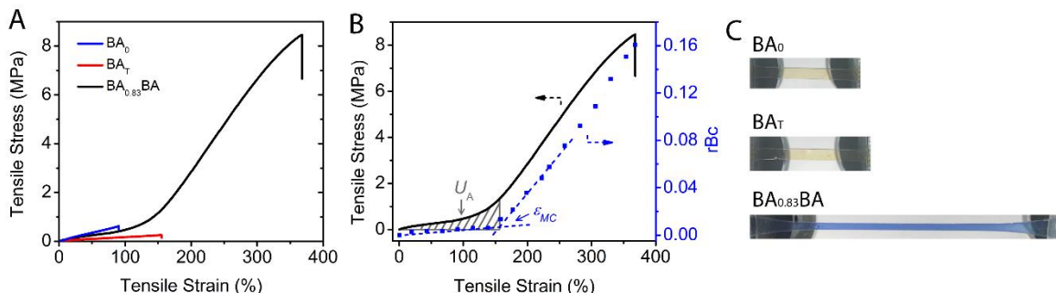
Figure 1. (A) Tensile stress-strain curves of SNs prepared in the presence/absence of toluene ( BA_T and BA_0 ) and DN ( BA_{0.83}BA ). (B) A plot of rBc as a function of tensile strain for BA_{0.83}BA with \epsilon_{MC} determined by the intersection of two tangent lines. The color activation energy U_A is calculated by integration of the area underneath the onset of color change on stress-strain curve. (C) Images of the two SNs and DN BA_{0.83}BA under tension prior to fracture.
