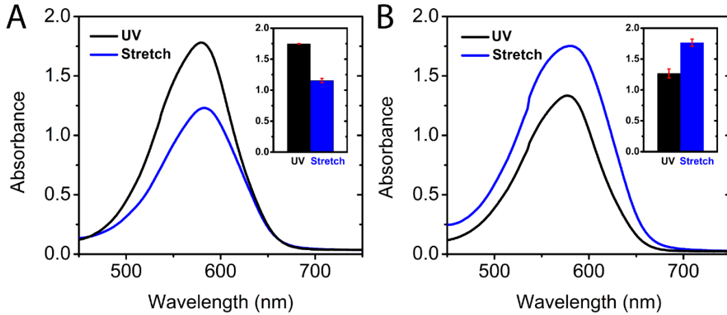
Figure 6. Absorbance spectra of (A) BA 0.83 BA and (B) BA 0.83 MA activated by UV light until plateaued and by stretching upon fracture. The inset figures present the absorbance intensity at the peak wavelength at 580 nm.
