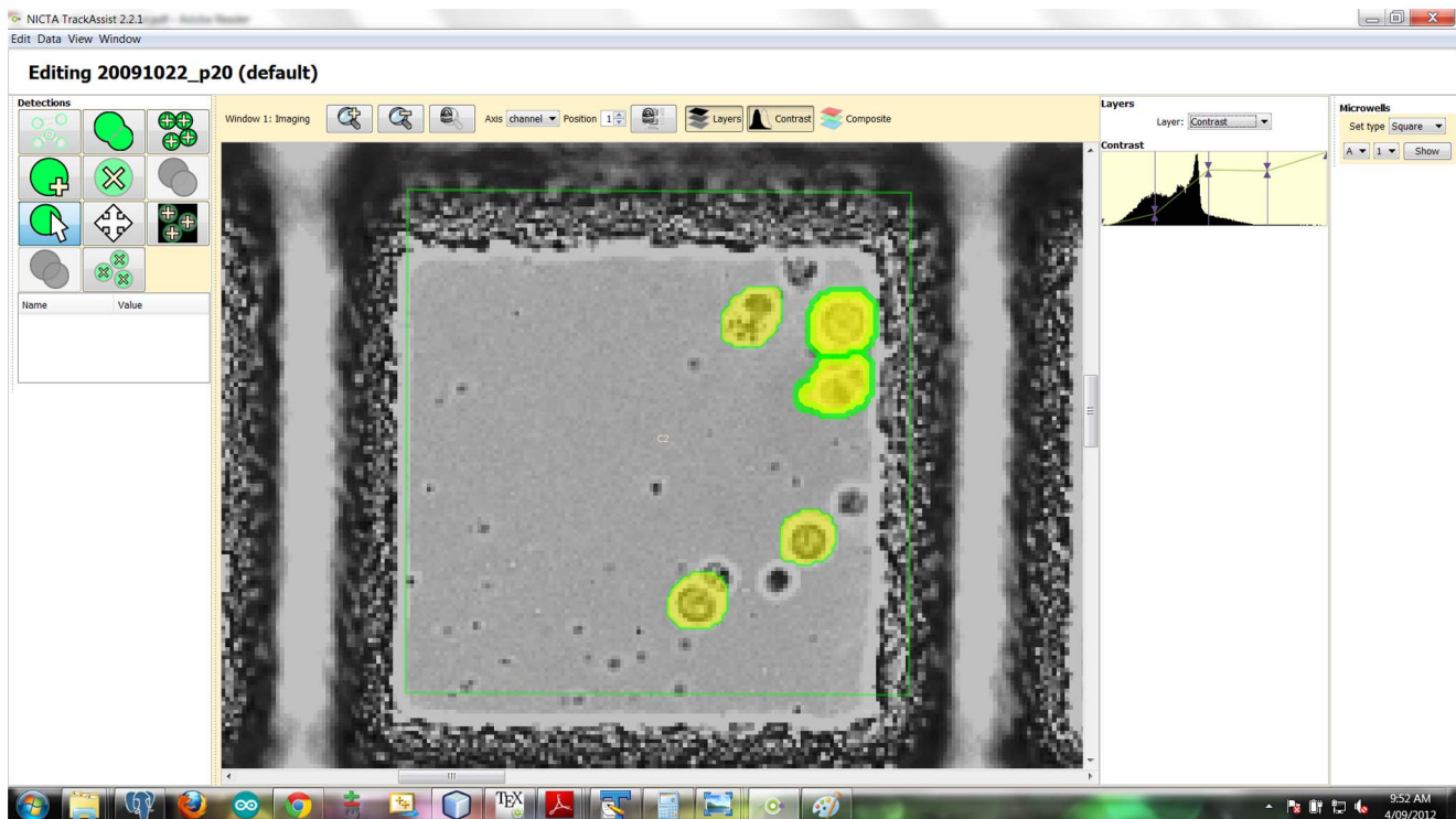
Figure 12. Graphical user interface of the TrackAssist software. The bright field is shown here, with histogram based manual contrast enhancement for viewing purposes. Five segmented cells are shown, two of which are selected. Other objects in the well are debris. The detection editing tools are shown in a panel on the left. In row-major order from top-left, these are: De-select all tracks and detections; merge selected detections; automatically create detections (by background modelling and motion detection); create detection; delete selected detections; cut brush from selected detection contour; select detections; move detection; automatically create detections (based on thresholded constant fluorescence); add brush area to selected detection contour; delete all detections in range of images. doi:10.1371/journal.pone.0083251.g012
