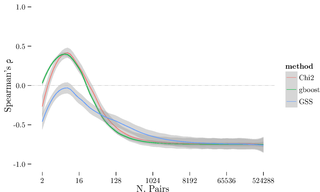
Figure 1. Spearman's \rho for all three methods ( \chi^2 , GSS, and GBOOST) on BD dataset. On this dataset, GSS fails to obtain a stable set of pairs on average. GBOOST and \chi^2 both have similar profiles and show similar ZIC points. Note that while the peaks for GBOOST and \chi^2 occur at approximately the same number of pairs, the higher \rho for GBOOST indicates better stability of the ordering within the stable set. doi:10.1371/journal.pone.0093319.g001
