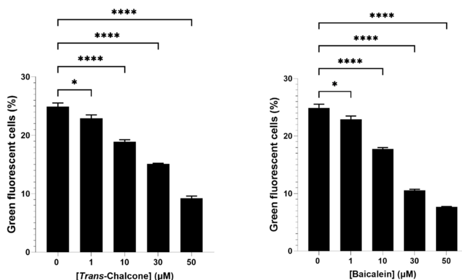
Figure 2. Population of BY4743 \Delta\text{ahp1} [p416.GPD.GFP- \text{Ab}_{42} ] with green fluorescence following exposure to trans -chalcone (left panel) and baicalein (right panel). Statistically significant values obtained from one-way ANOVA test in reference to untreated control are represented by asterisks (* p < 0.05 and **** p < 0.0001 ).
