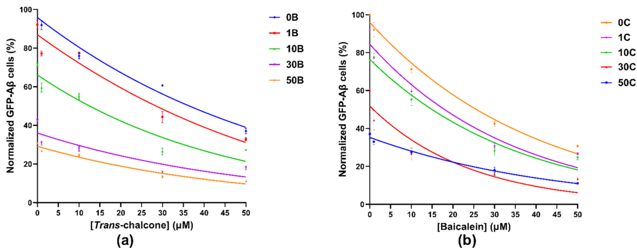
Figure 3. Gaussian curves obtained by plotting the normalized GFP- \text{Ab}_{42} positive cells in percentages when the BY4743 \Delta\text{ahp1} [p416.GPD.GFP- \text{Ab}_{42} ] cells were treated with (a) combinations of 0, 1, 10, 30 and 50 \mu\text{M} trans -chalcone with constant concentrations of baicalein at 0, 1, 10, 30 and 50 \mu\text{M} represented by curves 0B, 1B, 10B, 30B and 50B, respectively, and (b) combinations of 0, 1, 10, 30 and 50 \mu\text{M} baicalein with constant concentrations of trans -chalcone at 0, 1, 10, 30 and 50 \mu\text{M} represented by curves 0C, 1C, 10C, 30C and 50C, respectively. The total GFP- \text{Ab}_{42} producing cells in the untreated control were normalized to 100% and used for comparison with the treated populations.
