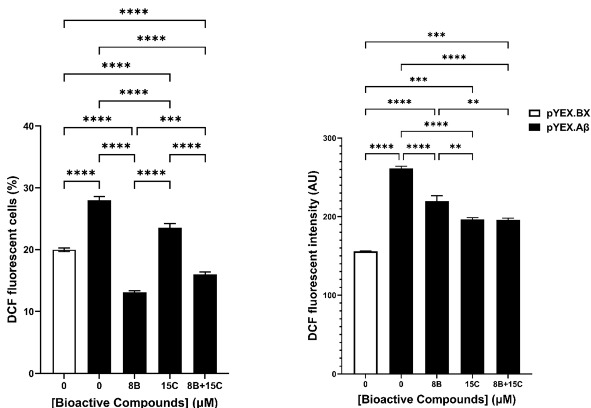
Figure 6. Effect on intracellular reactive oxygen species (ROS) in BY4743 [pYEX.A \beta ] cells treated with 8 \mu\text{M} baicalein (8B), 15 \mu\text{M} trans -chalcone (15C) and their combination (8B + 15C). pYEX.BX represents data obtained from BY4743 [pYEX.BX] empty vector control and pYEX.A \beta represents data obtained from BY4743 [pYEX.A \beta ] transformants. Left panel shows the change in percentage of dichlorofluorescein (DCF) fluorescent cells and right panel shows the median DCF fluorescence intensity differences between the treatments. Statistically significant values obtained by one-way ANOVA analysis are represented by asterisks (** p < 0.01 , *** p < 0.001 and **** p < 0.0001 ).
