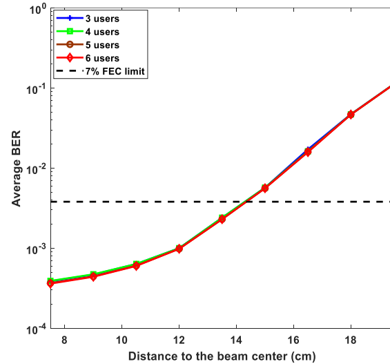
Fig. 7. Average BER performance of single-PD reception with different number of served users when the gross data rate is 10 Gb/s.
