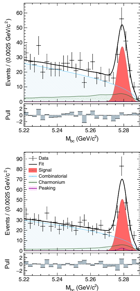
FIG. 1. Results of the combined B^+ and B^0 signal yield fit to the M_{bc} distributions for the electron (top) and muon (bottom) modes for q^2 > 0.045 \text{ GeV}^2/c^4 . Combinatorial (dashed blue), signal (red filled), charmonium (dashed green), peaking (purple dotted), and total (solid) fit distributions are superimposed on data (points with error bars).
