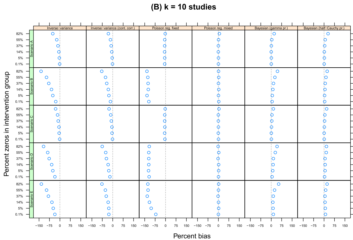
Figure 1 Percentage bias in the estimate of \hat{\rho}_{int} by number of studies, estimation method and percentage of zeros in the data. The true value is \log(0.2) = -1.609 and the estimates are unbiased if they fall along the x = 0 line. (A) k = 5 studies and (B) k = 10 studies.
