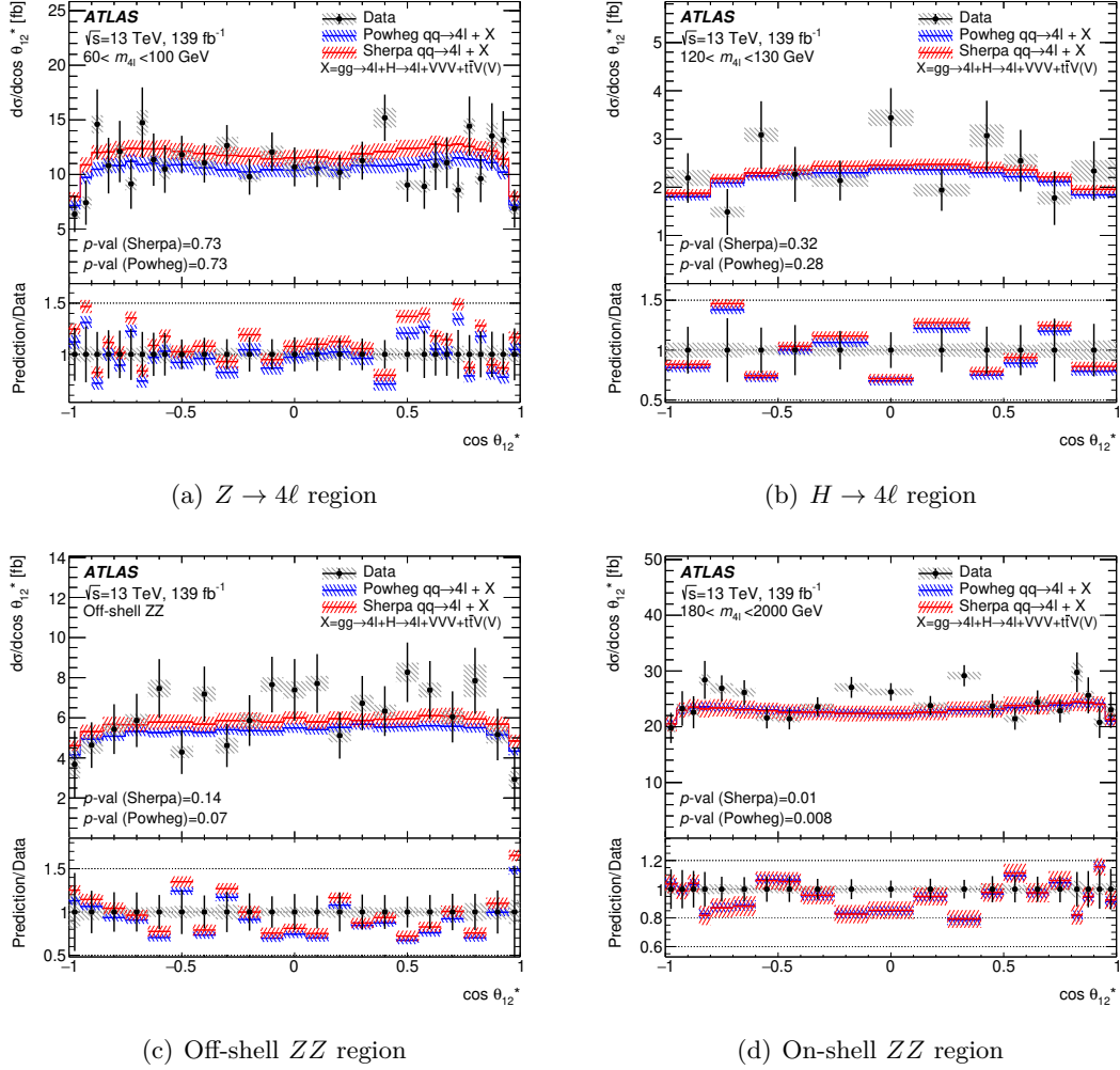
Figure 10. Differential cross-section as a function of \cos\theta_{12}^* in the four m_{4\ell} regions. The measured data (black points) are compared with the SM prediction using either SHERPA (red, with red hashed band for the uncertainty) or POWHEG + PYTHIA8 (blue, with blue hashed band for the uncertainty) to model the q\bar{q} \rightarrow 4\ell contribution. The error bars on the data points give the total uncertainty and the grey hashed band gives the systematic uncertainty. The p -value is the probability for the \chi^2 , with the number of degrees of freedom equal to the number of bins in the distribution, to have at least the observed value, given the SM prediction. The lower panel shows the ratio of the SM predictions to the data.
