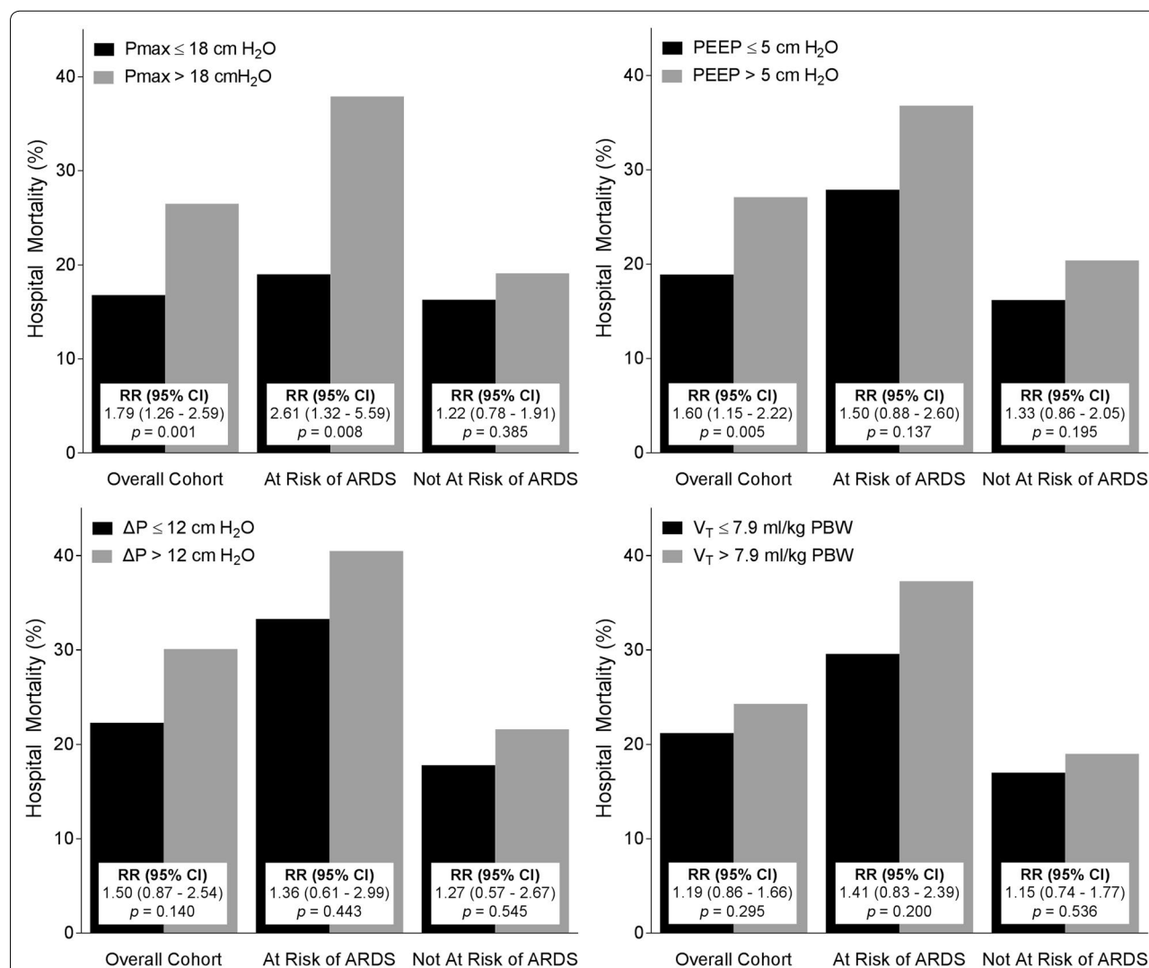
Fig. 2 Unadjusted relative risks of hospital mortality in the overall cohort and in patients at risk and not at risk of ARDS and according to the median of the: a P_{max} ; b PEEP; c \Delta P ; and d tidal volume. Abbreviations: P_{max} : maximum airway pressure; PEEP: positive end-expiratory pressure; V_T : tidal volume; \Delta P : driving pressure; RR: relative risk; CI: confidence interval
