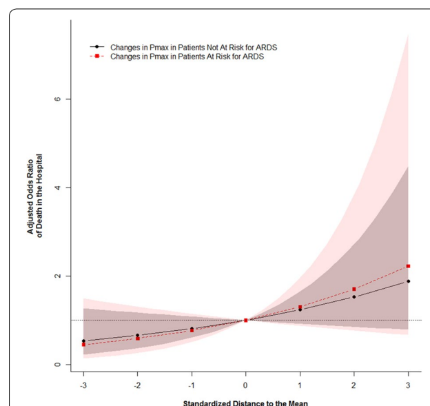
Fig. 3 Odds ratio of hospital mortality according to increases in one standard deviation of P_{\max} and in the patients at risk and not at risk of ARDS. All curves are adjusted by the same set of variables described in Table 3
