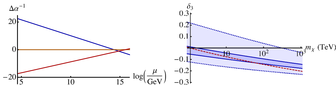
Figure 2. Left: the running differential SM gauge couplings in a composite Higgs model with 20 TeV top companions. \Delta\alpha_i^{-1} \equiv \alpha_i^{-1} - \alpha_2^{-1} . Right: the postdiction of the QCD gauge coupling as a function of the top companion mass: \delta_3 \equiv [\alpha_3^{\text{th}}(M_Z) - \alpha_3^{\text{ex}}(M_Z)]/\alpha_3^{\text{ex}}(M_Z) . The solid and dotted lines mark out the bands from the 4D calculation for b_{\text{strong}} = 1, 5 respectively, the dashed line the result of the 5D calculation.
