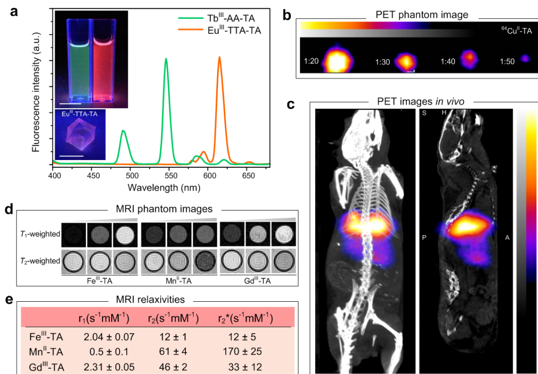
Figure 4. Engineering multifunctional MPN capsules for imaging. a) Normalized fluorescence spectra of capsule suspensions of Eu III -TTA-TA and Tb III -AA-TA excited at 360 nm. Insets are photographs of the corresponding capsule suspensions (top) and of PDMS coated with Eu III -TTA-TA (bottom) excited at 254 and 365 nm. Scale bars are 1 cm. b) Pseudo-colour PET phantom of suspensions of 64 Cu II -TA capsules at different dilution ratios (stock suspension concentration is 3.2 \times 10^8 capsules per ml with an activity of 1 MBq). c) Small-animal PET/CT image of an in vivo model 30 min after injection of 1 MBq 64 Cu II -TA capsules (maximum intensity projection (right), sagittal view (left)). d) MRI phantom images of capsule suspensions immobilized in agarose. Shown are T 1 -weighted inversion recovery images (with inversion time T i = 1,375 ms) and T 2 -weighted spin echo images (with echo time T E = 50 ms) of samples with three different metal concentrations: 0.02 mM, 0.1 mM and 0.3 mM (0.15 mM for Gd III -TA). e) Table of MRI relaxivities for Fe III -TA, Mn II -TA and Gd III -TA capsule suspensions measured with a 9.4 T animal MRI system.
