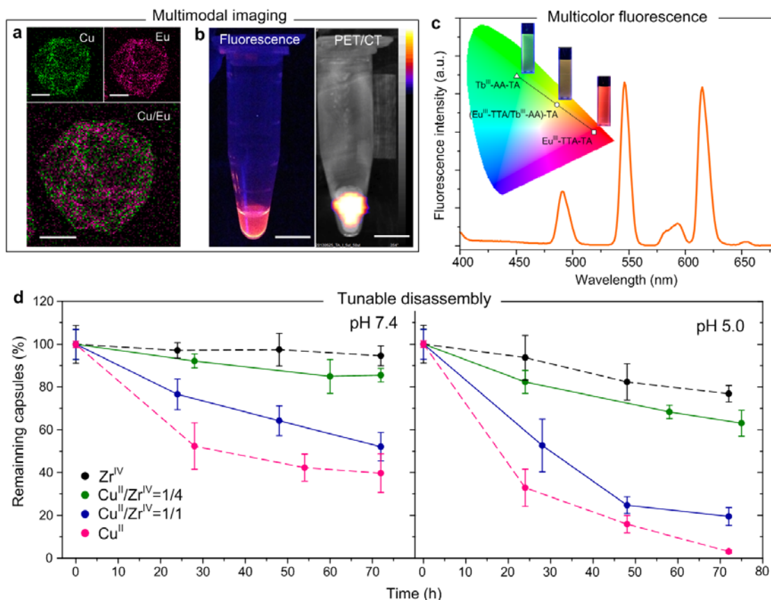
Figure 5. Hybrid dual metal MPN capsules for multimodal imaging, multicolour properties and tunable disassembly. a) EDX elemental mapping of dual metal (Cu II /Eu III -TTA)-TA capsules. Scale bar is 1 \mu m. b) Fluorescence (left) and PET/CT pseudo-colour (right) images of a suspension of ( 64 Cu II /Eu III -TTA)-TA capsules. Scale bars are 1 cm. c) Normalized fluorescence spectra for (Eu III -TTA/Tb III -AA)-TA capsule suspensions excited at 312 nm. Insets are fluorescence images of Eu III -TTA-TA, Tb III -AA-TA and (Eu III -TTA/Tb III -AA)-TA capsule suspensions and the corresponding locations on the CIE 1931 chromaticity diagram. d) pH-dependent disassembly kinetics of Cu II -TA, Zr IV -TA and hybrid Cu II /Zr IV -TA capsules at different pH, as assessed by flow cytometry. Data are means \pm SD (N = 3).
