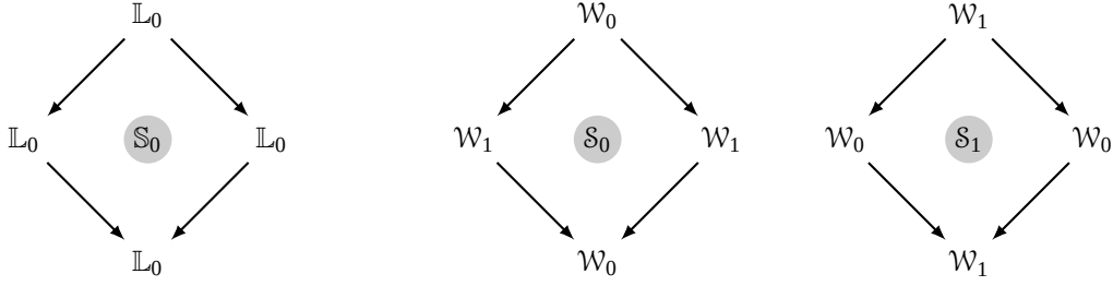
FIGURE 4. The Loewy diagrams for the socle series of the indecomposable symplectic fermion module \mathbb{S}_0 (left) and the indecomposable \mathfrak{W}(1,2) -modules \mathbb{S}_0 and \mathbb{S}_1 (right). In each case, the non-diagonalisable action of L_0 maps the top factor (the head) onto the bottom factor (the socle).
