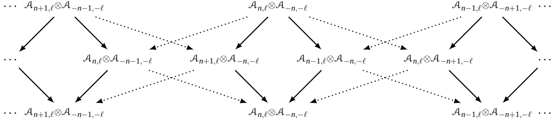
FIGURE 13. A part of the Loewy diagrams for the atypical bulk modules \mathcal{J}_{n,e} corresponding to the charge-conjugate modular invariant partition function. We have neglected to indicate relative parities because the conjugate of an atypical \mathcal{A}_{n,e} changes parity unless e = 0 .
