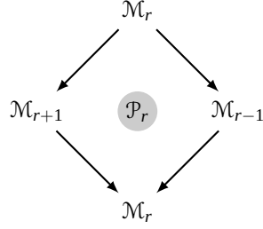
FIGURE 5. Conjectured Loewy diagram for the proposed indecomposable \mathfrak{M}(1,2) -module \mathcal{P}_r .
