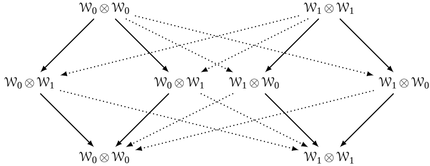
FIGURE 7. The Loewy diagram for the indecomposable bulk module \mathcal{B} of \mathfrak{W}(1,2) \oplus \mathfrak{W}(1,2) . The solid/dotted arrows indicate the action of the holomorphic/antiholomorphic triplet algebra. It is clear that restricting to each chiral subalgebra results in \mathcal{B} decomposing as (\mathcal{W}_0 \otimes \mathcal{S}_0) \oplus (\mathcal{W}_1 \otimes \mathcal{S}_1) and (\mathcal{S}_0 \otimes \mathcal{W}_0) \oplus (\mathcal{S}_1 \otimes \mathcal{W}_1) , respectively.
