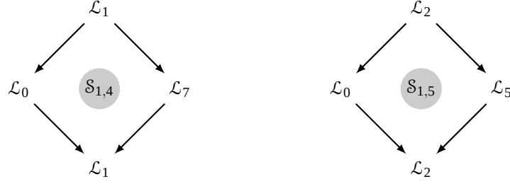
FIGURE 2. Loewy diagrams illustrating the socle series (see Appendix A.4) for the indecomposable Virasoro modules \mathcal{S}_{1,4} and \mathcal{S}_{1,5} constructed using the Nahm-Gaberdiel-Kausch fusion algorithm.
