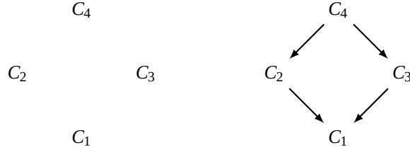
FIGURE 14. An example of a Loewy diagram (left) and its annotated version (right).
