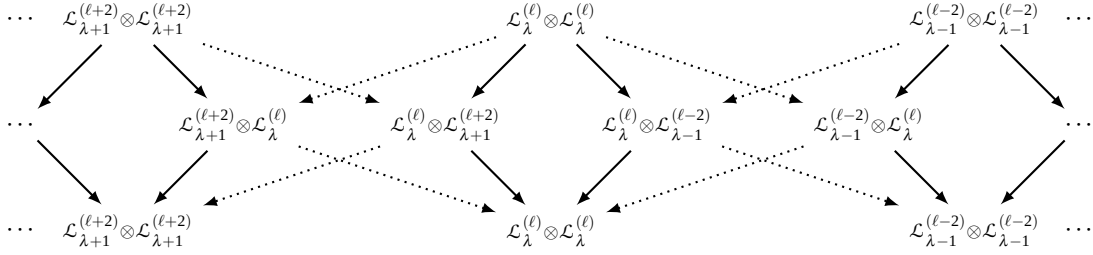
FIGURE 10. A part of the (proposed) Loewy diagrams for the atypical bulk modules. Taking \lambda = 0 \bmod 2 and \ell = 0, 1, 2, 3 \bmod 4 gives the diagrams for \mathcal{B}_0 , \mathcal{B}_{-1/2;+} , \mathcal{B}_1 and \mathcal{B}_{-3/2;+} , respectively.
