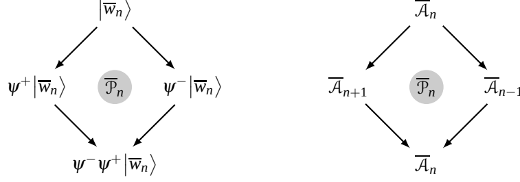
FIGURE 11. The projective cover \overline{\mathcal{P}}_n of the \mathfrak{gl}(1|1) -module \overline{\mathcal{A}}_n , illustrated by its states on the left and by its Loewy diagram on the right.
