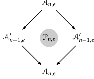
FIGURE 12. The Loewy diagram of the indecomposable \widehat{\mathfrak{gl}}(1|1) -module \mathcal{P}_{n,e} .
