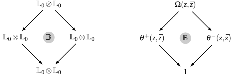
FIGURE 6. On the left, the Loewy diagram of the bulk indecomposable module \mathbb{B} (over the direct sum of two copies of the symplectic fermion algebra). On the right, the same diagram but with the bulk composition factors replaced by the fields naturally associated to them.
