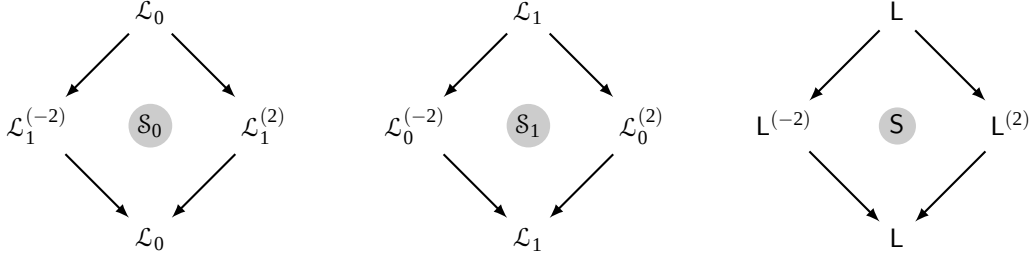
FIGURE 9. Loewy diagrams for the indecomposable \widehat{\mathfrak{sl}}(2)_{-1/2} -modules S_0 and S_1 (left) and the indecomposable \beta\gamma ghost module S (right).
