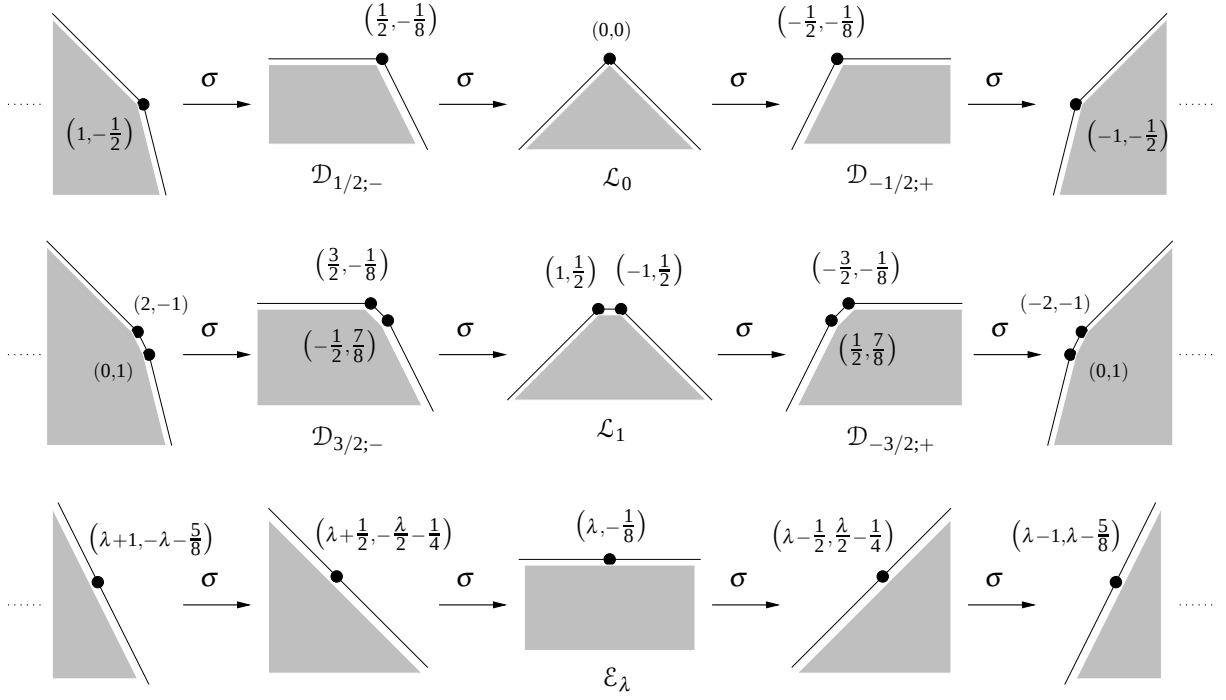
FIGURE 8. Depictions of the physical irreducible \widehat{\mathfrak{sl}}(2)_{-1/2} -modules. Each labelled state declares its weight and conformal dimension (in that order). Conformal dimensions increase from top to bottom and \mathfrak{sl}(2) -weights increase from right to left.
