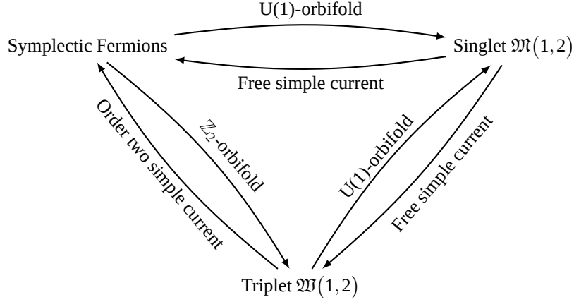
FIGURE 3. The symplectic fermion algebra, the triplet algebra \mathfrak{W}(1,2) and the singlet algebra \mathfrak{M}(1,2) are all related by simple current extensions and orbifolds.
