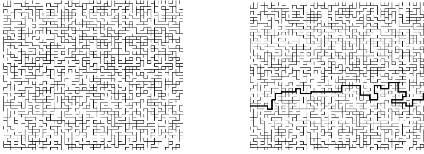
FIGURE 1. A typical percolation configuration (left) for a rectangular subdomain of a square lattice showing only the open edges (closed edges are omitted). This lattice has several crossings from left to right, one of which is indicated in bold (right).
