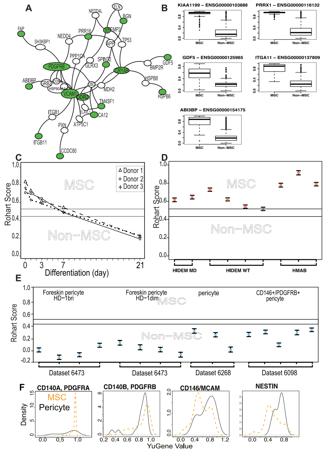
Figure 3 The MSC signature forms part of a network of extracellular proteins and discriminates between differentiating or related adult stem cell types. (A) An extended protein-protein network diagram of the Rohart MSC signature genes demonstrating a role for VCAM1 and PDGFRB as part of a functionally interconnected set of glycoproteins, integrins, growth factors and extracellular matrix proteins. Green nodes are seed network members from component (continued on next page...)
