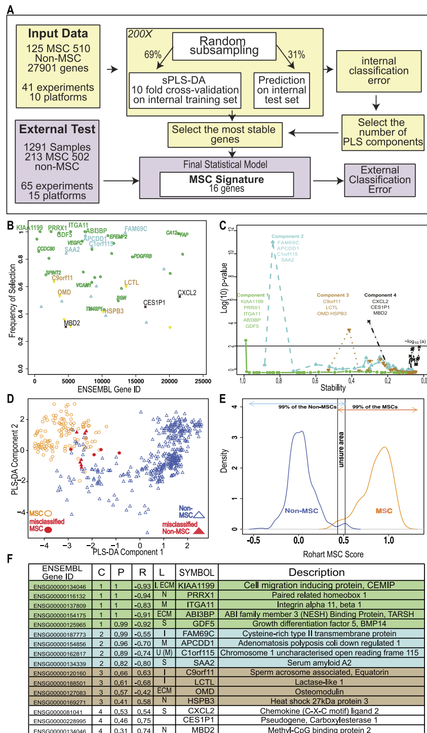
Figure 2 An improved in silico MSC signature. (A) Workflow summarizing the modified implementation of the PLS-DA to integrate and evaluate cross-platform studies for derivation of a stable classifier; (B) Evaluation of the stability of each gene across four components, where frequency of selection over 200 subsamplings (Y-axis) is shown per gene (ENSEMBL ID, X-axis). Labels are provided for the 16 genes contributing to the signature across 4 components. Component 1 (green), (continued on next page...)
