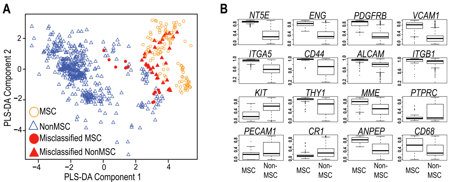
Figure 1 Evaluation of Common MSC markers as transcriptional classifiers. (A) PLS-DA scatter plot of MSC (circles) and non-MSC cell types (triangles). Red symbols indicate cells which are incorrectly classified by the PLS-DA matrix. The matrix components consisted of 32 commonly used MSC markers. (B) Box and Whisker plots showing average expression of common MSC markers that are significantly differentially expressed ( t -test, P > 10^{-6} ) between MSC ( n = 125 ) and non-MSC ( n = 510 ) cell types. See also Fig. S1 and Table S1.
