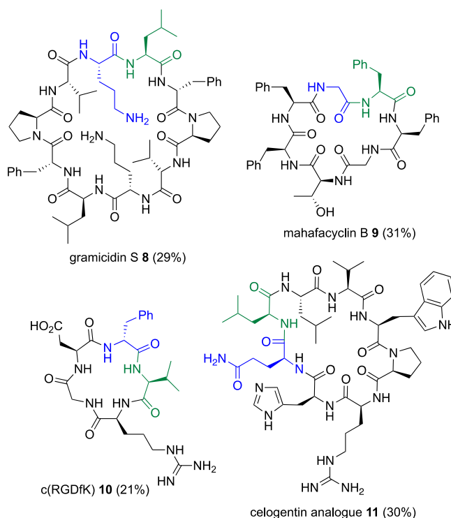
Figure 2. Diverse examples of cyclic peptides synthesized by Ag(I)-promoted thioamide cyclization (overall yields from starting resin shown in parentheses).
