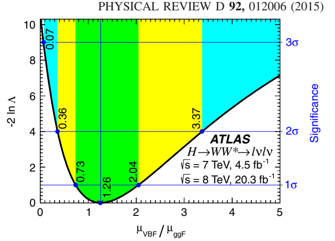
FIG. 39 (color online). Likelihood scan as a function of \mu_{\text{VBF}}/\mu_{\text{ggF}} for m_H = 125.36 GeV. The value of the likelihood at \mu_{\text{VBF}}/\mu_{\text{ggF}} = 0 gives the significance of the VBF signal at 3.2 standard deviations. The inner (middle) [outer] band shaded darker (lighter) [darker] represents the one (two) [three] standard deviation uncertainty around the central value represented by the vertical line.
