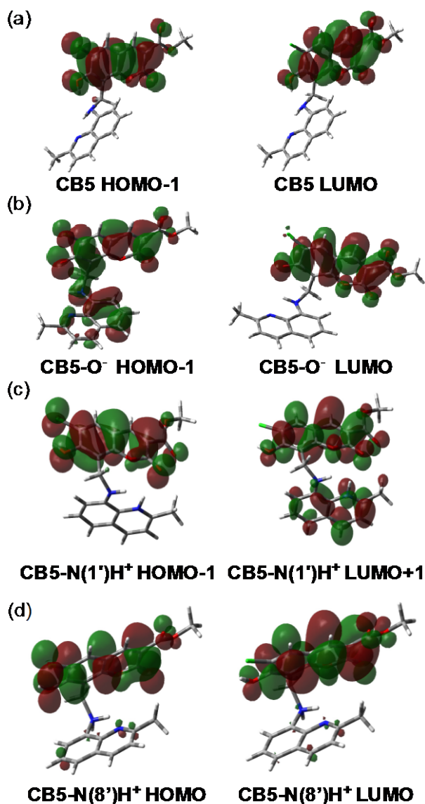
Figure 4. MO pairs with dominant contributions to the \lambda_{\max} TD-DFT excitations of (a) CB5 , (b) CB5-O - , (c) CB5-N(1')H + and (d) CB5-N(8')H + displayed with an isovalue of ca. 0.02 e - /Å (TD-CAM-B3LYP/6-311G** level of theory). [36]
