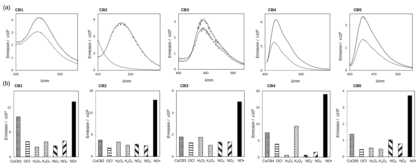
Figure 6. (a) Fluorescence quenching of CB1-5 by addition of equimolar amounts of \text{CuCl}_2 (100 \mu\text{M} in TBS at pH 7 with 1% DMSO) CB1-5 (solid line) and Cu(II)-CB1-5 (dotted line). (b) Selectivity of Cu(II)-CB1-5 towards \text{NO}^\bullet and a series of RNS and ROS (100 \mu\text{M} in TBS at pH 7 with 1% DMSO; 400 equiv. of oxidant). The reactions with CB2 in (a) and (b) were performed in neat DMSO.
