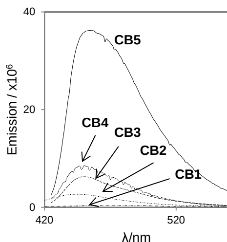
Figure 1. Fluorescence emission intensities of CB1-5 at pH 7 (100 \mu M in TBS, with 1% DMSO; \lambda_{\text{ex}} = 410 nm ( CB1,3-5 ) or 360 nm ( CB2 )).
