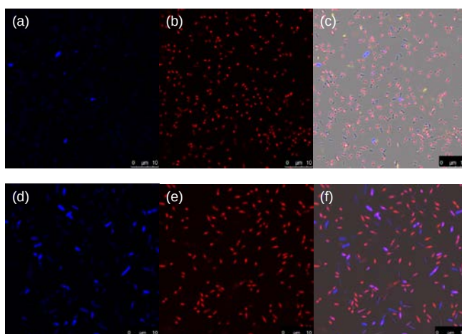
Figure 7. NO • detection in 24-hour P. aeruginosa biofilms that were up-regulated for NO • production using confocal laser-scanning microscopy. NO • detected with CB4 (a) and CB5 (d); HCS stained live and dead cells in the presence of CB4 (b) and CB5 (e); overlaid images of CB4 and HCS (c) and CB5 and HCS (f).
