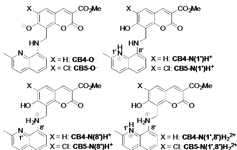
Figure 2. O-Deprotonated and N-protonated isomers of CB4 and CB5 .
