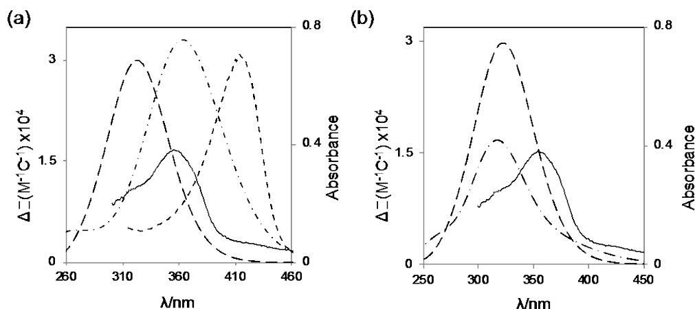
Figure 5. (a) Simulated UV/vis spectrum (left y-axis) of CB5 (---) and CB5-O - (-.-) vs. the experimentally measured absorbance (right y-axis) at pH 1 (—) and pH 7 (- - -). (b) Simulated UV/vis spectrum (left y-axis) of CB5 (---) and CB5-N(1')H + (-.-) vs. the experimentally measured absorbance (right y-axis) at pH 1 (—).
