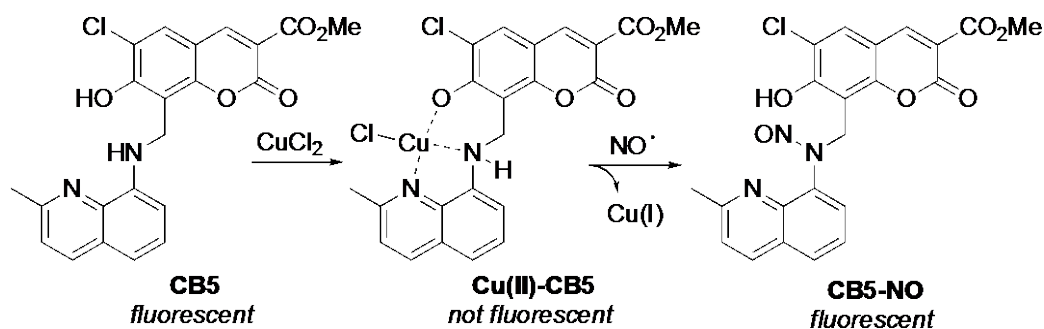
Scheme 1. Mechanism of “turn-on” fluorescence through replacement of Cu(II) by NO • in the recently developed coumarin based probe CB5 . [20]
