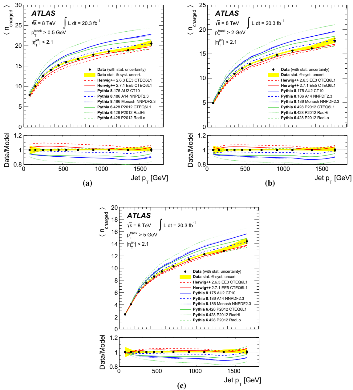
Fig. 4 The measured average charged-particle multiplicity as a function of the jet p_T , combining the more forward and the more central jets for a p_T^{\text{track}} > 0.5 GeV, b p_T^{\text{track}} > 2 GeV, and c p_T^{\text{track}} > 5 GeV. The band around the data is the sum in quadrature of the statistical
