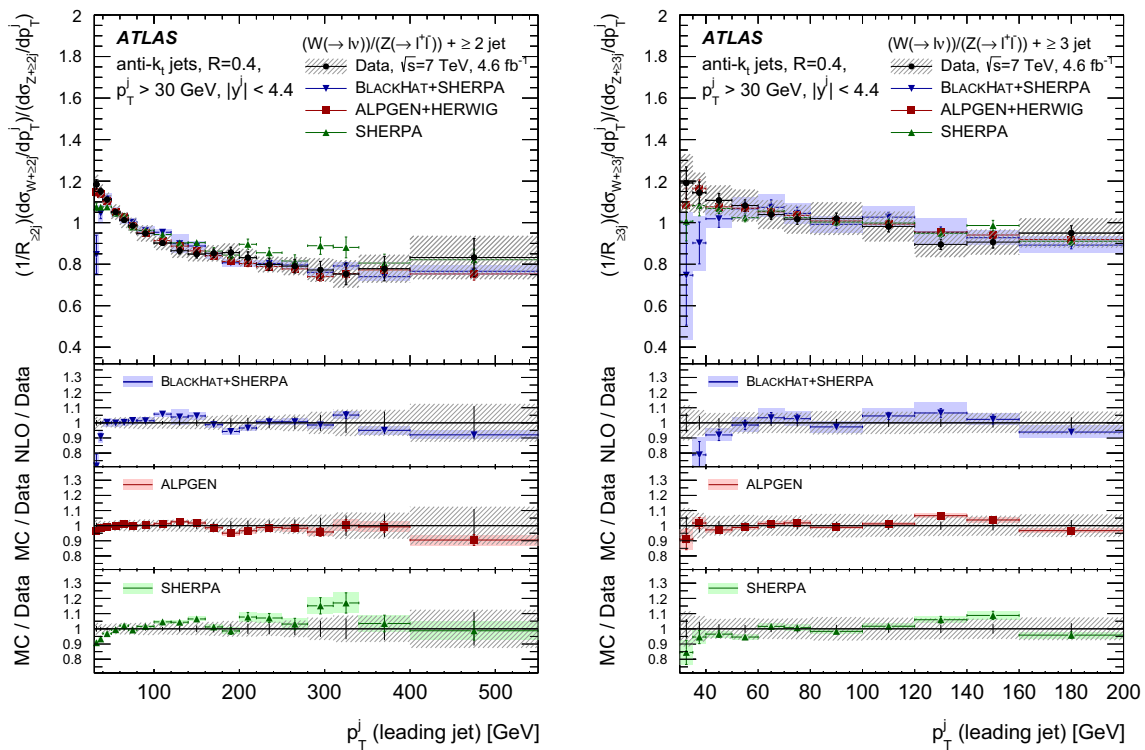
Fig. 3 The ratio of W + jets and Z + jets production cross sections, R_{\text{jets}} , normalized as described in the text versus the leading-jet transverse momentum, p_T^j , for N_{\text{jets}} \geq 2 (left) and \geq 3 (right). The electron and muon channel measurements are combined as described in the text. Ratios of the BLACKHAT+SHERPA NLO calculation and the ALPGEN and SHERPA generators to the data are shown in the lower
