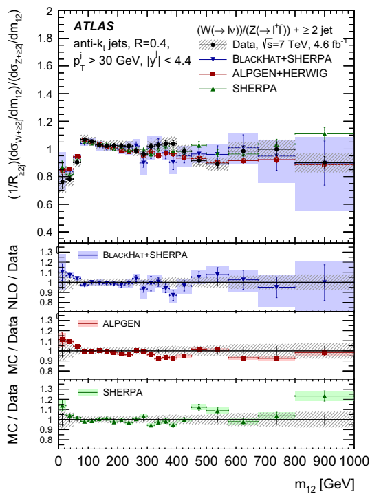
Fig. 8 The ratio of W + \text{jets} and Z + \text{jets} production cross sections, R_{\text{jets}} , normalized as described in the text versus the dijet invariant mass, m_{12} , for N_{\text{jets}} \geq 2 . The electron and muon channel measurements are combined as described in the text. Ratios of the BLACKHAT+SHERPA NLO calculation and the ALPGEN and SHERPA generators to the data are shown in the lower panels. Vertical error bars show the respective statistical uncertainties. The hatched error band shows statistical and systematic uncertainties added in quadrature for the data. The solid error bands show the statistical uncertainties for the ALPGEN and SHERPA predictions, and the combined statistical and theoretical uncertainties for the BLACKHAT+SHERPA prediction
