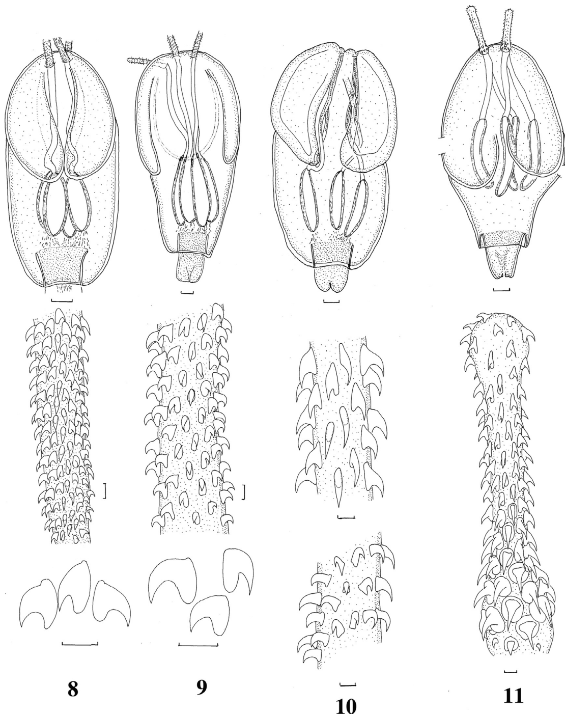
Figures 8–11. Tentacularioid metacestodes incompletely identified. 8. Nybelinia sp. A from Herklotsichthys quadrimaculatus (Rüppell, 1937). Scolex, basal and metabasal armature, hook profiles. Scale-bars: scolex and tentacle, 0.1 mm; hooks, 0.01 mm. 9. Nybelinia sp. B from Parupeneus multifasciatus (Quoy & Gaimard, 1825). Scolex, basal and metabasal armature, hook profiles. Scale-bars: scolex and tentacle, 0.1 mm; hooks, 0.01 mm. 10. Heteronybelinia sp. C from Sufflamen fraenatus (Latreille, 1804). Scolex, bothrial metabasal armature and antithrial metabasal armature. Scale-bars: scolex 0.1 mm; hooks 0.01 mm. 11. Nybelinia basimegacantha Carvajal, Campbell & Cornford, 1976, specimen from Neoniphon sammara (Forssskål, 1775). Scolex, basal and metabasal armature. Scale-bars: scolex 0.1 mm; tentacle 0.01 mm.
