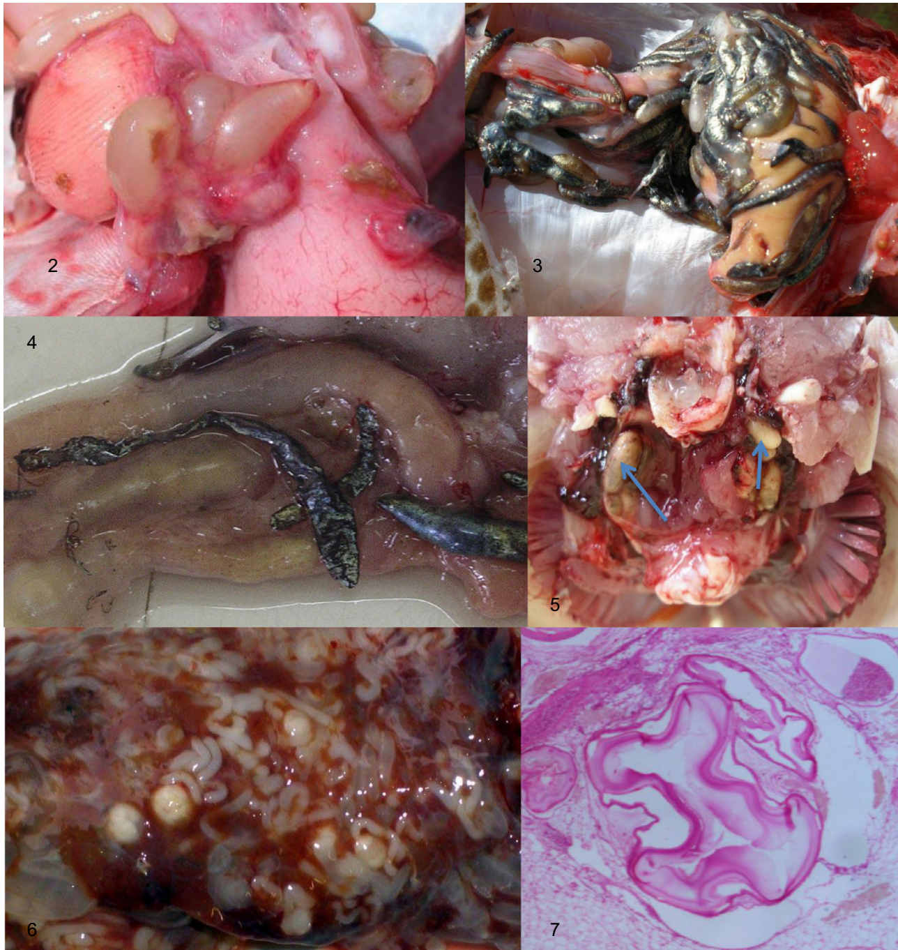
Figures 2–7. Metacestodes of trypanorhynch cestodes from teleost fishes. 2. Viable plerocerci of Callitetrarhynchus gracilis in the body cavity of Scomberomorus commerson . 3. Melanised trypanorhynch plerocerci in the body cavity of Epinephelus sp. 4. Melanised and contracted cysts of trypanorhynch metacestodes in the body cavity of Cephalopholis miniata ; no viable plerocerci were recovered from these cysts. 5. Plerocerci of Pseudogilquinia spp. (arrows) around the oesophagus of Lethrinus nebulosus . 6. Merocerci of Molicola horridus in the liver of Diodon hystrix . 7. Plerocerci of Grillotiella exile in the gill arches of Scomberomorus commerson (histological section).
