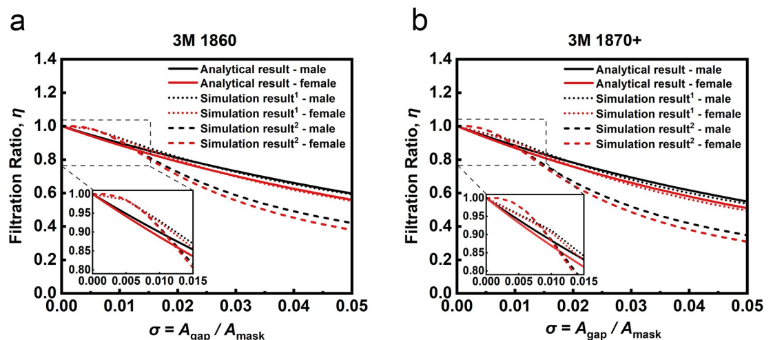
Fig 6. The dependences between \eta and \sigma for (a) 3M 1860 and (b) 1870+ masks. Dotted lines, 1, with W_{\text{mouth}} = W_{\text{mask}} + W_{\text{gap}} . Dashed lines, 2, showing the case a finite modelled mouth width W_{\text{mouth}} = 0.00463 m.
