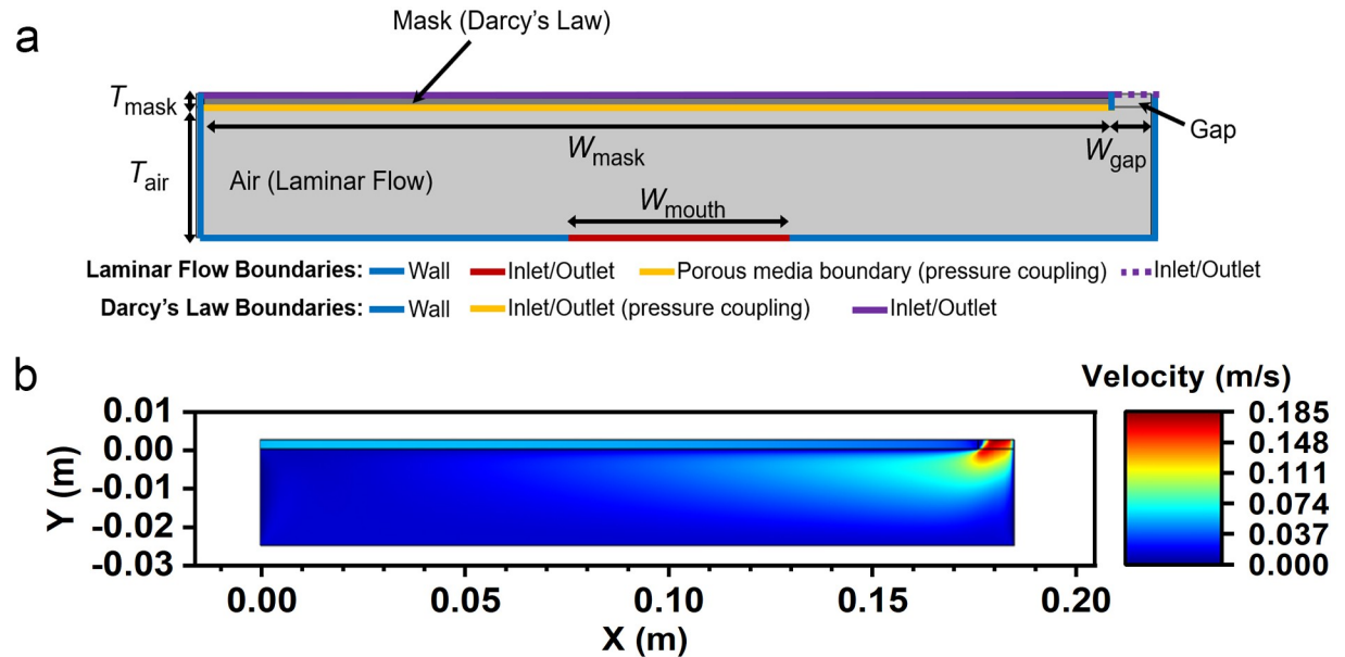
Fig 3. Schematic diagrams of the model. (a) Schematic diagram of FEM model and boundary conditions. Blue lines indicate solid walls, the red line indicates the inspiration/expiration location, the yellow line the inlet/outlet on the interior of the mask and the purple line the inlet/outlet on the mask exterior. (b) The velocity distribution during exhalation of a mask with \sigma = 0.05 and R = 900 \text{ Pa}\cdot\text{s}\cdot\text{m}^{-1} .
