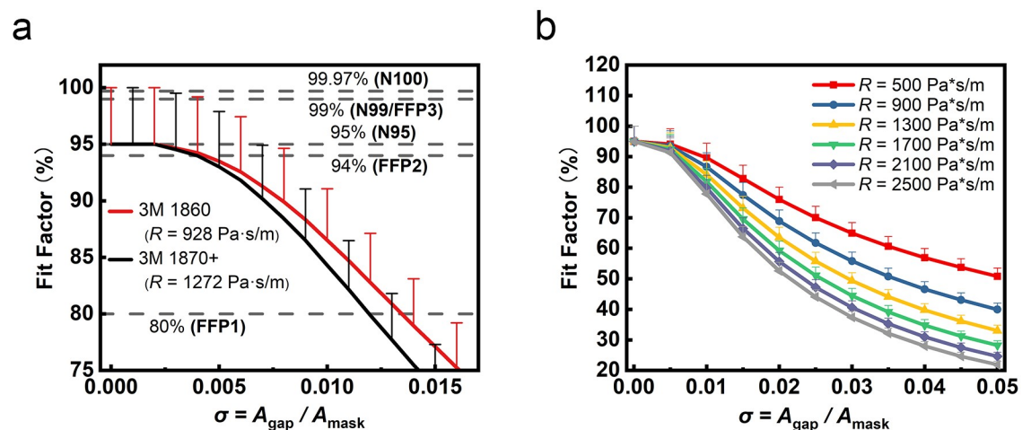
Fig 7. The results of gap area vs. fit factor. For (a) representative commercially available masks (3M 1860 and 1870+) and (b) N95 masks with various ventilation resistances.
