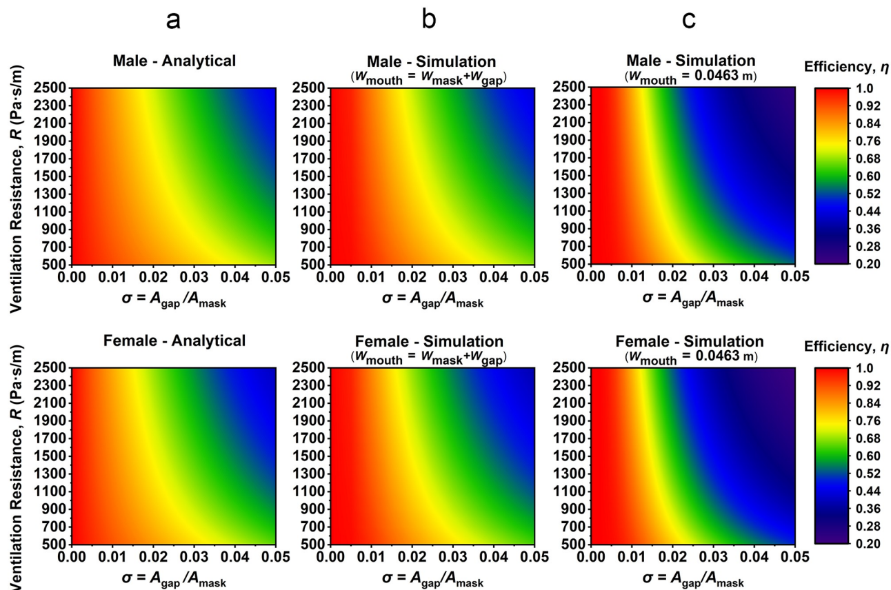
Fig 5. The relationships between \sigma , R , and \eta of different sex. (a) Analytical result, (b) simulation result with mouth inlet/outlet extending the width of the simulation domain ( W_{\text{mouth}} = W_{\text{mask}} + W_{\text{gap}} ), and (c) simulation result with a finite mouth width ( W_{\text{mouth}} = 0.0463 m).
