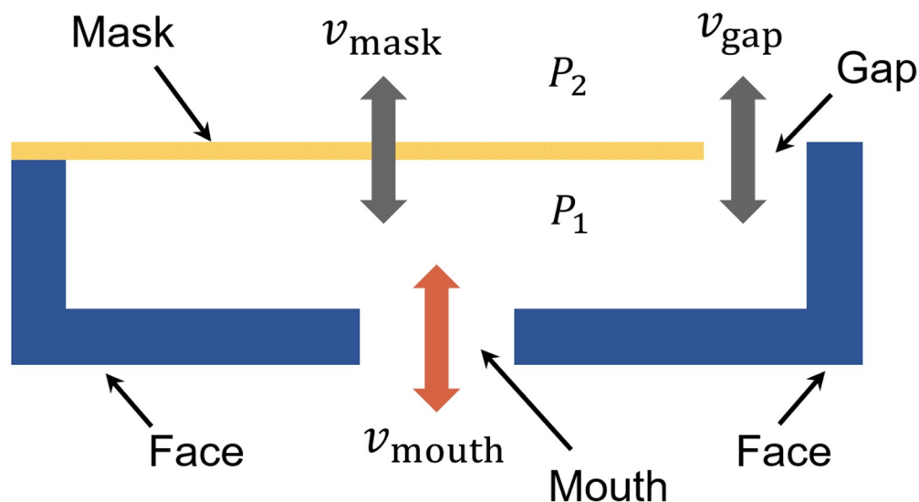
Fig 2. The model of the mask with face-seal leakage.
