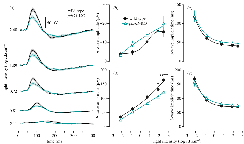
FIGURE 4. Scotopic ERGs of wild-type and pdzk1 -KO larvae. (a) Group average ERG traces. Wild-type and pdzk1 -KO larvae responses are shown as black and cyan lines, respectively, at -2.11, -0.81, 0.72, 1.89, and 2.48 log cd.s.m -2 . Scale bar: 50 \mu V. The light bands around group average traces represent \pm 1 SEM. Note that the a-wave is not visible in the group averages owing to variability in the implicit time, which causes the individual traces to cancel out. Remaining panels show group average ( \pm SEM) (b) a-wave amplitude, (c) a-wave implicit time, (d) b-wave amplitude, and (e) b-wave implicit time for wild-type (black circles) and pdzk1 -KO (cyan triangles) larvae. Lines were fit using a four-parameter sigmoidal function. Data were compared using two-way ANOVA with Bonferroni correction. * P < 0.05 ; **** P < 0.0001 .
