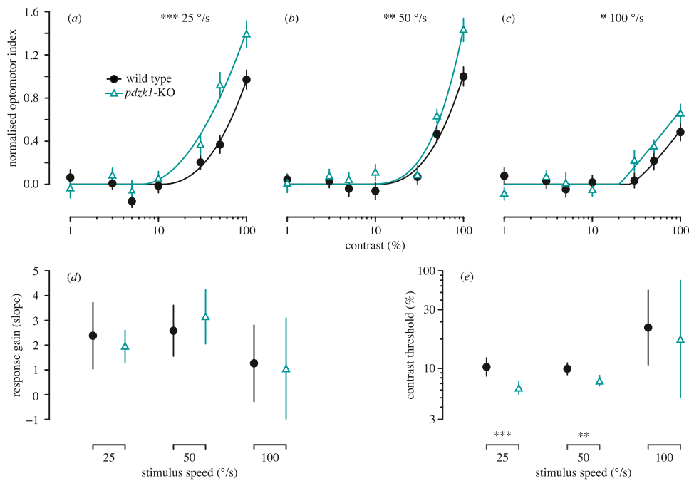
FIGURE 3. Contrast response functions measured using the OMR in wild-type (black circles and lines) and pdzk1 -KO larvae (cyan triangles and lines) at (a) 25°/s, (b) 50°/s, and (c) 100°/s. Contrast response curves are fit to the data using two-parameter piecewise functions by minimizing the least-squares error with respect to the data. Error bars show \pm SEM across trials. The bottom panels show (d) response gain and (e) contrast threshold as a function of group at the three stimulus speeds tested. Error bars show 95% confidence intervals on the fitted parameter. * P < 0.05 ; ** P < 0.01 ; *** P < 0.001 for the omnibus comparison of functions (upper panels) and for the comparison of individual parameters (lower panels) between genotypes.
