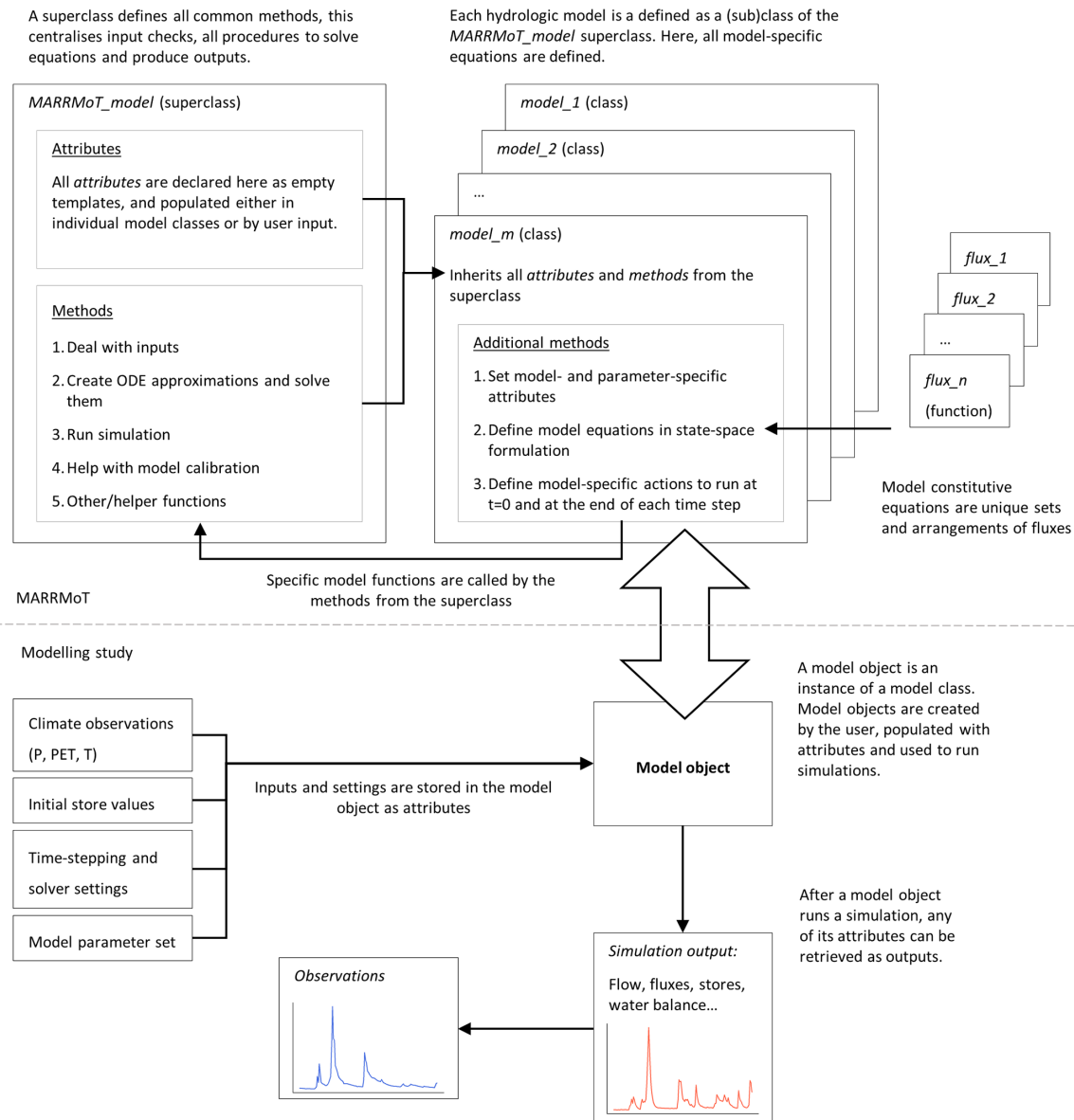
Figure 1. Schematic overview of the MARRMoT framework in its v2.1 implementation. A detailed description of the object-oriented MARRMoT implementation can be found in Sect. 2.1 and 2.2.
