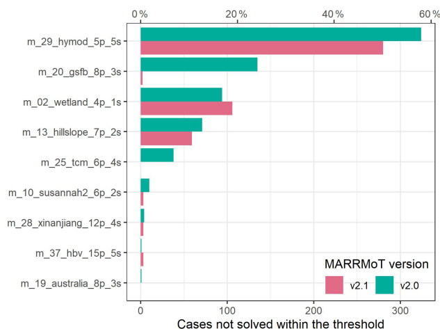
Figure 3. Number of cases (out of 559) where at least 1 time step is not solved within the convergence threshold for MARRMoT v2.0 and v2.1. All models not shown solved all time steps of all simulations for both versions of MARRMoT.
