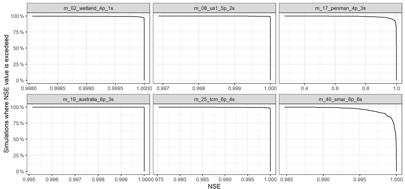
Figure 4. Exceedance curves of NSE values calculated between streamflow simulated with MARRMoT v2.0 and v2.1. All models not shown have \text{NSE} > 0.999 for all simulations. The exceedance curves indicate the percentage of simulations (out of 559) with NSE scores higher than the values on the x axis.
