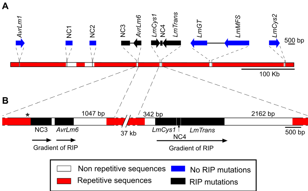
Figure 1. Location of the genes and non-coding, non-repetitive regions analysed from a 520 kb region of the Leptosphaeria maculans genome located on a 2.6 Mb chromosome in isolate v23.1.3. (A) Schematic representation of the AvrLm1-LmCys2 genomic region whereby highly-repetitive sequences with low GC content (red) flank single copy sections with high GC content (white). Four genes encoding small-secreted proteins, AvrLm1 , AvrLm6 , LmCys1 and LmCys2 , were sequenced from 295 Australian isolates, whilst the remaining three genes and four non-coding, non-repetitive regions (NC1-4) were sequenced in 84 of the 295 isolates. Repeat-induced point (RIP) mutations were detected in AvrLm6 , LmCys1 , LmTrans and two non-coding, non-repetitive regions (NC3 and NC4) (black). (B) Location of single-copy sequences relative to the flanking repetitive regions. Within each of the two single copy regions (black) analysed, the frequency of RIP alleles and distribution of RIP mutations decreased in a 5' to 3' gradient (arrows). The single copy region (149 bp) between NC3 and AvrLm6 was not analysed and so the gradient arrow is discontinuous. * denotes a repeat region (620 bp) directly upstream of NC3 that is highly RIP-affected. doi:10.1371/journal.ppat.1001180.g001
