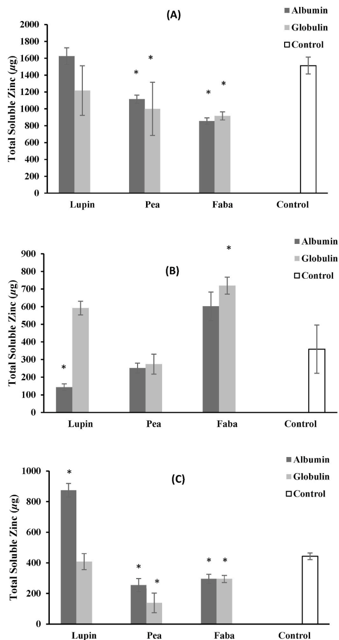
Fig. 3. Soluble zinc from mineral salt control and mineral fortified legume protein fractions subjected to a) oral-gastric (G), b) sequential oral-gastric-fasted intestinal (GI-Fasted), or c) sequential oral-gastric-fed intestinal (GI-Fed) stages of digestion. Values with an asterisk (*) are statistically significantly different from that of the mineral salt control in each column ( P < 0.05 ). Results are expressed as means \pm SEM ( n = 3 ).
