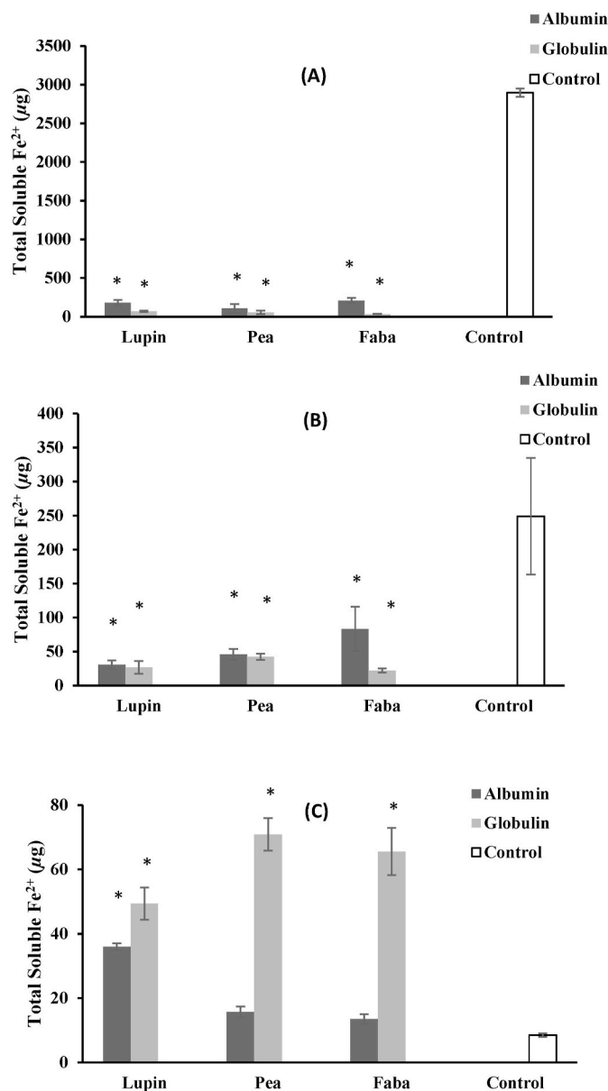
Fig. 2. Soluble Ferrous ( \text{Fe}^{2+} ) from mineral salt control and mineral fortified legume protein fractions subjected to a) oral-gastric (G), b) sequential oral-gastric-fasted intestinal (GI-Fasted), or c) sequential oral-gastric-fed intestinal (GI-Fed) stages of digestion. Values with an asterisk (*) are statistically significantly different from that of the mineral salt control in each column ( P < 0.05 ). Results are expressed as means \pm SEM ( n = 3 ).
