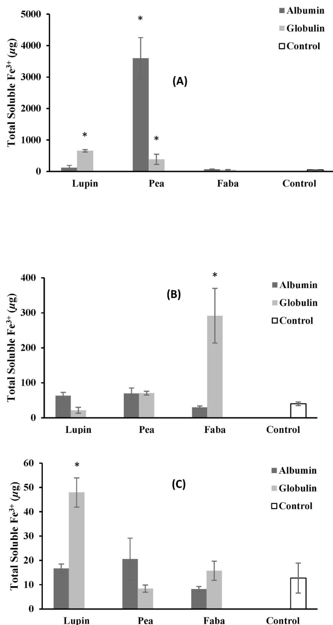
Fig. 1. Soluble Ferric ( \text{Fe}^{3+} ) from mineral salt control and mineral fortified legume protein fractions subjected to a) oral-gastric (G), b) sequential oral-gastric-fasted intestinal (GI-Fasted), or c) sequential oral-gastric-fed intestinal (GI-Fed) stages of digestion. Columns with an asterisk (*) are significantly different from that of the control mineral salt ( P < 0.05 ). Results are expressed as means \pm SEM ( n = 3 ).
