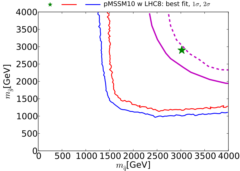
Figure 26. The (m_{\tilde{q}}, m_{\tilde{q}}) plane with our 68 and 95% CL contours shown as solid red and blue lines, respectively, and the best-fit point as a green star. Also shown as solid (dashed) magenta lines are the estimated ATLAS sensitivities for 5- \sigma discovery (95% CL exclusion) of SUSY via the generic \cancel{E}_T search with 300 \text{ fb}^{-1} at 14 TeV.
