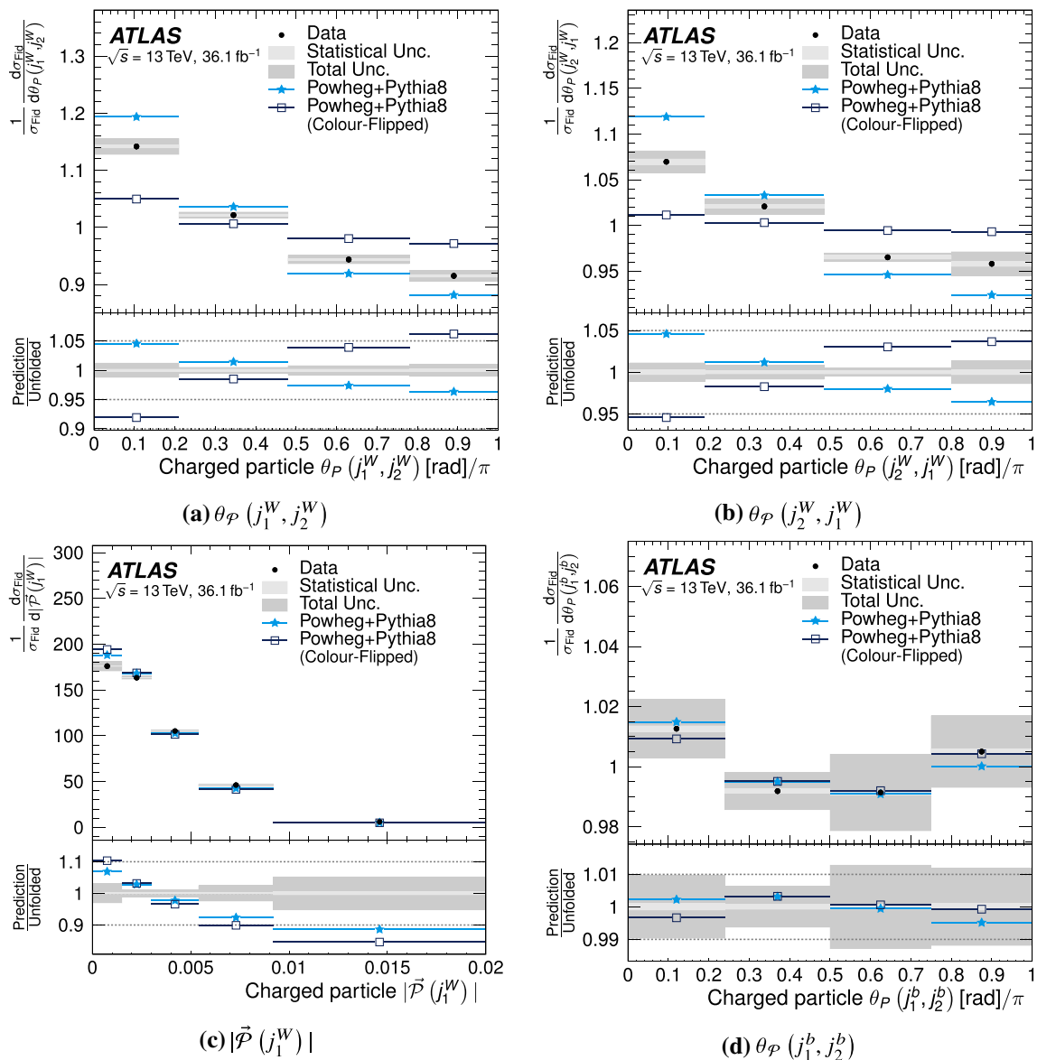
Fig. 6 Normalised fiducial differential cross-sections as a function of the a forward and b backward pull angle for the hadronically decaying W boson daughters, c the magnitude of the leading W daughter's jet-pull vector, and d the forward di- b -jet-pull angle. The data are compared to a SM prediction produced with POWHEG + PYTHIA 8 as well as the model with exotic colour flow also created with POWHEG + PYTHIA 8.
