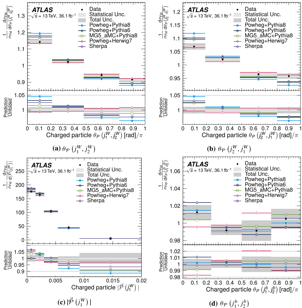
Fig. 5 Normalised fiducial differential cross-sections as a function of the a forward and b backward pull angle for the hadronically decaying W boson daughters, c the magnitude of the leading W daughter's jet-pull
