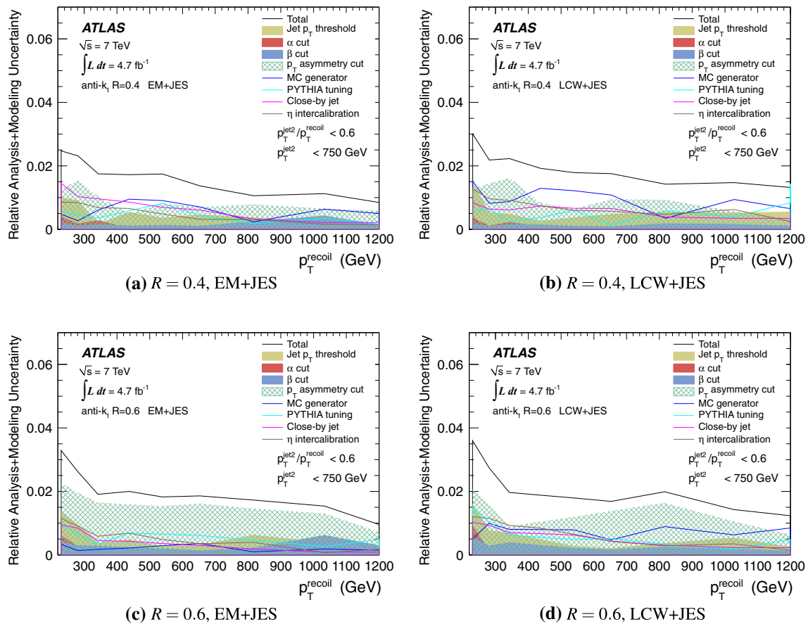
Fig. 32 Relative uncertainties on the MJB due to the systematic uncertainty sources considered in the analysis as a function of the recoil system p_T for anti- k_t jets with (a, b) R = 0.4 and (c, d) R = 0.6 , cali-
