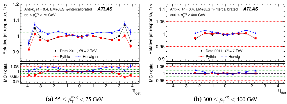
Fig. 34 Relative jet response, 1/c , as a function of the jet \eta_{\text{det}} for anti- k_t jets with R = 0.4 calibrated with the EM+JES scheme and in addition the derived \eta -intercalibration. Results are shown separately for a 55 \leq p_T^{\text{avg}} < 75 GeV and b 300 \leq p_T^{\text{avg}} < 400 GeV. For all points included in the original calibration ( |\eta_{\text{det}}| < 2.8 ), the data are corrected
