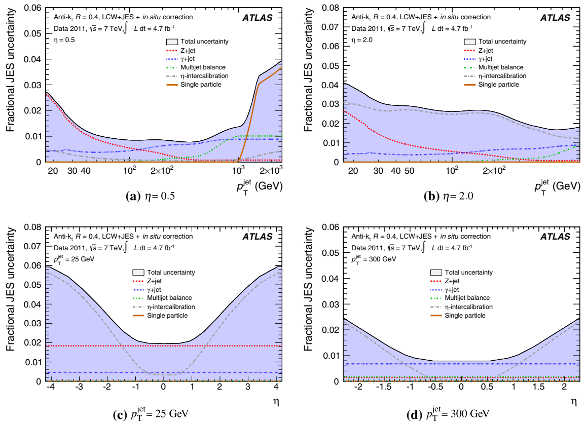
Fig. 60 Fractional in situ jet energy scale systematic uncertainty as a function of a, b p_T^{\text{jet}} and c, d jet pseudorapidity for anti- k_T jets with distance parameter of R = 0.4 calibrated using the LCW+JES cali-
