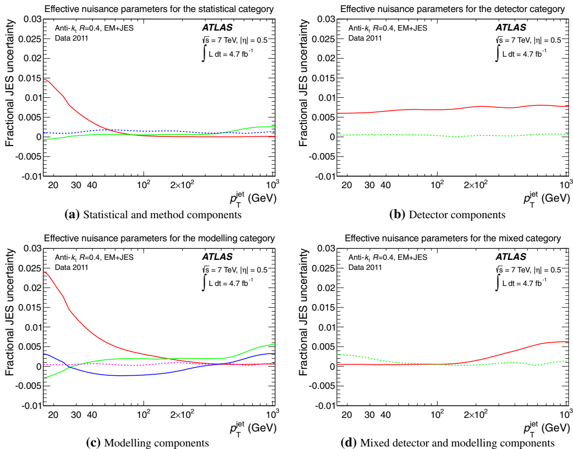
Fig. 42 Relative uncertainties for reduced (effective) components within a single category displayed as a fraction of jet p_T for anti- k_t jets with R = 0.4 , calibrated with the EM+JES scheme. The convention from Fig. 40 is followed here. The 54 nuisance parameters that are input to the reduction for each of the categories are listed in Table 10. The reduction is performed for all nuisance parameters belonging to any given category, which are statistical and method components ( a ), detec-
