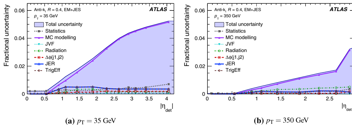
Fig. 13 Summary of uncertainties on the intercalibration as a function of the jet \eta_{\text{det}} for anti- k_t jets with R = 0.4 calibrated with the EM+JES scheme, separately for a p_T = 35 GeV and b p_T = 350 GeV.
