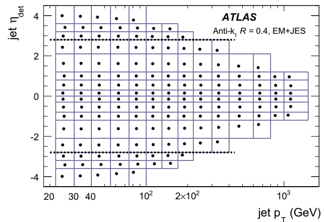
Fig. 9 Overview of the (p_T^{\text{avg}}, \eta_{\text{det}}) bins of the dijet balance measurements for jets reconstructed with distance parameter R = 0.4 calibrated using the EM+JES scheme. The solid lines indicate the (p_T^{\text{avg}}, \eta_{\text{det}}^{\text{probe}}) bin edges, and the points show the average transverse momentum and pseudorapidity of the probe jet within each bin. The measurements within the \eta_{\text{det}} range spanned by the two thick, dashed lines are used to derive the residual calibration
