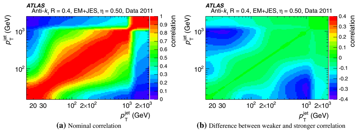
Fig. 41 In a , the nominal JES correlation matrix is shown. The difference between the correlation matrices of the interpretations resulting in stronger and weaker correlations for anti- k_t jets with R = 0.4 calibrated
