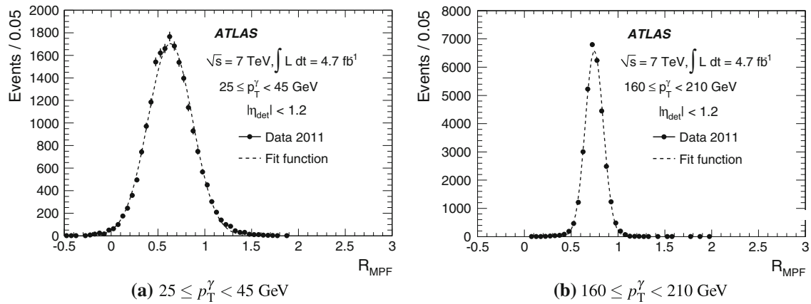
Fig. 21 MPF response distributions in the \gamma -jet data for a 25 \leq p_T^\gamma < 45 \text{ GeV} and b 160 \leq p_T^\gamma < 210 \text{ GeV} when using topo-clusters at the EM scale. The dashed lines represent the fits with a Gaussian function.
