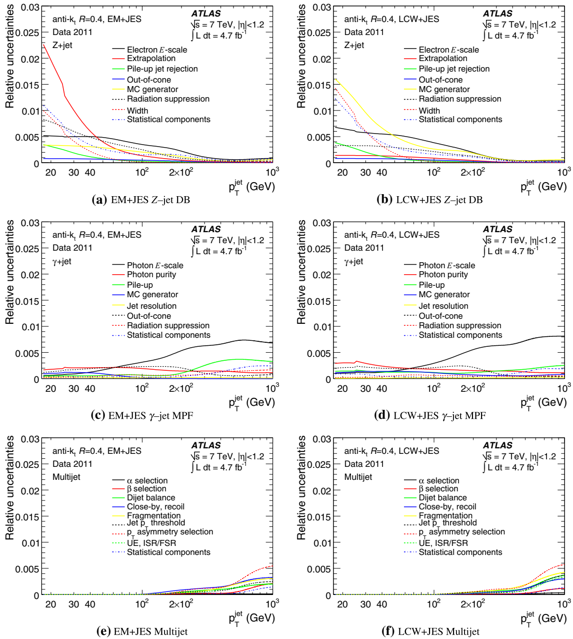
Fig. 37 Individual uncertainty sources applicable to the combined response ratio as a function of the jet p_T for the three in situ techniques: a, b Z-jet direct balance, c, d \gamma -jet MPF and e, f multijet balance for
