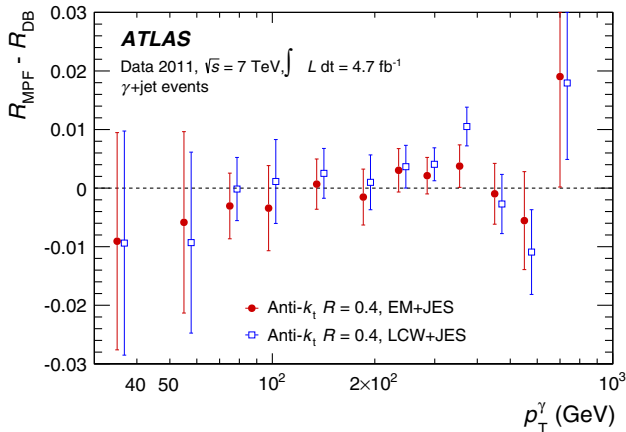
Fig. 39 Difference between the data-to-MC response ratio R measured using the direct balance (DB) and the missing momentum fraction (MPF) methods for jets reconstructed with the anti- k_t algorithm with R = 0.4 calibrated with the EM+JES and LCW+JES schemes. The error bars shown only contain the uncorrelated uncertainties
