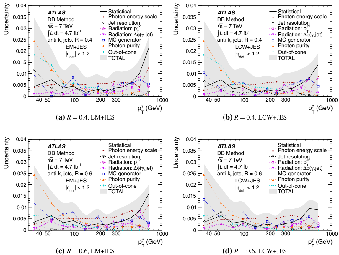
Fig. 28 Systematic uncertainties on the data-to-MC ratio of the jet response, as determined by the DB technique in \gamma -jet events, for anti- k_t jets with (a, b) R = 0.4 and (c, d) R = 0.6 , calibrated with the (a, c)
