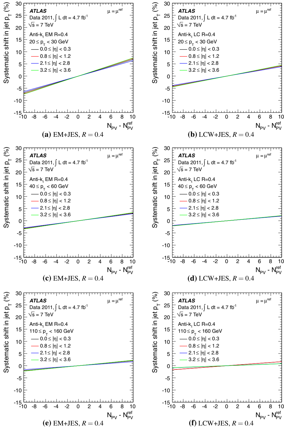
Fig. 46 The fractional systematic shift due to mis-modelling of the effect of in-time pile-up on the transverse momentum p_{T,EM+JES}^{\text{jet}} of jets reconstructed with the anti- k_t algorithm with R = 0.4 , and calibrated with the EM+JES scheme, is shown as a function of (N_{PV} - N_{PV}^{\text{ref}}) in a ,
