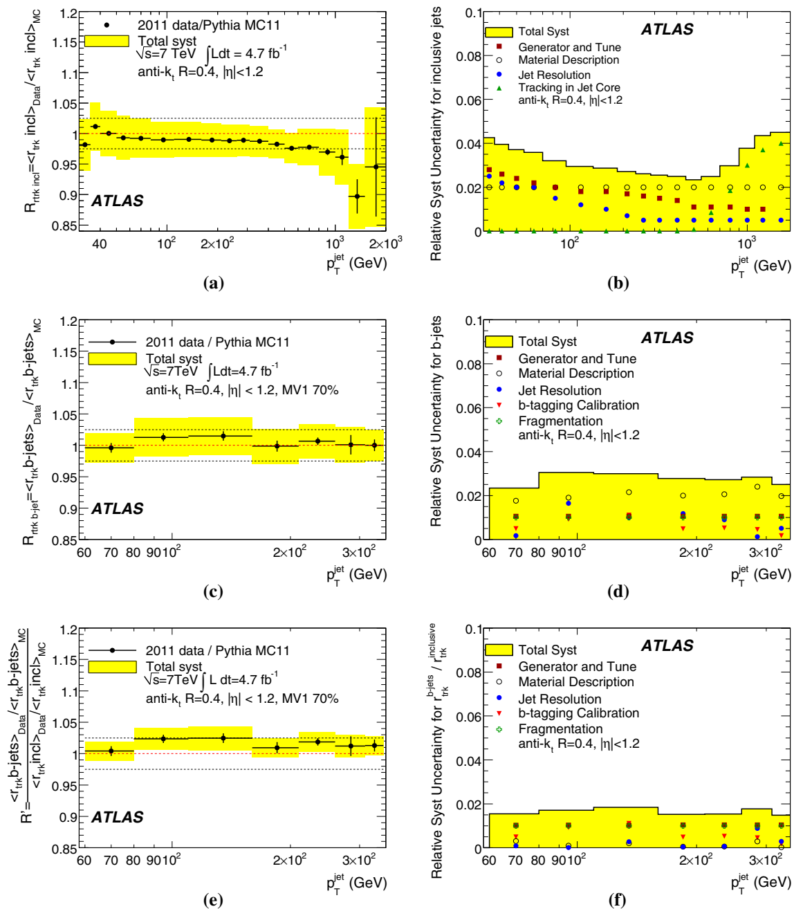
Fig. 54 Ratio of the average r_{\text{trk}} given in Eq. (19) in data and MC simulations for a inclusive jets and c tagged b -jets. In e , the b -tagged to inclusive sample ratio variable R' from Eq. (21) is shown. The con-
