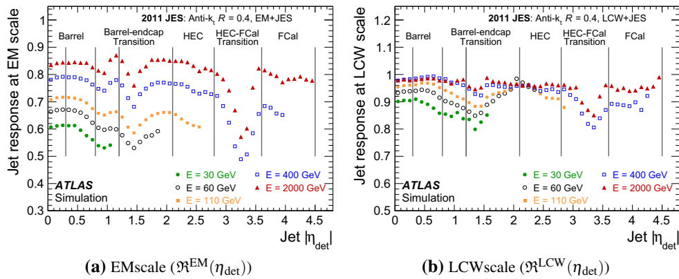
Fig. 4 Average response of simulated jets formed from topo-clusters, calculated as defined in Eq. (1) and shown in a for the EM scale ( \mathcal{R}^{\text{EM}} ) and in b for the LCW scale ( \mathcal{R}^{\text{LCW}} ). The response is shown separately for various truth-jet energies as function of the uncorrected (detector) jet
