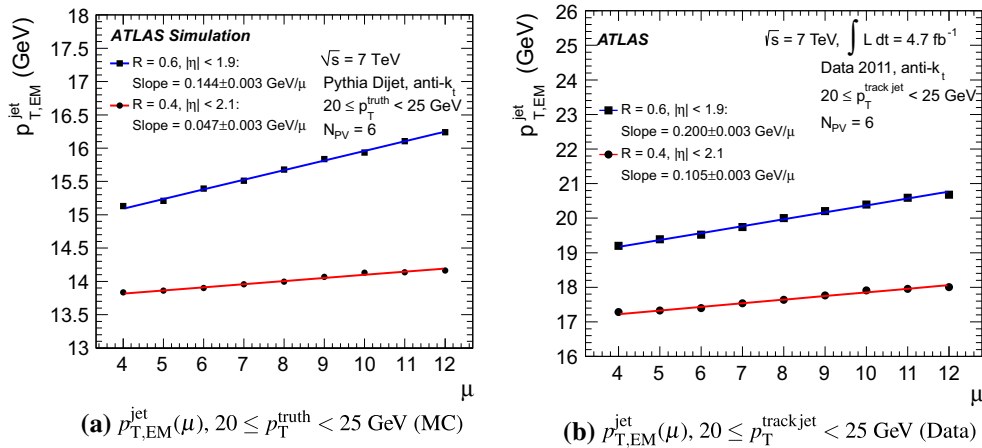
Fig. 7 The average reconstructed jet transverse momentum p_{T,EM}^{jet} on EM scale as function of the average number of collisions \mu at a fixed number of primary vertices N_{PV} = 6 , for truth jets in MC simulation a
