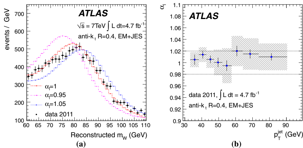
Fig. 44 The three templates distributions for the reconstructed W mass in t\bar{t} events obtained by shifting the jet energy by a factor \alpha_l = 0.95, 1 and 1.05 in the Monte Carlo simulation with respect to the one in data (a). The Monte Carlo simulation templates are also compared to the data
