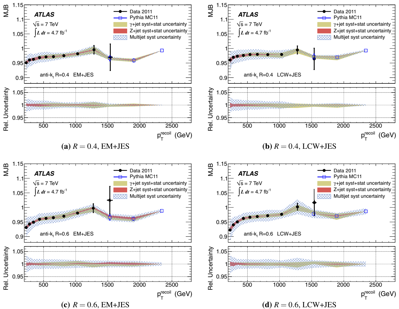
Fig. 33 Multijet balance and systematic uncertainties related to the multijet balance technique and to the propagated uncertainties from the \gamma -jet and Z-jet balance as a function of the recoil system p_T^{\text{recoil}} for anti- k_t jets with (a, b) R = 0.4 and (c, d) R = 0.6 , calibrated with the (a, c) EM+JES scheme and with the (b, d) LCW+JES scheme. The subleading jets in the data are corrected by the combination of \gamma -jet and Z-jet in situ calibrations at p_T < 750 GeV and MJB calibration at
