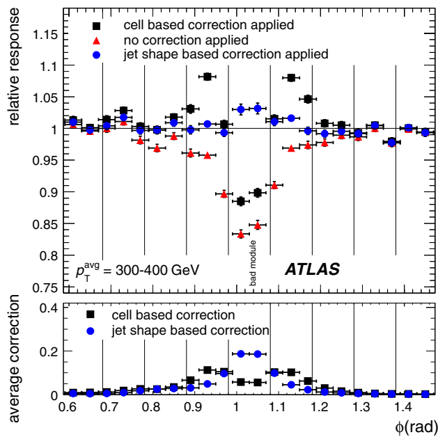
Fig. 58 Average relative response of the probe jets with respect to the tag jets as a function of various impact points in the azimuthal direction ( \phi ) of the probe jet. The average p_T of the two leading jets is 300 \leq p_T^{\text{avg}} < 400 GeV. The vertical solid lines indicate the location of the Tile calorimeter modules. The non-operating Tile calorimeter module is at \phi = 1.03 . The markers indicate the results for no correction (triangles), the cell-based corrections (squares) and the corrections based on the jet shape (circles). The lower part of the figure shows the respective average values of the two corrections as a function of the azimuthal angle of the probe jet
