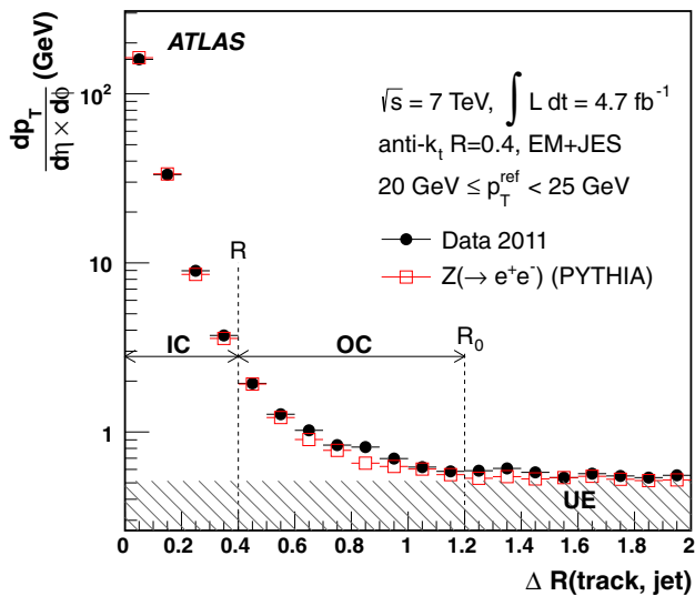
Fig. 18 Transverse momentum profile of tracks around the leading jet axis for events with 20 \leq p_T^{\text{ref}} < 25 GeV in Z-jet events. The radii R and R_0 are those used in Eq. (12) to define the IC and IC+OC regions. The hatched area indicates the contribution from the underlying event (UE). Anti- k_t jets with R = 0.4 calibrated with the EM+JES scheme are considered
