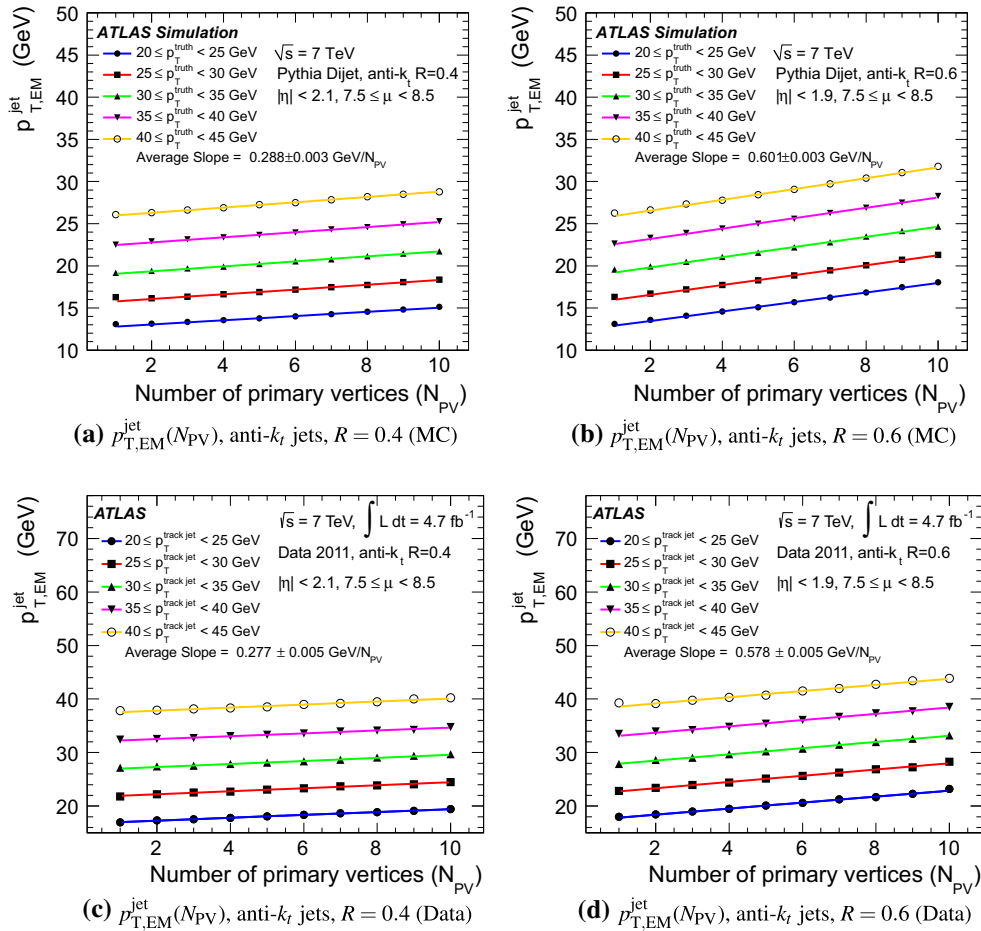
Fig. 6 The average reconstructed transverse momentum p_{T,EM}^{\text{jet}} on EM scale for jets in MC simulations, as function of the number of reconstructed primary vertices N_{PV} and 7.5 \leq \mu < 8.5 , in various bins of truth-jet transverse momentum p_T^{\text{truth}} , for jets with a R = 0.4 and b
