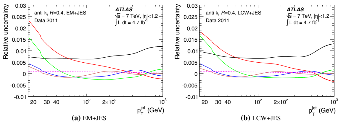
Fig. 40 Systematic (effective) relative uncertainties displayed as a function of jet p_T for anti- k_t jets with R = 0.4 calibrated with the a EM+JES and the b LCW+JES calibration schemes for the reduced scheme with six nuisance parameters. Each curve can be interpreted as
