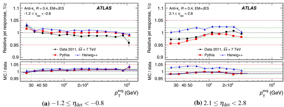
Fig. 12 Relative jet response ( 1/c ) as a function of the average jet p_T of the dijet system for anti- k_t jets with R = 0.4 calibrated with the EM+JES scheme, separately for a -1.2 \leq \eta_{\text{det}} < -0.8 and b
