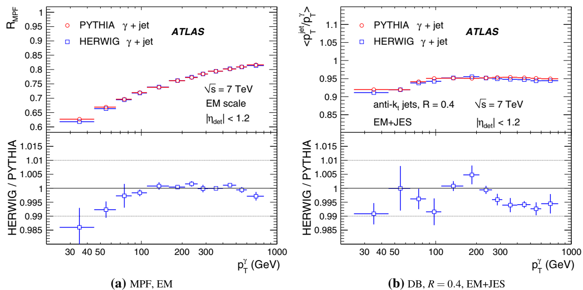
Fig. 25 Average jet response as determined by the a MPF and b DB techniques, using anti- k_t jets with R = 0.4 at the EM and EM+JES energy scales respectively, for PYTHIA (circles) and HERWIG (squares)
