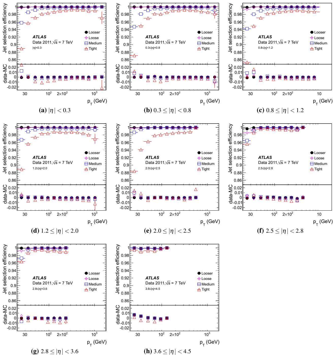
Fig. 5 Jet quality selection efficiency for anti- k_t jets with R = 0.4 measured with a tag-and-probe technique as a function of p_T^{\text{jet}} in various \eta ranges, for the four sets of selection criteria. Only statistical uncertainties are shown. Differences between data and MC simulations are also shown
