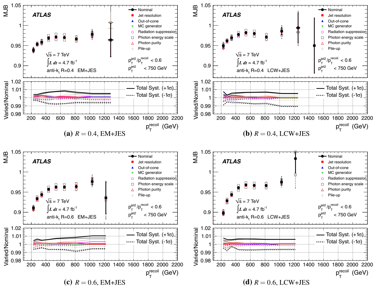
Fig. 31 Multijet balance with the nominal and varied \gamma -jet in situ calibrations as a function of the recoil system p_T^{\text{recoil}} for anti- k_T jets with (a, b) R = 0.4 and (c, d) R = 0.6 , calibrated with the (a, c) EM+JES scheme and with the (b, d) LCW+JES scheme. The varied distributions are obtained by fluctuating the jet energy scale for the non-leading jets by \pm 1\sigma for each of the systematic uncertainties and repeating the analy-
