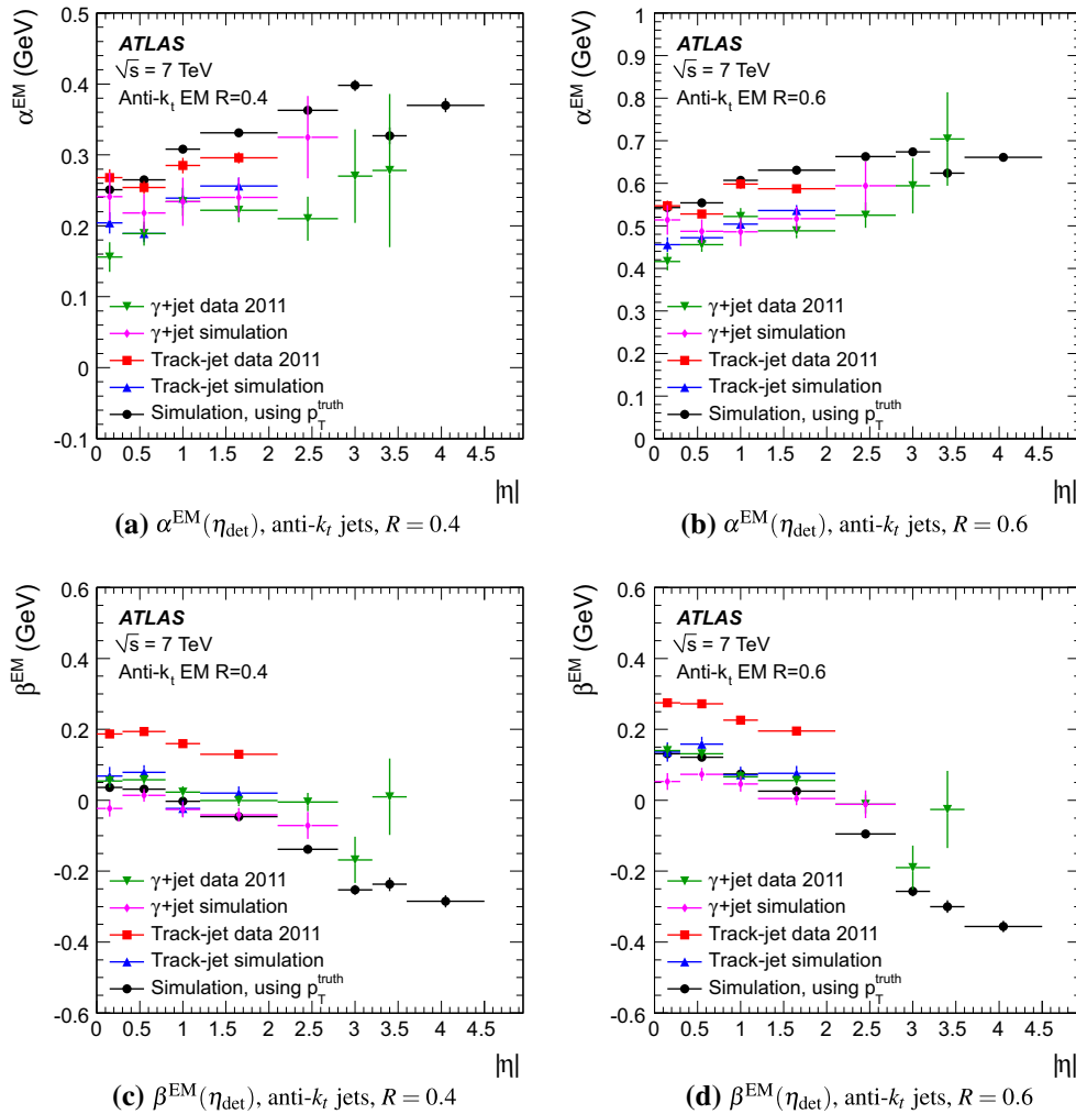
Fig. 8 The pile-up contribution per additional vertex, measured as \alpha^{\text{EM}} = \partial p_{\text{T,EM}}^{\text{jet}} / \partial N_{\text{PV}} , as function of |\eta_{\text{det}}| , for the various methods discussed in the text, for a R = 0.4 and b R = 0.6 jets. The contribution from \mu , calculated as \beta^{\text{EM}} = \partial p_{\text{T,EM}}^{\text{jet}} / \partial \mu and displayed for the various
