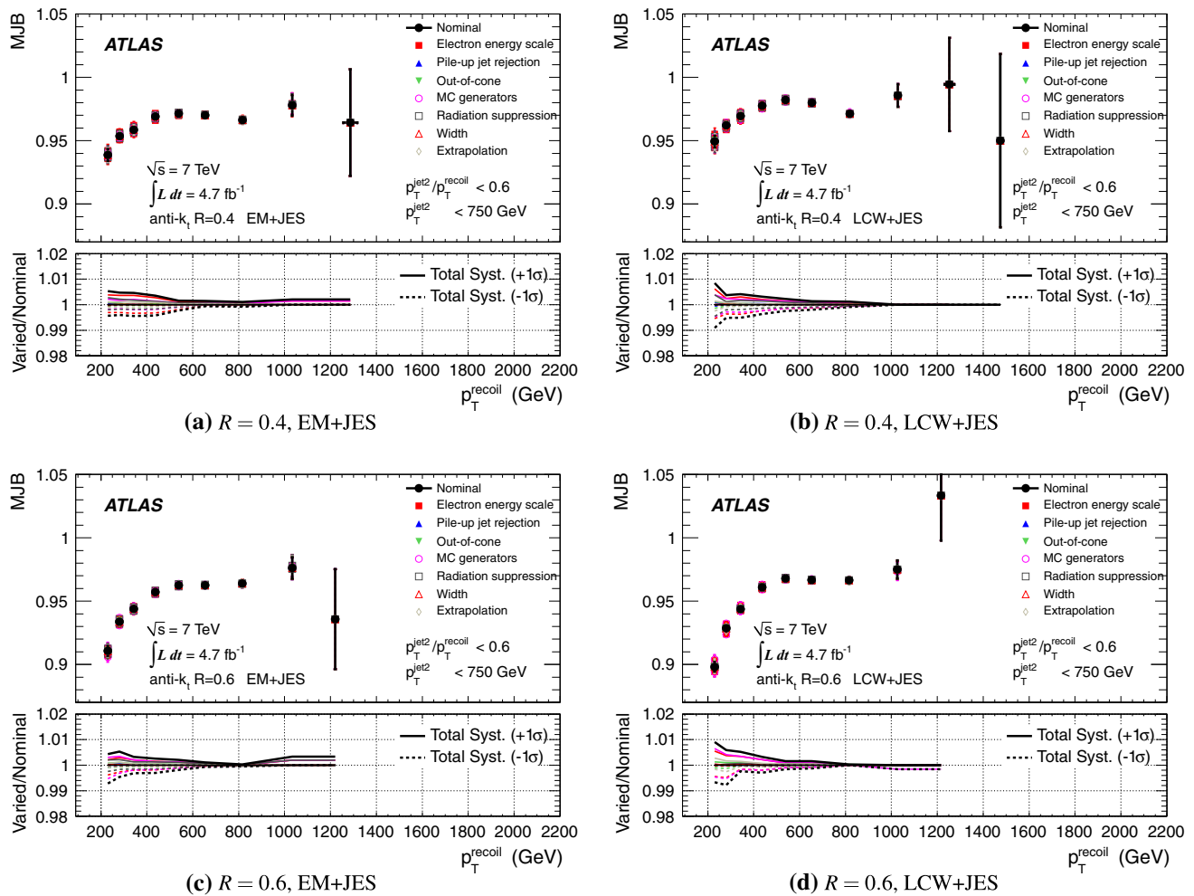
Fig. 30 Multijet balance with the nominal and varied Z-jet in situ calibrations as a function of the recoil system p_T^{\text{recoil}} for anti- k_t jets with (a, b) R = 0.4 and (c, d) R = 0.6 , calibrated with the (a, c) EM+JES scheme and with the (b, d) LCW+JES scheme. The varied distributions are obtained by fluctuating the jet energy scale for the non-leading jets by \pm 1\sigma for each of the systematic uncertainties for the Z-jet calibra-
