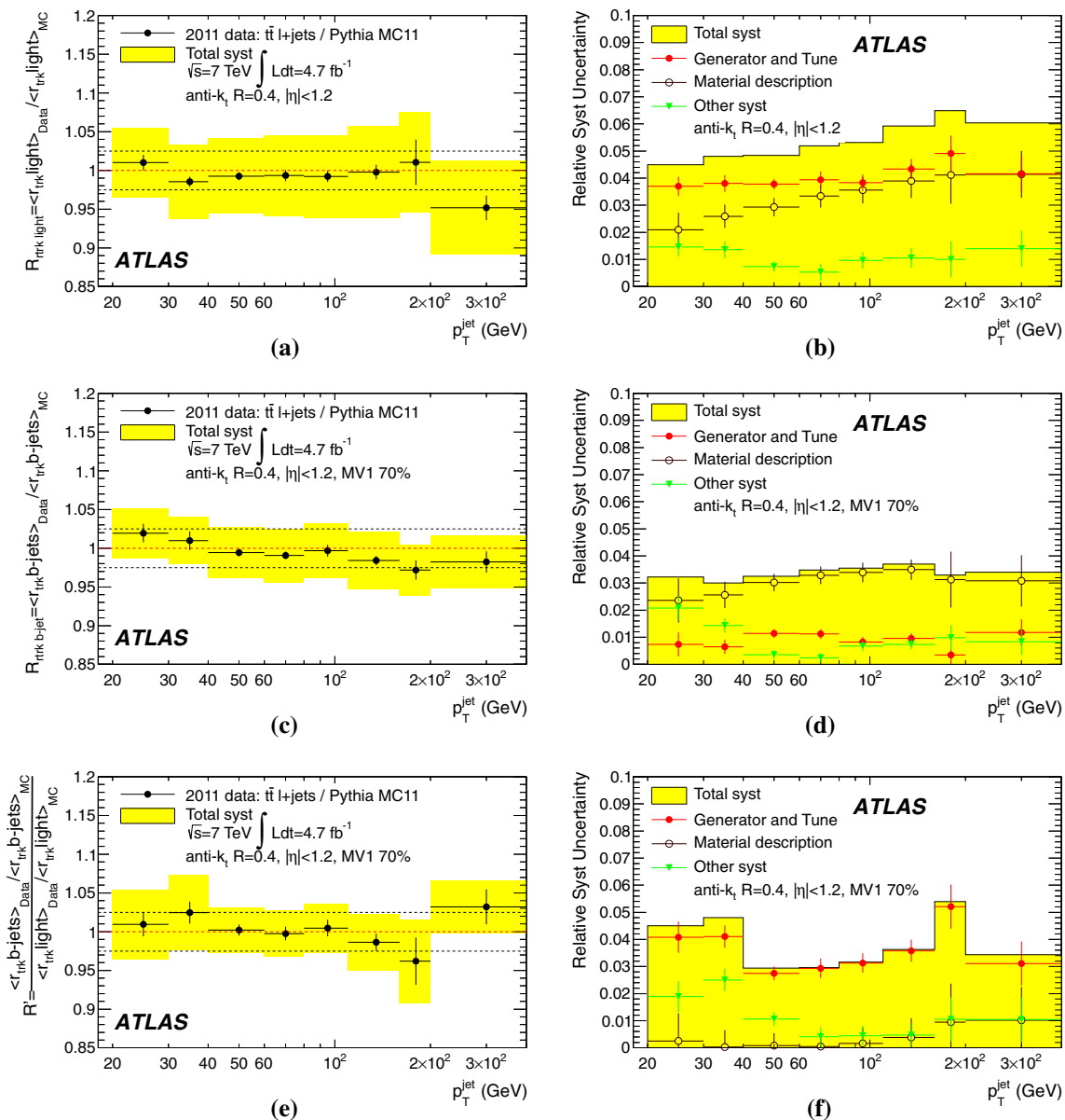
Fig. 55 Ratio of the average r_{\text{trk}} given in Eq. (19) in t\bar{t} events in data and MC simulations for a light-jets and tagged c b -jets. In e , the ratio of R_{r_{\text{trk}}} from Eq. (20) between the b -jet and the light-jet sample is shown. The total systematic uncertainty is shown as a band, and the dotted lines correspond to unity and the 2.5 % deviation from unity. The contributions of the systematic uncertainties to the total uncertainty in the
