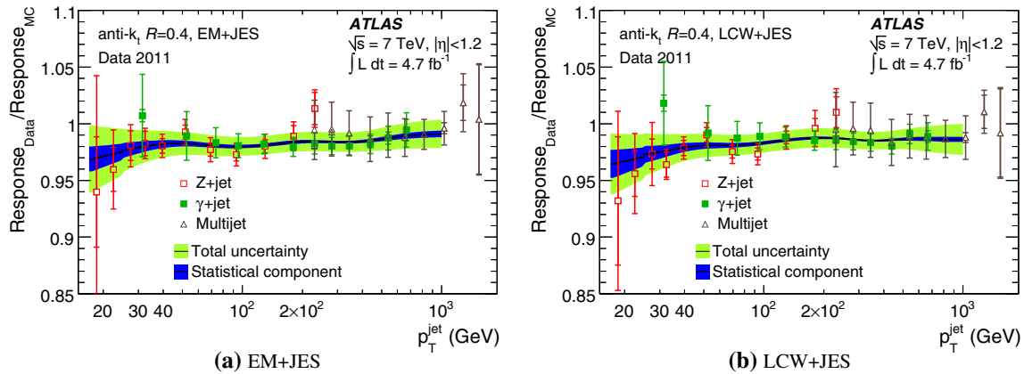
Fig. 38 Ratio of the average jet response \langle p_T^{\text{jet}} / p_T^{\text{ref}} \rangle measured in data to that measured in MC simulations for jets within |\eta| < 1.2 as a function of the transverse jet momentum p_T^{\text{jet}} . The data-to-MC jet response ratios are shown separately for the three in situ techniques used in the combined calibration: direct balance in Z-jet events, MPF in \gamma -jet events, and multijet p_T balance in inclusive jet events. The error bars
