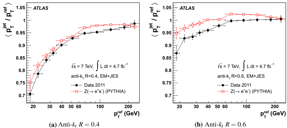
Fig. 17 Mean p_T balance obtained in the data and with the PYTHIA simulation. Results for anti- k_t jets with distance parameter a R = 0.4 and b R = 0.6 calibrated with the EM+JES scheme are shown. Only statistical uncertainties are shown
