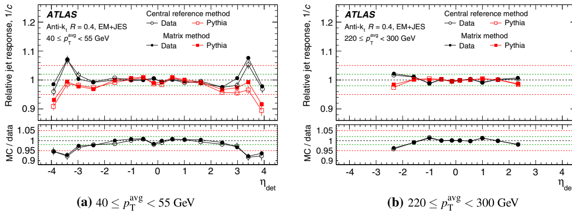
Fig. 10 Relative jet response ( 1/c ) for anti- k_t jets with R = 0.4 calibrated with the EM+JES scheme as a function of the probe jet pseudorapidity measured using the matrix and the central reference methods.
