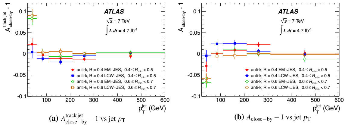
Fig. 50 In a , the deviation from unity of the data-to-MC ratio of the track-jet p_T for non-isolated jets divided by the track-jet p_T for isolated jets, is shown as a function of the jet p_T . The deviation from unity of the data-to-MC ratio of the relative response of non-isolated jets with
