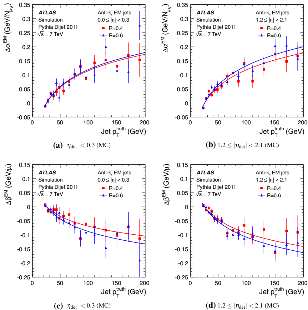
Fig. 45 The difference from the average \alpha^{\text{EM}}(\eta_{\text{det}}) of the in-time pile-up signal contribution per reconstructed primary vertex ( \Delta(\partial p_{\text{T,EM}}^{\text{jet}}/\partial N_{\text{PV}})(p_{\text{T}}^{\text{truth}}) ) as a function of the true jet transverse momentum p_{\text{T}}^{\text{truth}} , for MC-simulated jets reconstructed with anti- k_t R = 0.4 and R = 0.6 at the EM scale, in two different regions a |\eta_{\text{det}}| < 0.3 and b 1.2 \leq |\eta_{\text{det}}| < 2.1 of the ATLAS calorimeter. In c and
