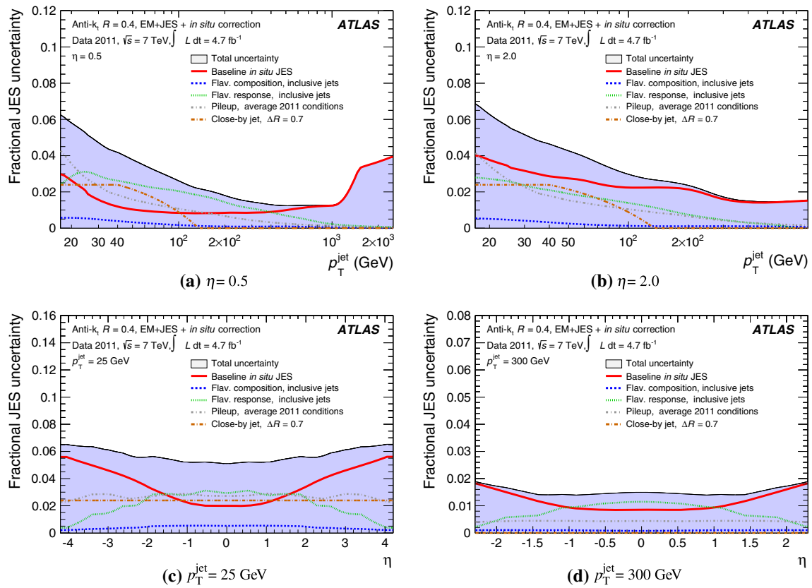
Fig. 63 Sample-dependent fractional jet energy scale systematic uncertainty as a function of a, b p_T^{\text{jet}} and c, d jet pseudorapidity for anti- k_T jets with distance parameter of R = 0.4 calibrated using the
