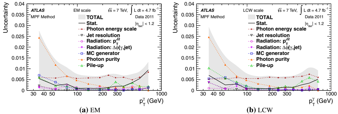
Fig. 27 Systematic uncertainties on the data-to-MC ratio of the jet response, as determined by the MPF technique for \gamma -jet events using topo-clusters at the a EM and b LCW energy scales, as a function of the photon transverse momentum
