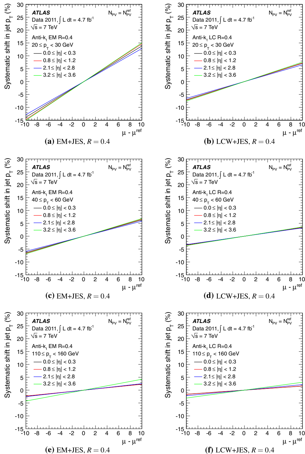
Fig. 48 The fractional systematic shift due to mis-modelling of the effect of out-of-time pile-up on the transverse momentum p_{T,EM+JES}^{\text{jet}} of jets reconstructed with the anti- k_t algorithm with R = 0.4 and calibrated with the EM+JES scheme, is shown as a function of (\mu - \mu^{\text{ref}})
