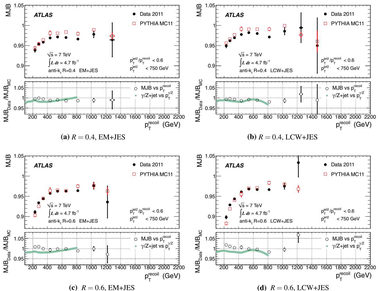
Fig. 29 Multijet balance as a function of the recoil system p_T^{\text{recoil}} for anti- k_t jets with (a, b) R = 0.4 and (c, d) R = 0.6 , calibrated with the (a, c) EM+JES scheme and with the (b, d) LCW+JES scheme, for both data and MC simulations. The non-leading jets in the data with p_T < 750 GeV are corrected by the combination of \gamma -jet and Z-jet in situ calibrations as described in Sect. 11.1. The open points in the
