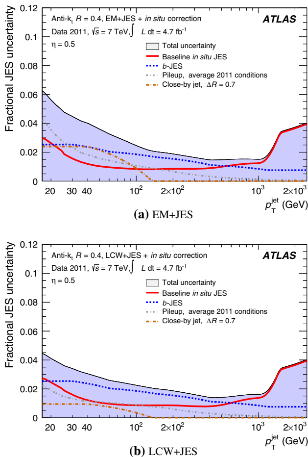
Fig. 65 Fractional jet energy scale systematic uncertainty as a function of p_T^{\text{jet}} for anti- k_t jets with distance parameter of R = 0.4 calibrated using the a EM+JES and b LCW+JES calibration schemes. The uncertainty shown applies to b -jets with average 2011 pile-up conditions
