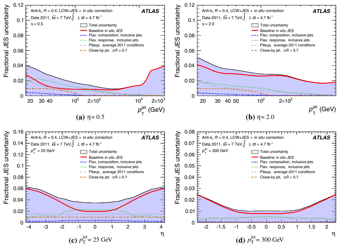
Fig. 64 Sample-dependent fractional jet energy scale systematic uncertainty as a function of a, b p_T^{\text{jet}} and c, d jet pseudorapidity for anti- k_t jets with distance parameter of R = 0.4 calibrated using the
