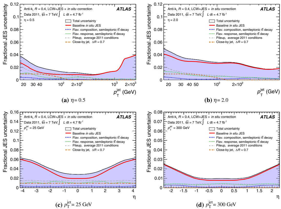
Fig. 62 Sample-dependent fractional jet energy scale systematic uncertainty as a function of a , b p_T^{\text{jet}} and c , d jet pseudorapidity for anti- k_t jets with distance parameter of R = 0.4 calibrated using
