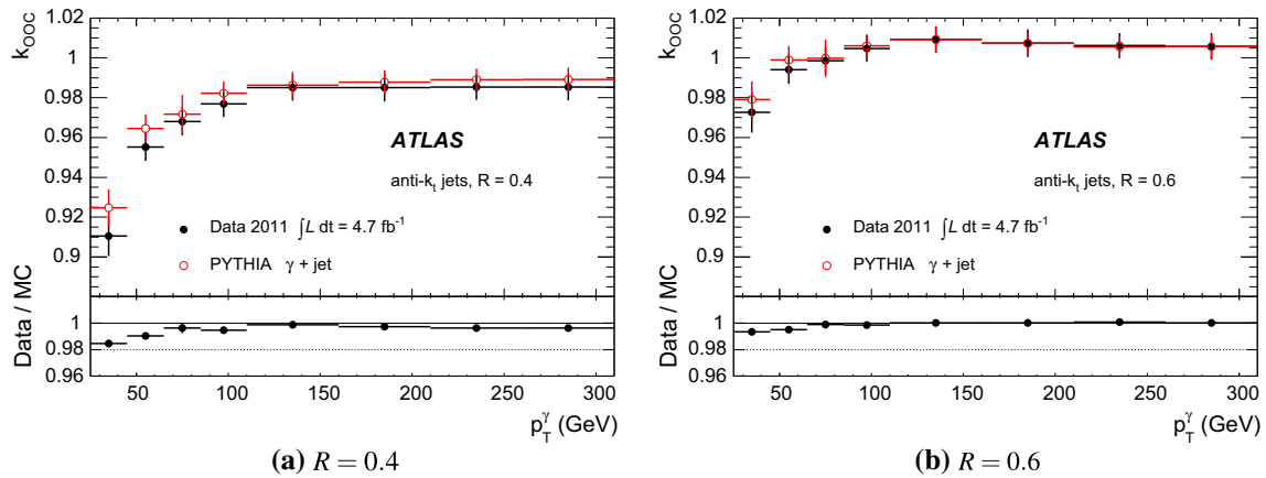
Fig. 26 Out-of-cone radiation factor k_{\text{OOC}} relating the p_T of the photon with the p_T of the truth jet as a function of the photon transverse momentum, measured using charged particles, for anti- k_t jets with a
