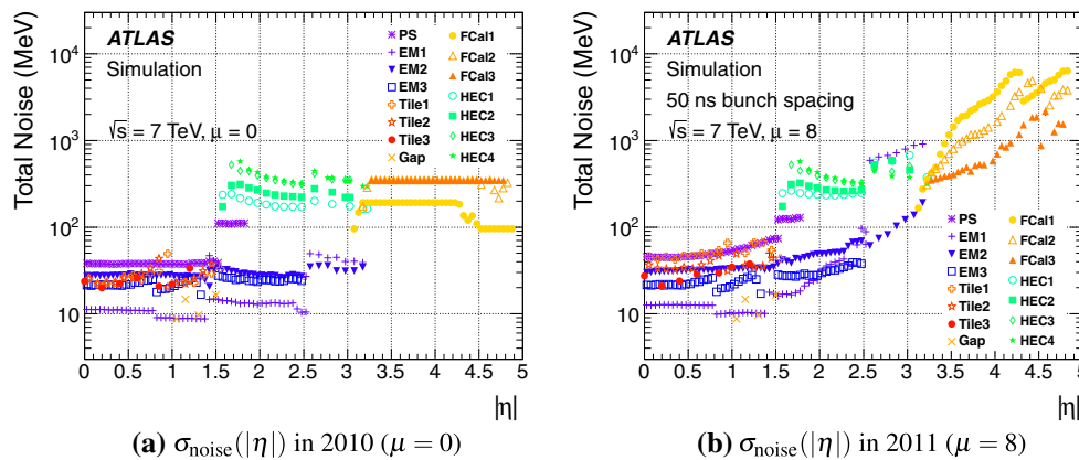
Fig. 1 The energy-equivalent cell noise in the ATLAS calorimeters on the electromagnetic (EM) scale as a function of the direction |\eta| in the detector, for the 2010 configuration with a \mu = 0 and the 2011 configuration with b \mu = 8 . The various colours indicate the noise in the
