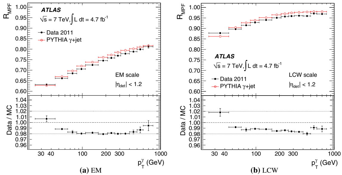
Fig. 23 Average jet response as determined by the MPF technique in \gamma -jet events using topo-clusters at the a EM and b LCW energy scales, for both data and MC simulations, as a function of the photon transverse
