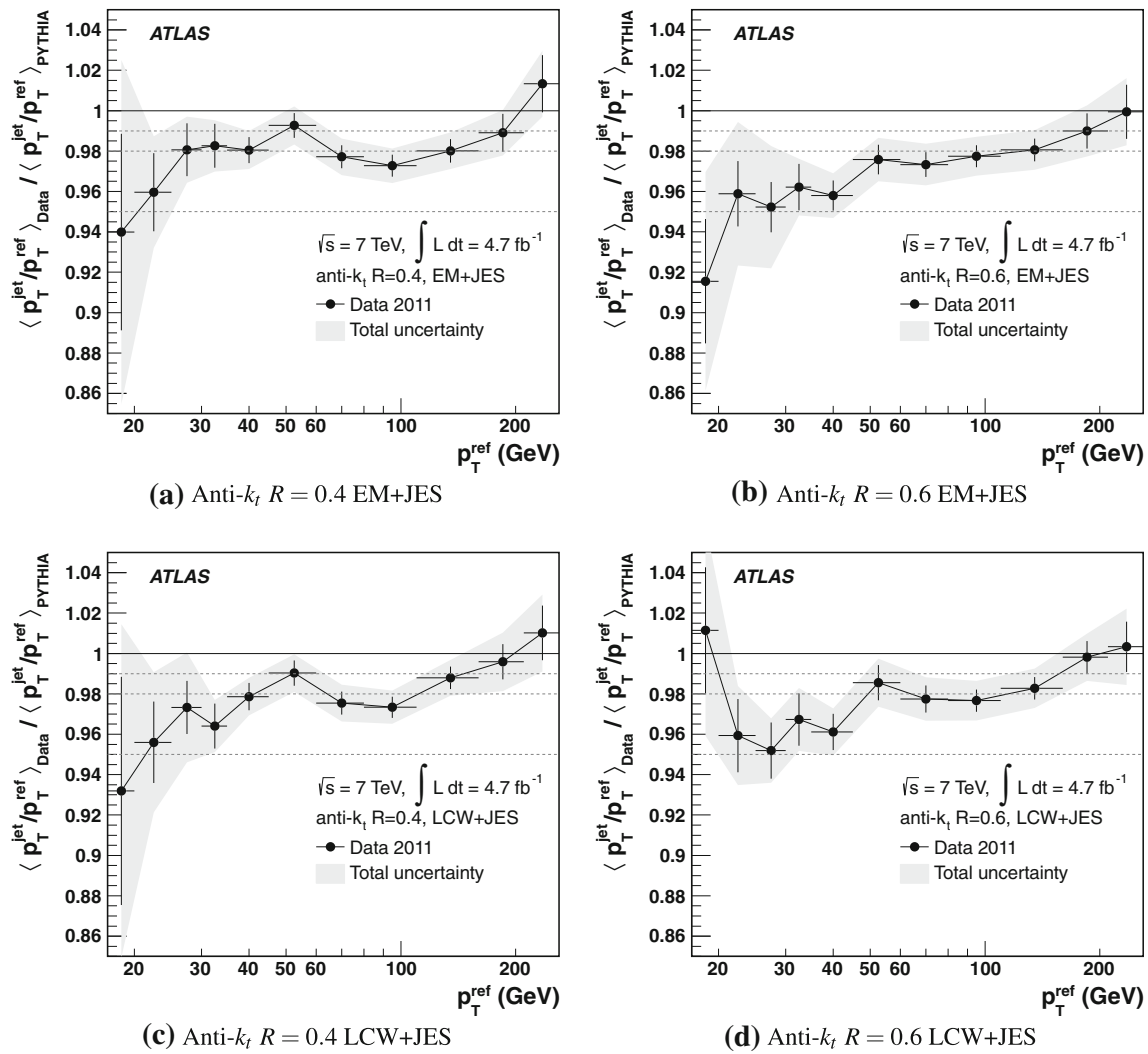
Fig. 20 Data-to-MC ratio of the mean p_T balance for Z-jet events as a function of p_T^{\text{ref}} for anti- k_t jets with distance parameter (a, c) R = 0.4 and (b, d) R = 0.6 calibrated with the (a, b) EM+JES and the (c, d)
