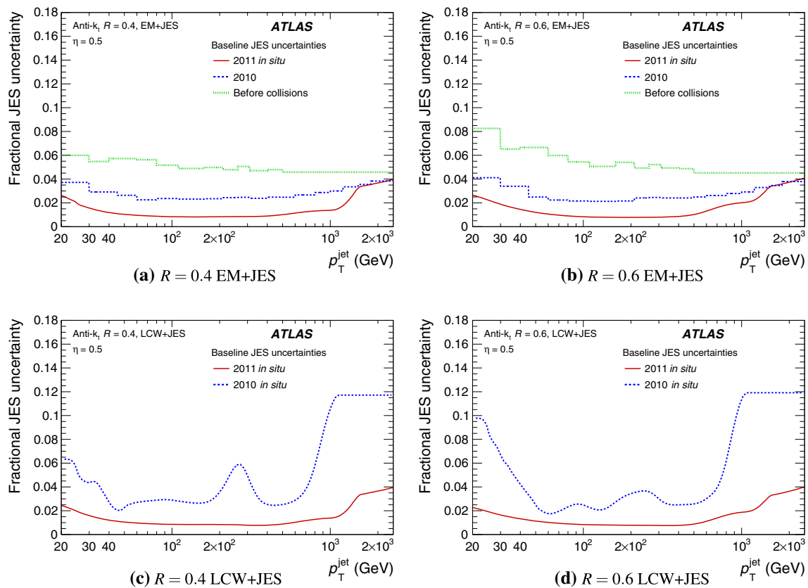
Fig. 66 Fractional jet energy scale systematic uncertainty for inclusive jets as a function of p_T^{\text{jet}} for jets with a, c R = 0.4 and b, d R = 0.6 calibrated with the a, b EM+JES and c, d LCW+JES schemes and with \eta = 0.5
