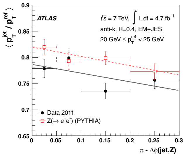
Fig. 16 Mean p_T^{\text{jet}}/p_T^{\text{ref}} balance vs \Delta\phi(\text{jet}, Z) for 20 \leq p_T^{\text{ref}} < 25 \text{ GeV} in the data and in the simulation. A linear function used to extrapolate the balance to \Delta\phi = \pi is superimposed. Anti- k_t jets with distance parameter R = 0.4 calibrated with the EM+JES scheme are used. Only statistical uncertainties are shown
