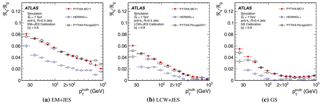
Fig. 51 Difference in jet response \mathcal{R} = p_T^{\text{jet}}/p_T^{\text{truth}} of isolated jets initiated by light quarks and gluons as a function of the true jet p_T , for anti- k_t jets with R = 0.4 in the barrel calorimeter. Three different calibration schemes are shown for a the EM+JES calibration, b the LCW+JES
