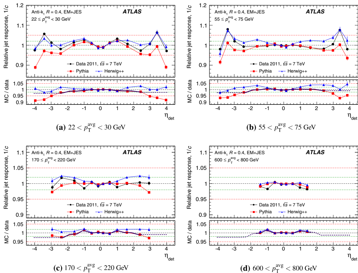
Fig. 11 Relative jet response ( 1/c ) as a function of the jet pseudorapidity for anti- k_t jets with R = 0.4 calibrated with the EM+JES scheme, separately for a 22 \leq p_T^{\text{avg}} < 30 GeV, b 55 \leq p_T^{\text{avg}} < 75 GeV, c 170 \leq p_T^{\text{avg}} < 220 GeV and d 600 \leq p_T^{\text{avg}} < 800 GeV. The lower parts of the figures show the ratios between the data and MC relative
