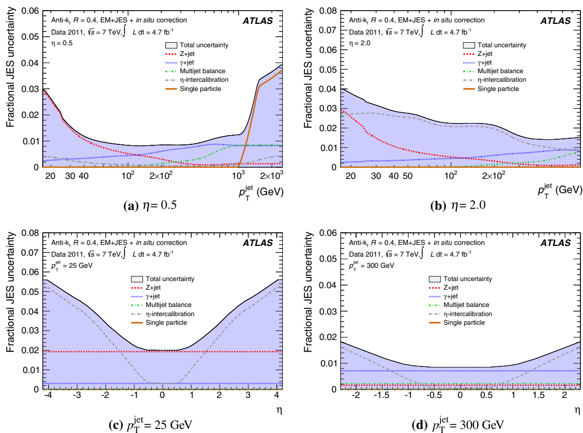
Fig. 59 Fractional in situ jet energy scale systematic uncertainty as a function of a, b p_T^{\text{jet}} and c, d jet pseudorapidity for anti- k_t jets with distance parameter of R = 0.4 calibrated using the EM+JES calibration scheme. The contributions from each in situ method are shown separately. Uncertainties from pile-up, flavour, and topology are not included
