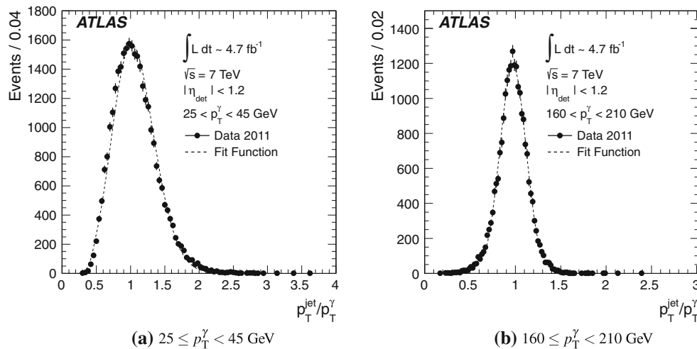
Fig. 22 Jet response distributions in the \gamma -jet data for a 25 \leq p_T^\gamma < 45 \text{ GeV} and b 160 \leq p_T^\gamma < 210 \text{ GeV} as measured by the DB technique for anti- k_t jets with R = 0.6 at the EM+JES scale. The dashed lines represent fits of Gaussian functions, except in the lowest bin
