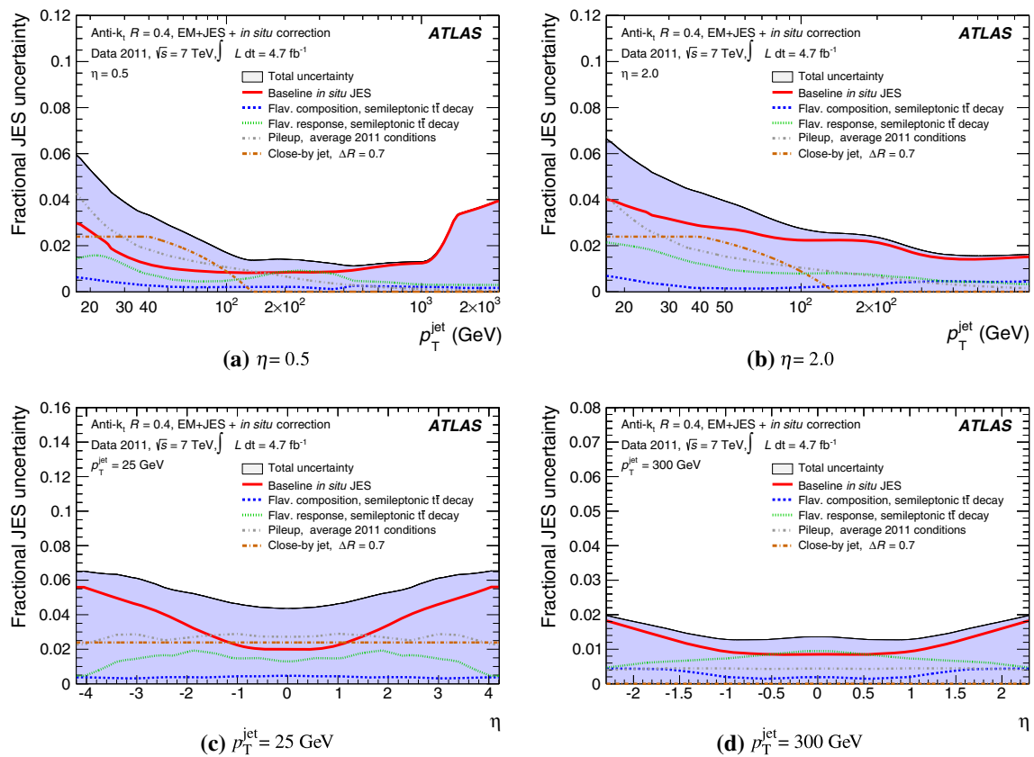
Fig. 61 Sample-dependent fractional jet energy scale systematic uncertainty as a function of a , b p_T^{\text{jet}} and c , d jet pseudorapidity for anti- k_t jets with distance parameter of R = 0.4 calibrated using the EM+JES
