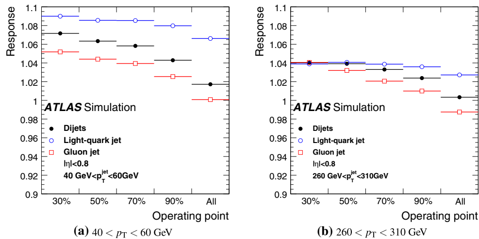
Fig. 52 Jet p_T response for the two leading jets in the dijet sample for different tagger light-quark operating points for jets with a 40 \text{ GeV} < p_T < 60 \text{ GeV} and b 260 \text{ GeV} < p_T < 310 \text{ GeV} , and
