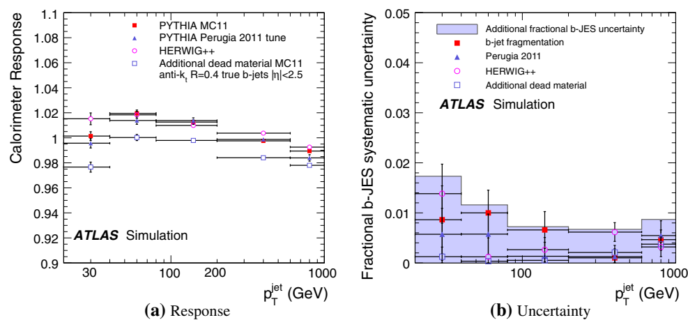
Fig. 53 Average response to b -jets in some of the different samples used to calculate the b -jet energy scale systematic uncertainties is depicted in a . The resulting uncertainties in the ratio of the b -jet response
