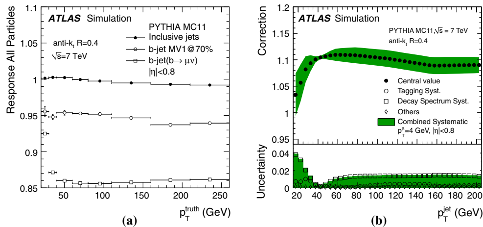
Fig. 56 Average jet response as a function of true transverse momentum of jets built using all stable particles, for a sample of inclusive jets (solid circles), a sample of b -jets tagged with the MV1 tagging algorithm (open circles) and a sample of semileptonically decaying b -jets with a reconstructed muon inside (open squares), is shown in a . The
