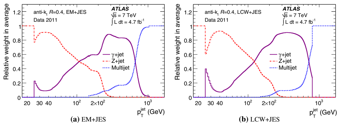
Fig. 36 Weight carried by each in situ technique in the combination to derive the residual jet energy scale calibration as a function of the jet transverse momentum p_T^{\text{jet}} for anti- k_t jets with R = 0.4 calibrated with
