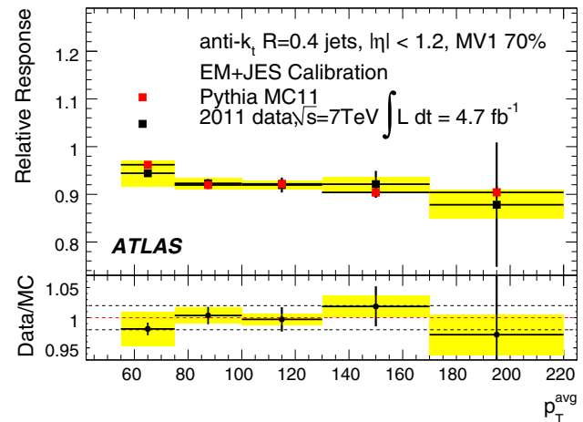
Fig. 57 Relative response of the semileptonic sample with respect to the inclusive b -jet sample as calculated from the dijet p_T asymmetry. The uncertainty band around the data denotes systematic uncertainties in the asymmetry measurement
