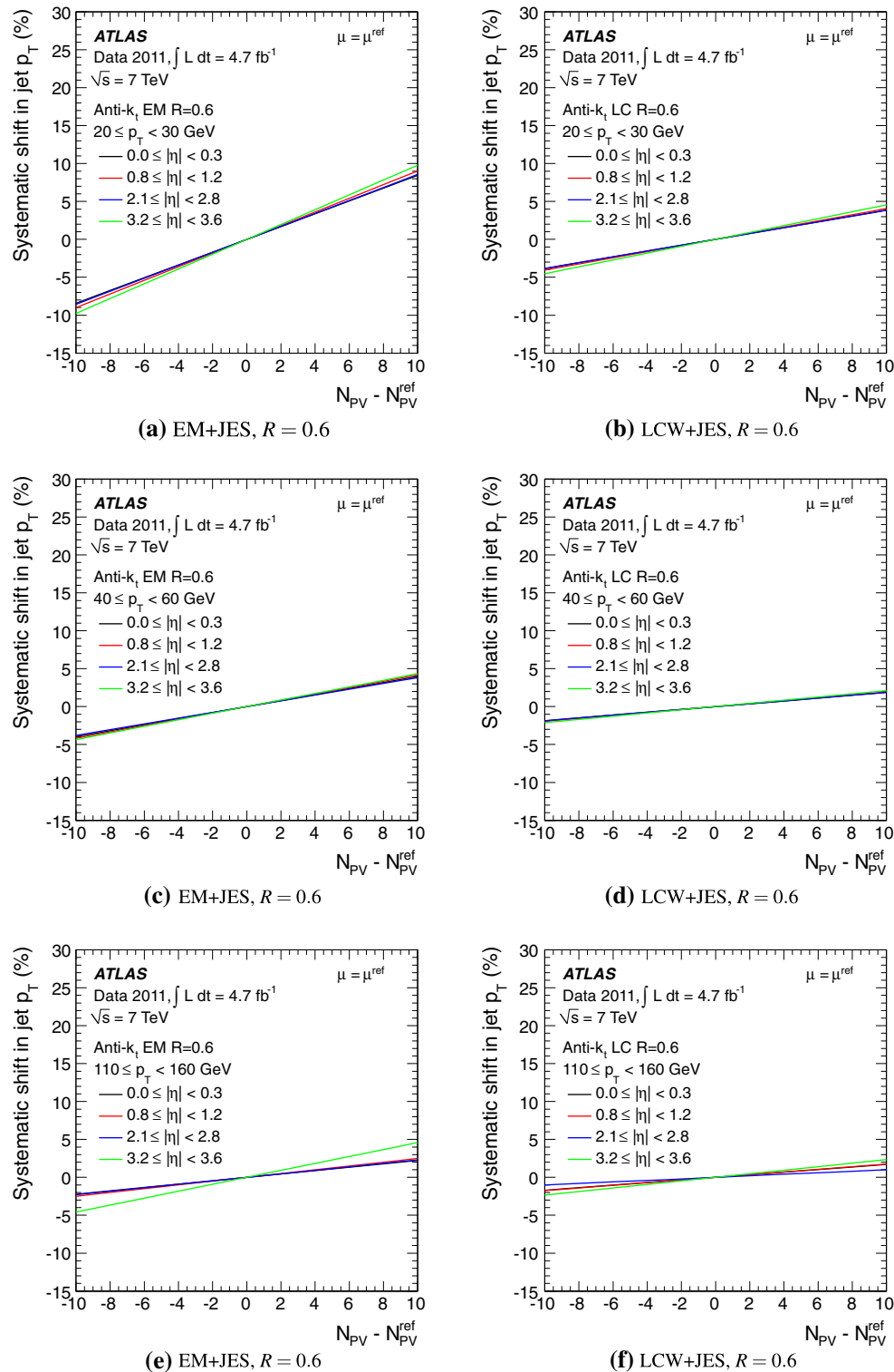
Fig. 47 The fractional systematic shift due to mis-modelling of the effect of in-time pile-up on the transverse momentum p_{T,EM+JES}^{\text{jet}} of jets reconstructed with the anti- k_t algorithm with R = 0.6 and calibrated with the EM+JES scheme, is shown as a function of (N_{PV} - N_{PV}^{\text{ref}}) in a ,
