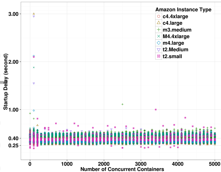
Figure 12. The container start up delay for running 1 to 5000 concurrent containers in each of the studied Amazon EC2 instances.
