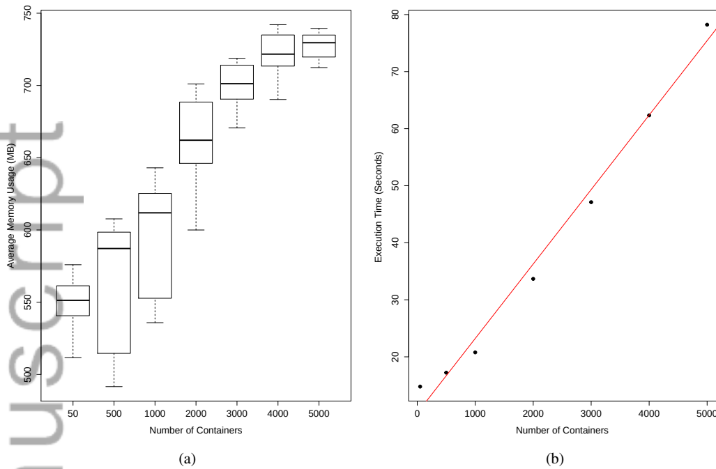
Figure 13. Impact of increasing the number of containers on the average memory usage and the execution time of the simulator.
