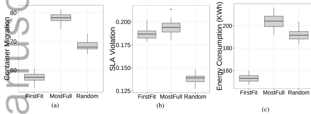
Figure 11. Impact of initial container placement algorithm on the container migration rate (per 5 minute), SLA violations, and data center energy consumption.
