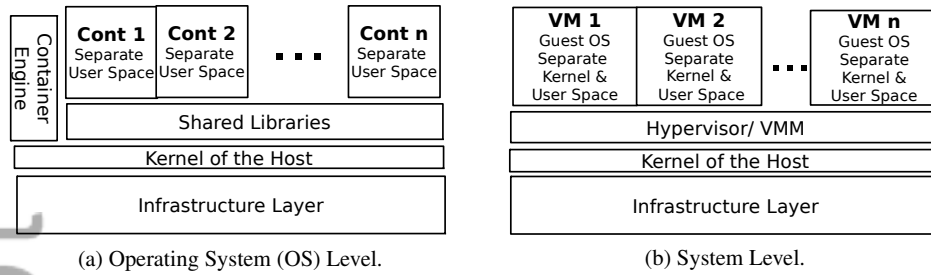
Figure 1. OS level versus System level virtual environments.
