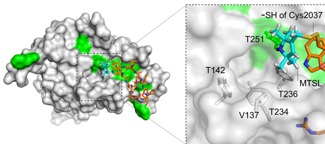
Figure 3. Surface representation of N*bcRON2hp complexed with FVO Pf AMA1. The MTSL spin label (cyan) of the peptide probe (orange stick) projects towards the hot spot at the centre of the cleft (green). Some hot spot forming residues flanked at one side of the druggable hot spot are highlighted in sticks in the enlarged box.
