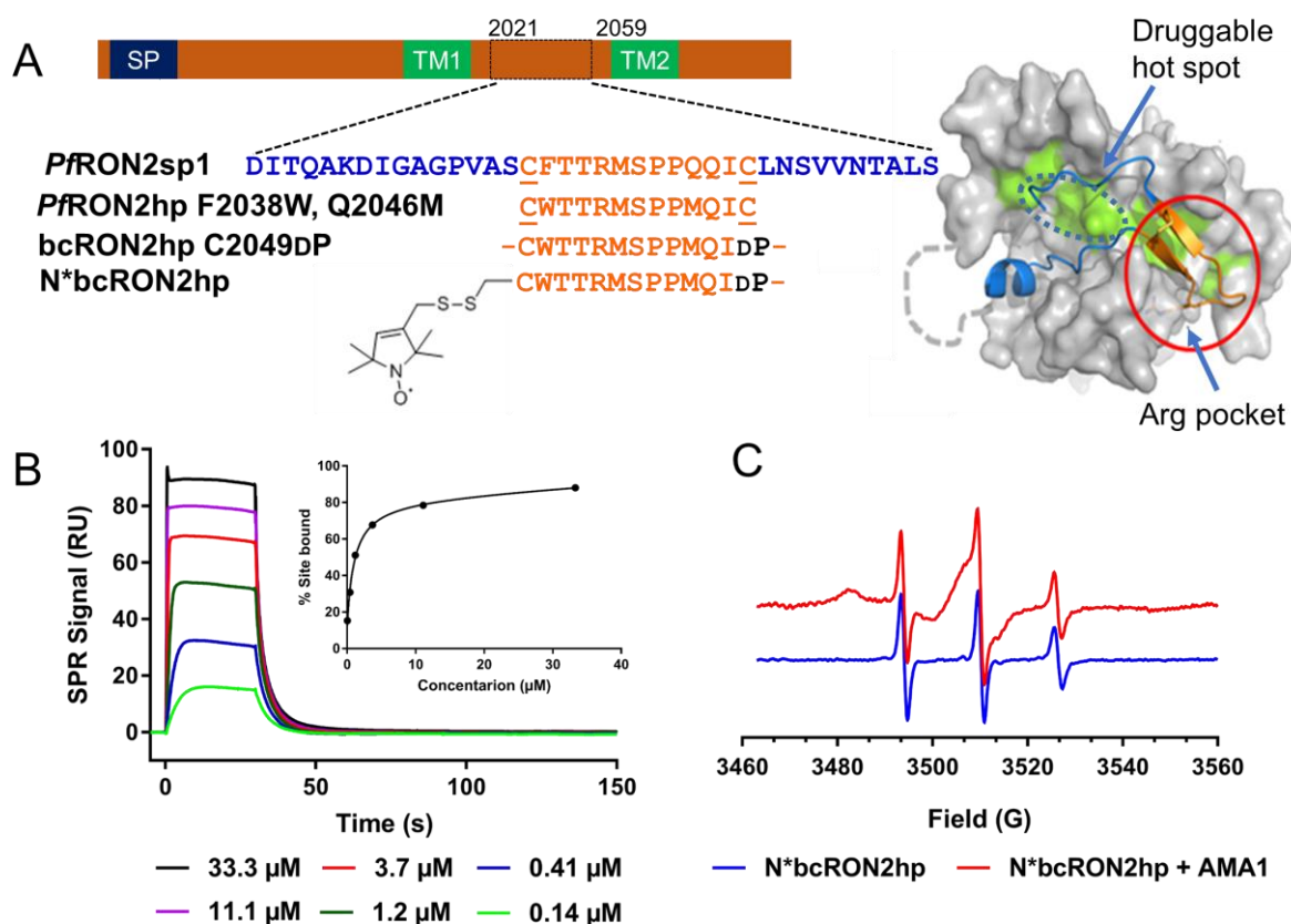
Figure 1. Design and development of the spin-labelled peptide as probe. A. Schematic overview of Pf RON2 protein. SP, signal peptide. TMD, putative membrane domain. Disulfide-bond-forming cysteines are underlined. The probe is designed based on the truncated RON2 hairpin RON2hp (orange) with two beneficial mutations: Cys2049 is replaced with D-Pro and backbone cyclised with Cys2037 for bcRON2hp. The MTSL spin label is attached to the free -SH of Cys2037 of bcRON2hp. The residues involved in backbone cyclisation are hyphenated. The right-hand panel shows the co-crystal structure of Pf AMA1 with Pf RON2sp1 peptide (PDB id: 3ZWZ) [35] reproduced from Wang et al. [31] Pf AMA1 is represented as grey surface. The hydrophobic cleft of AMA1 is highlighted in green with the druggable hot spot dashed circled and arrowed. The domain II loop of Pf AMA1 that is displaced on Pf RON2sp1 binding is depicted as a broken grey line. The \beta -hairpin of Pf RON2 (RON2hp, residues 2037-2049) coloured in orange and circled in red, binds to the polar Arg pocket (arrowed); the rest of the peptide is coloured in blue. B. SPR analysis of N*bcRON2hp binding to immobilized FVO Pf AMA1. C. First harmonic EPR spectra showing sharper line shape of N*bcRON2hp in the free state (blue), which broadens when bound to FVO Pf AMA1 (orange).
