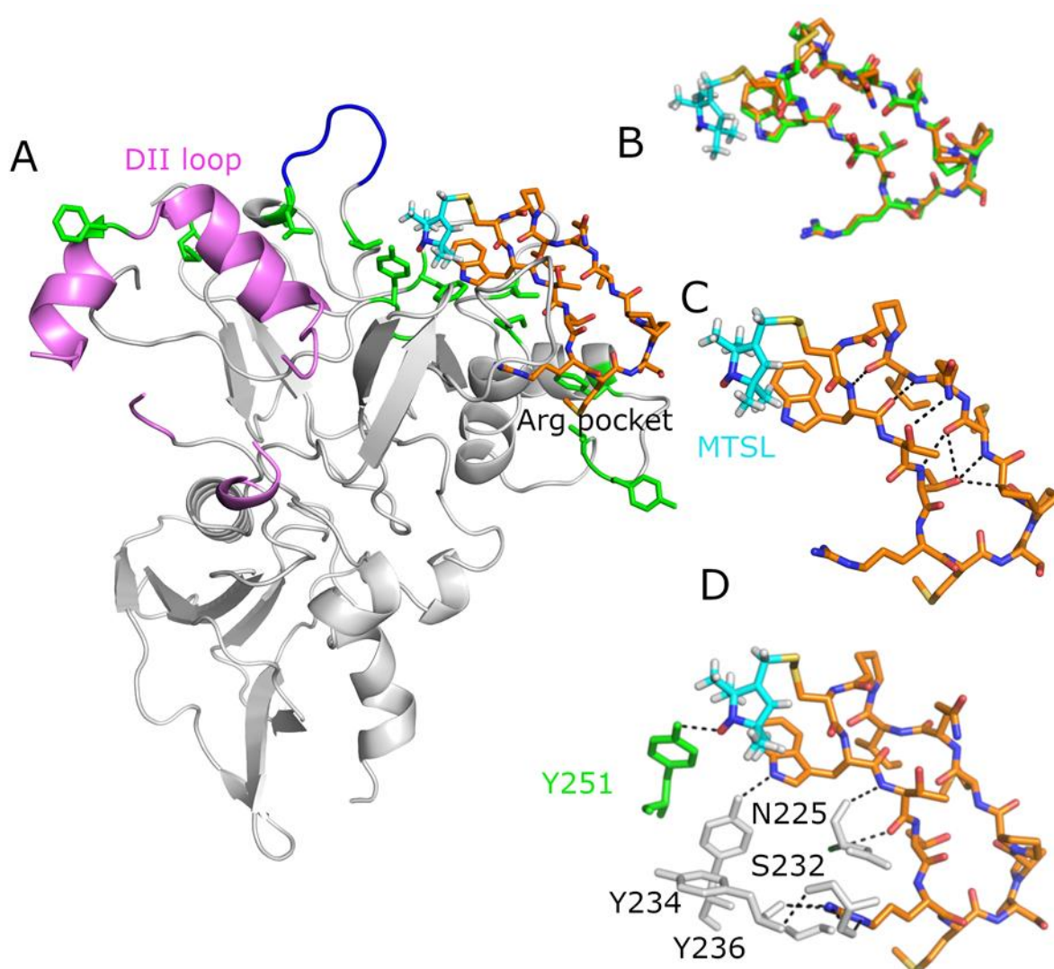
Figure 2. Crystal Structure of N*bcRON2hp complexed with FVO Pf AMA1. A. Cartoon representation of N*bcRON2hp-bound FVO Pf AMA1 structure. The spin-labelled peptide is situated at one end of the hydrophobic cleft, and occupies the polar Arg pocket opposite to the DII loop
