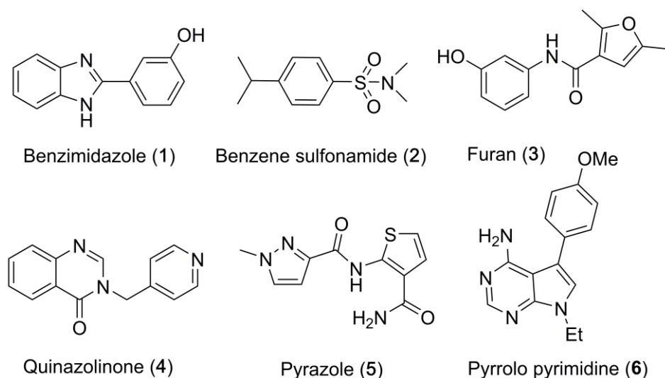
Figure 5. Fragment hits from representative scaffold series screened in the presence of N*bcRON2hp and AMA1.
