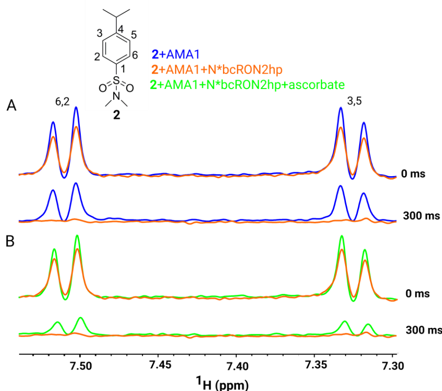
Figure 7. NMR profile of benzene sulfonamide (2) in PRE-based screening. A. CPMG spectra are shown at spin-lock periods of 0 and 300 ms. AMA1-bound fragment signal (blue) is broadened in the presence of N*bcRON2hp (orange) owing to PRE. B. Recovery of signals upon reduction of the paramagnetic nitroxide to the diamagnetic state by ascorbate (green vs orange). Spectra were acquired at 10 °C with 128 scans. Concentrations of 2 , N*bcRON2hp and AMA1 were 50, 3 and 10 μM, respectively.
