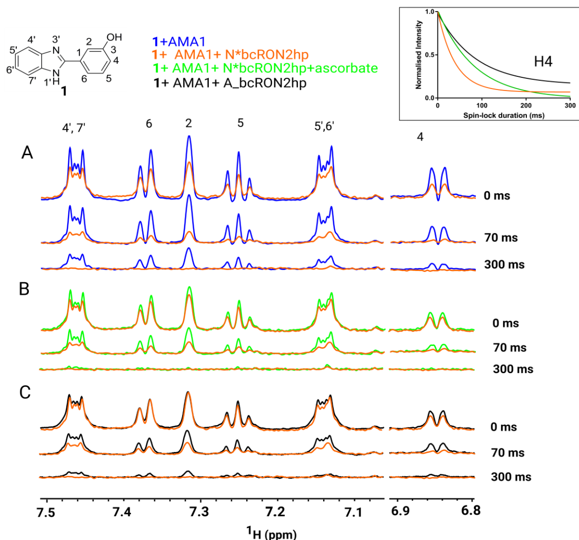
Figure 6. PRE based screening of benzimidazole (1). A. CPMG spectra are shown at spin-lock periods of 0, 70 and 300 ms. AMA1-bound fragment signal (blue) is broadened in the presence of N*bcRON2hp (orange) owing to PRE. B. Recovery of signals upon reduction of the paramagnetic nitroxide to the diamagnetic state by ascorbate (green vs orange) and C. in a separate study with the peptide without the spin-label, A_bcRON2hp (black vs orange). The concentrations used in each experiment were 50 \mu\text{M} 1 , 10 \mu\text{M} Pf AMA1 FVO, 3 \mu\text{M} N*bcRON2hp and 3 \mu\text{M} A_bcRON2hp. Spectra were acquired at 10 ^{\circ}\text{C} with 128 scans. The inset shows best fit to a single exponential for paramagnetic (orange) and diamagnetic (green and black represent ascorbate and A_bcRON2hp, respectively) samples by least squares method using Prism. Enhanced relaxation of proton H4 in the paramagnetic state slowed down upon conversion to the diamagnetic state.
