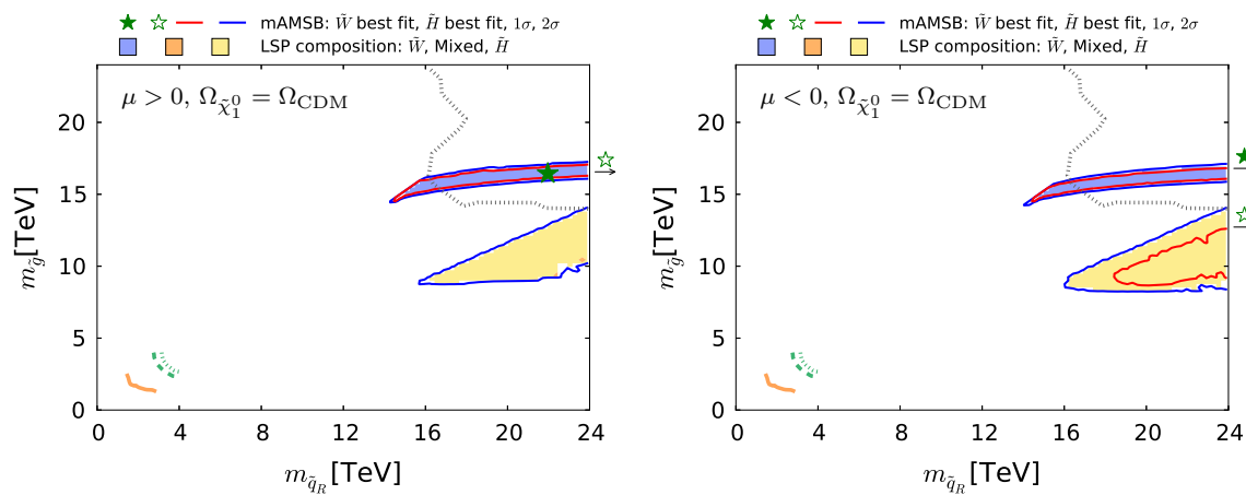
Fig. 25 The region of the (m_{\tilde{q}_R}, m_{\tilde{g}}) plane allowed in the \Omega_{\tilde{\chi}_1^0} = \Omega_{\text{CDM}} case for \mu > 0 (left) and \mu < 0 (right). The orange solid line represents the LHC 8-TeV 95% CL exclusion [138]. The green dashed and dotted lines show the projection estimated by ATLAS [140] for
