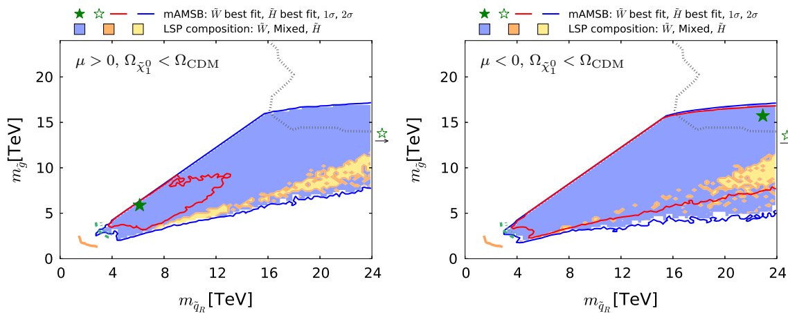
Fig. 21 The region of the (m_{\tilde{q}_R}, m_{\tilde{g}}) plane allowed in the \Omega_{\tilde{\chi}_1^0} \leq \Omega_{CDM} case for \mu > 0 (left) and \mu < 0 (right). The orange solid line represents the LHC 8-TeV 95% CL exclusion [138]. The green dashed and dotted lines show the projection estimated by ATLAS [140] for
