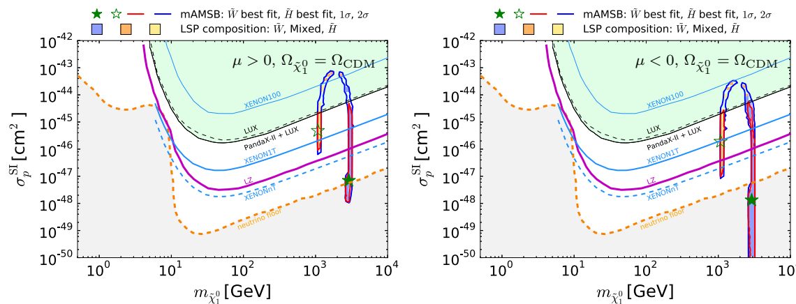
Fig. 26 The (m_{\tilde{\chi}_1^0}, \sigma_p^{\text{SI}}) planes in the mAMSB for \mu > 0 (left) and \mu < 0 (right) in the case when the LSP accounts for the whole DM density. The red and blue solid lines are the 1 and 2 \sigma CL contours, and the solid purple and blue lines show the projected 95% exclusion sensitivities of the LUX-Zeplin (LZ) [153] and XENON1T/nT experiments [154, 155],
