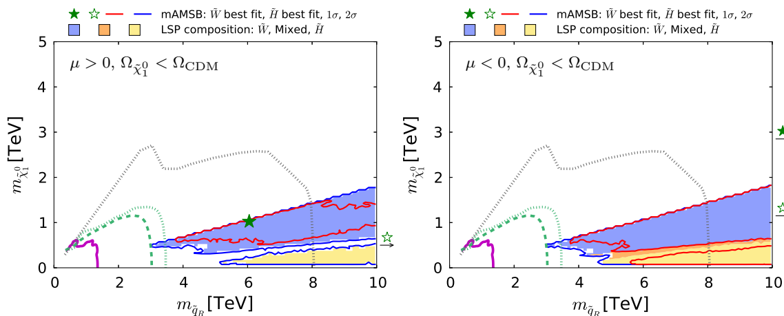
Fig. 22 The region of the (m_{\tilde{q}_R}, m_{\tilde{\chi}_1^0}) plane allowed in the \Omega_{\tilde{\chi}_1^0} \leq \Omega_{CDM} case for \mu > 0 (left) and \mu < 0 (right). The purple solid line represents the ATLAS 13-TeV 95% CL exclusion using 13 fb^{-1} of data [139]. The green dashed and dotted lines show the projected 95% CL sensitivity estimated by ATLAS [141] for 14-TeV data with integrated luminosities of 300 and 3000 fb^{-1} , respectively. The grey dotted
