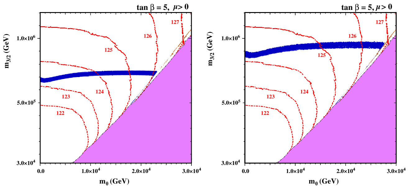
Fig. 2 The (m_0, m_{3/2}) plane for \tan \beta = 5 without (left panel) and with (right panel) the Sommerfeld enhancement, as calculated using SSARD. There are no consistent solutions of the electroweak vacuum conditions in the pink shaded triangular regions at lower right. The
