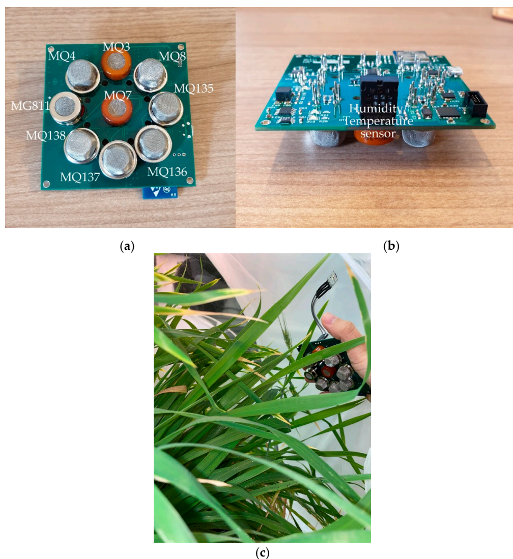
Figure 3. Electronic nose (e-nose) showing (a) the front part with gas sensors and their model ID (Henan Hanwei Electronics Co., Ltd., Henan, China) and (b) the back part which holds the humidity/temperature sensor; (c) Shows the e-nose positioning while taking measurements.
