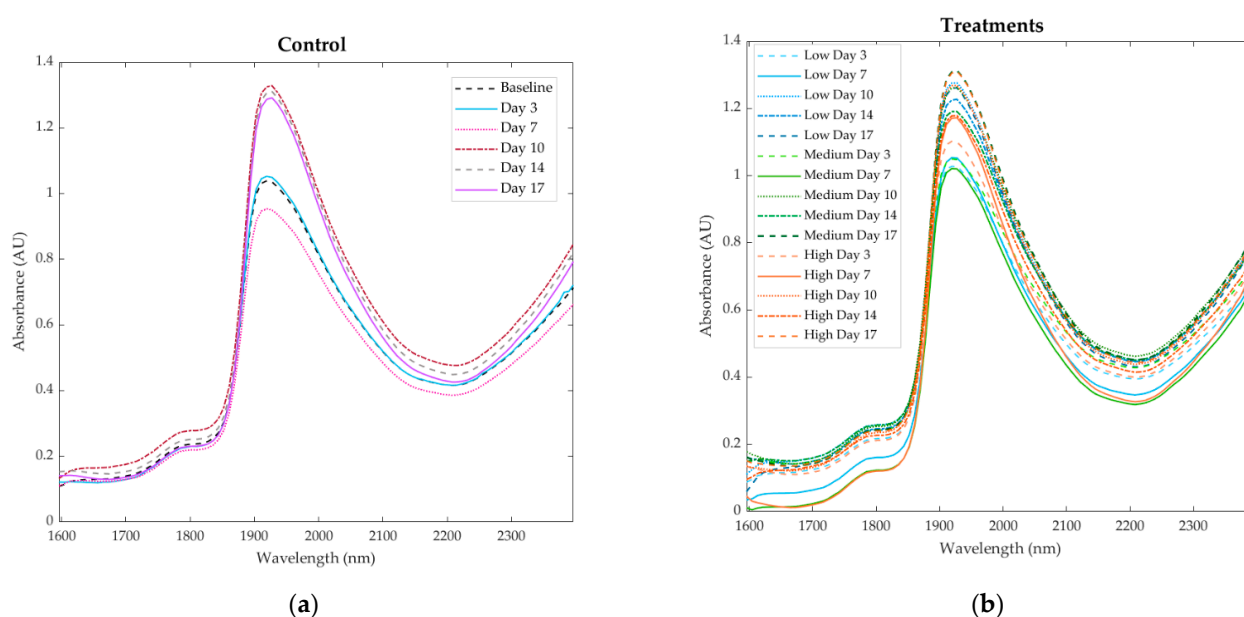
Figure 5. Near-infrared curves showing the absorbance values within the 1596–2396 nm wavelength range for (a) the control measurements and (b) the treatments (low, medium, high infestation) measured at different dates.
