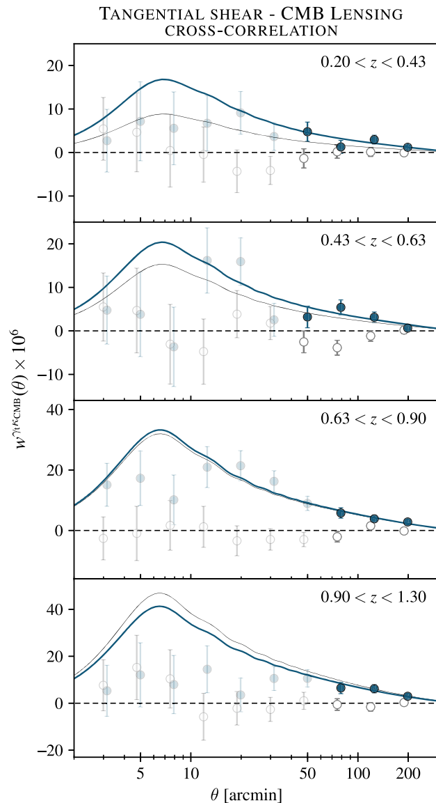
FIG. 2. Measurements of w^{\gamma_i \kappa_{\text{CMB}}}(\theta) (filled circles) and w^{\gamma_i \times \kappa_{\text{CMB}}}(\theta) (open circles) using METACALIBRATION shear estimates and the SPT+ Planck CMB lensing map. The four panels show results for the four source galaxy redshift bin. Faded points are removed from the final analysis due to systematics or uncertainties in the modeling. Also shown are the theoretical predictions using fiducial cosmology with A = 1 (black curves), and with best-fit A (blue curves), where A is defined in Sec. VI A.
