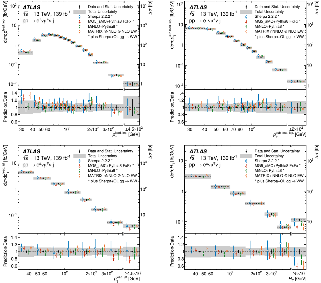
Figure 6. Measured fiducial cross-sections of WW +jets production for (from left to right and top to bottom): p_T^{\text{lead, lep.}} , p_T^{\text{sub-lead, lep.}} , p_T^{\text{lead, jet}} , and H_T . The last bin of each distribution is inclusive in the measured observable and the corresponding integrated cross-section is indicated by the right-hand-side axis. The measured cross-section values are shown as points with error bars giving the statistical uncertainty and solid bands indicating the size of the total uncertainty. The results are compared with the NNLO prediction with extra NLO EW corrections and NLO corrections for gg \rightarrow WW production (denoted MATRIX \otimes NLO EW) as well as NLO+PS predictions from SHERPA 2.2.2, MADGRAPH5_aMC@NLO + PYTHIA 8 with FxFx merging, and POWHEG MINLO + PYTHIA 8 for q\bar{q} initial states, combined with SHERPA + OPENLOOPS (LO+PS) for the gg initial state. The SHERPA 2.2.2 + OPENLOOPS prediction is normalized to the total cross-section calculated at NLO in QCD. Theoretical predictions are indicated as markers with vertical lines denoting PDF and scale uncertainties.
