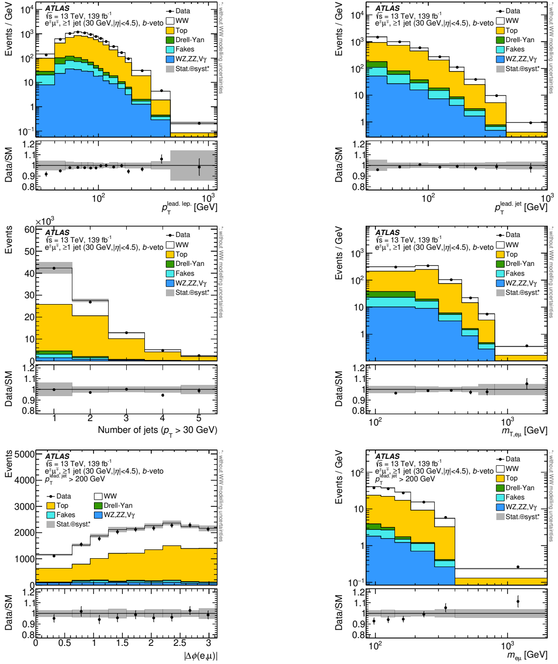
Figure 3. Signal region detector-level distributions of the p_{T}^{\text{lead, lep.}} (top left), the p_{T}^{\text{lead, jet}} (top right), the jet multiplicity (middle left), the m_{T, e\mu} (middle right), and, for events with p_{T}^{\text{lead, jet}} > 200 GeV, the \Delta\phi(e, \mu) (bottom left) and m_{e\mu} (bottom right). Data are shown as black markers together with the predictions for the signal and background production processes. The last bin contains overflow events. The lower panels show the ratio of the data to the total prediction. The uncertainty bands shown include statistical and systematic uncertainties, excluding theory uncertainties on the signal.
