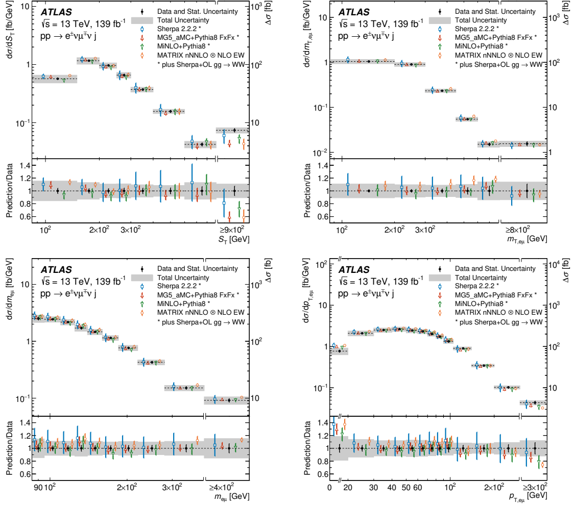
Figure 7. Measured fiducial cross-sections of WW +jets production for (from left to right and top to bottom): S_T , m_{T,e\mu} , m_{e\mu} , and p_{T,e\mu} . The last bin of each distribution is inclusive in the measured observable and the corresponding integrated cross-section is indicated by the right-hand-side axis. The measured cross-section values are shown as points with error bars giving the statistical uncertainty and solid bands indicating the size of the total uncertainty. The results are compared with the NNLO prediction with extra NLO EW corrections and NLO corrections for gg \rightarrow WW production (denoted MATRIX \otimes NLO EW) as well as NLO+PS predictions from SHERPA 2.2.2, MADGRAPH5_aMC@NLO + PYTHIA 8 with FxFx merging, and POWHEG MINLO + PYTHIA 8 for q\bar{q} initial states, combined with SHERPA + OPENLOOPS (LO+PS) for the gg initial state. The SHERPA 2.2.2 + OPENLOOPS prediction is normalized to the total cross-section calculated at NLO in QCD. Theoretical predictions are indicated as markers with vertical lines denoting PDF and scale uncertainties.
