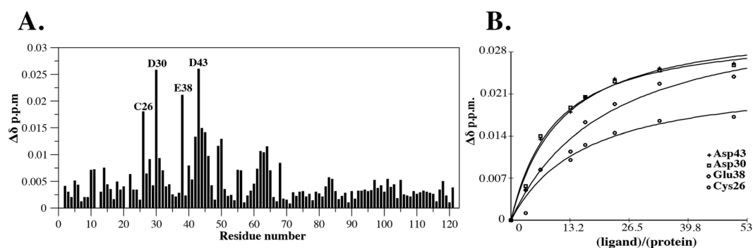
Figure 5. (A) Plot of the change in average ^1\text{H} and ^{15}\text{N} chemical shifts following titration of ^{15}\text{N} -RXFP 1 ( 1-72 ) P4F with 50 equivalents of truncated relaxin. (B) Single-site saturation binding curves ( K_d = 330 \pm 10 \mu\text{M} ) for the resonances that show the largest chemical shift changes and remained resolved throughout the titration.
