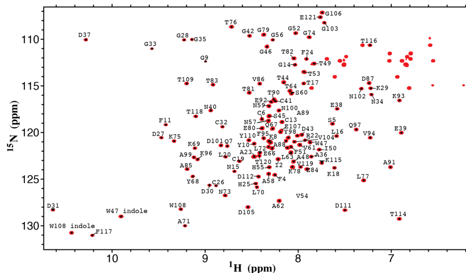
Figure 4. Full ^1\text{H}/^{15}\text{N} HSQC spectrum of RXFP 2 ( 1-65 ) P4F with residue assignments. Unmarked resonances in the upper right corner belong to Asn and Gln sidechains and have not been assigned. Residues I2 to E66 correspond to the LDLa-linker while residues Q67 to E121 belong to the GB1 module.
