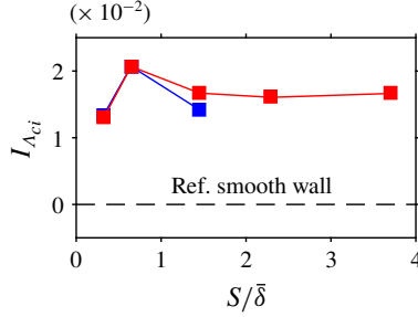
FIGURE 12. Integrated mean swirl strength I_{\Lambda_{ci}} as a function of S/\bar{\delta} . I_{\Lambda_{ci}} of counterclockwise (—■—, red) and clockwise (—■—, blue) roll modes inside the FOV (if any). Dashed line (---) is the reference smooth-wall case (SW-2).
