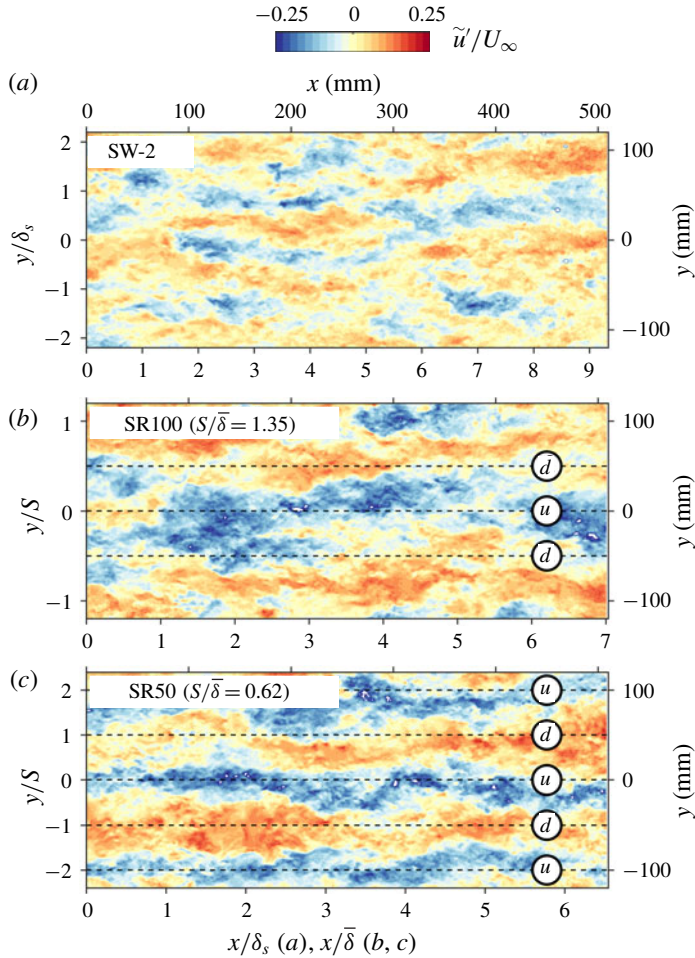
FIGURE 16. Snapshot of \tilde{u}' (turbulent fluctuations and mean spanwise variation) for (a) the reference smooth-wall case SW-2, (b) SR100 and (c) SR50, taken from WPIV measurements. Dashed lines are the spanwise locations related to the common flow up (ⓐ) and common flow down (ⓓ) of the mean secondary flows.
