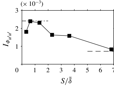
FIGURE 15. Integrated energy spectra I_{\Phi_{u'u'}} as a function of S/\bar{\delta} for SR cases (—■—). Dashed line (---) is reference smooth wall SW-1 and dash-dot line (-·-·-) is reference rough wall RW-2.
