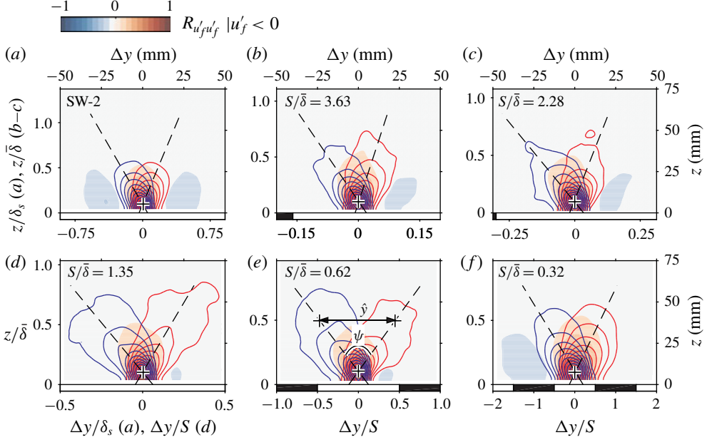
FIGURE 17. Contours of the normalised one-sided two-point correlation coefficient R_{u'_f u'_f} computed for low-speed events only ( u'_f < 0 ), where u'_f is the filtered streamwise velocity fluctuations, for (a) reference smooth-wall case SW-2, (b) SR250-2, (c) SR160, (d) SR100, (e) SR50 and (f) SR25. For heterogeneous cases, correlations are computed at a spanwise location corresponding to the common flow up of the secondary flow ( \textcircled{u} in figure 8). Symbol '+' indicates the reference wall height z_{ref}/\delta_s = 0.1 (a) and z_{ref}/\bar{\delta} = 0.1 (b-f). Red and blue solid contour lines are R_{u'_f u'_f} = 0.1, 0.2, \dots, 0.9 , further conditioned based on the sign of filtered spanwise velocity fluctuations at the reference location: v'_f > 0 (—, red) and v'_f < 0 (—, blue). Dashed line (---) shows the inclination of the v'_f -conditioned correlation maps. In (e), \hat{y} is the distance between v'_f -conditioned correlation maps measured at z/\bar{\delta} = 0.5 and \psi is the angle between the inclination of correlation maps.
