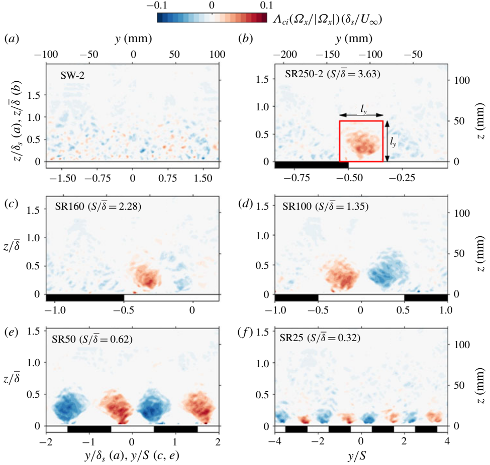
FIGURE 11. Large-scale secondary flows shown by the mean swirl strength A_{ci} multiplied by the sign of vorticity \Omega_x/|\Omega_x| . Red and blue indicate counterclockwise (CCW) and clockwise (CW) secondary flows, respectively. In (b), — illustrates the area of integration in (3.2).
