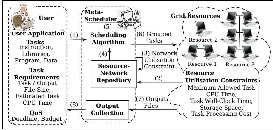
Fig. 2 Grid Entities and the Information Flow.
