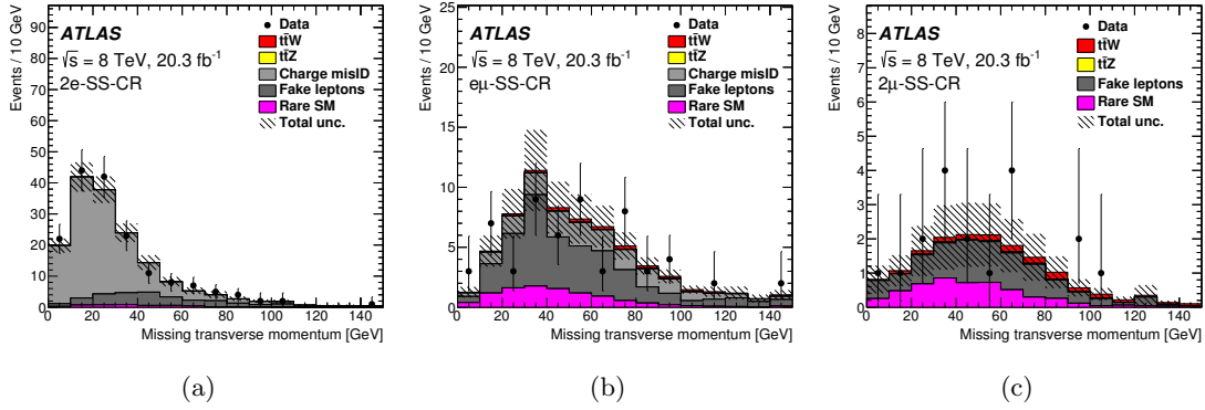
Figure 4. Distributions of E_T^{\text{miss}} for events in a same-sign dilepton control region with H_T < 240 GeV and at least one b -tagged jet for the different lepton flavour combinations, (a) ee , (b) e\mu and (c) \mu\mu . “Rare SM” contains small background contributions mainly consisting of the WW and WZ processes. The predictions are shown before fitting to data in the control region. The instrumental backgrounds, including fake leptons and leptons with misidentified charge are predicted using data-driven methods. The hatched area corresponds to the total uncertainty on the predicted yields. The last bin in each histogram includes the overflow.
