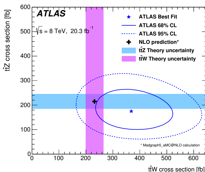
Figure 11. The result of the simultaneous fit to the t\bar{t}W and t\bar{t}Z cross sections along with the 68% and 95% CL uncertainty contours. The shaded areas correspond to 14% uncertainty, which includes renormalisation and factorisation scale uncertainties as well as PDF uncertainties including \alpha_S variations.
