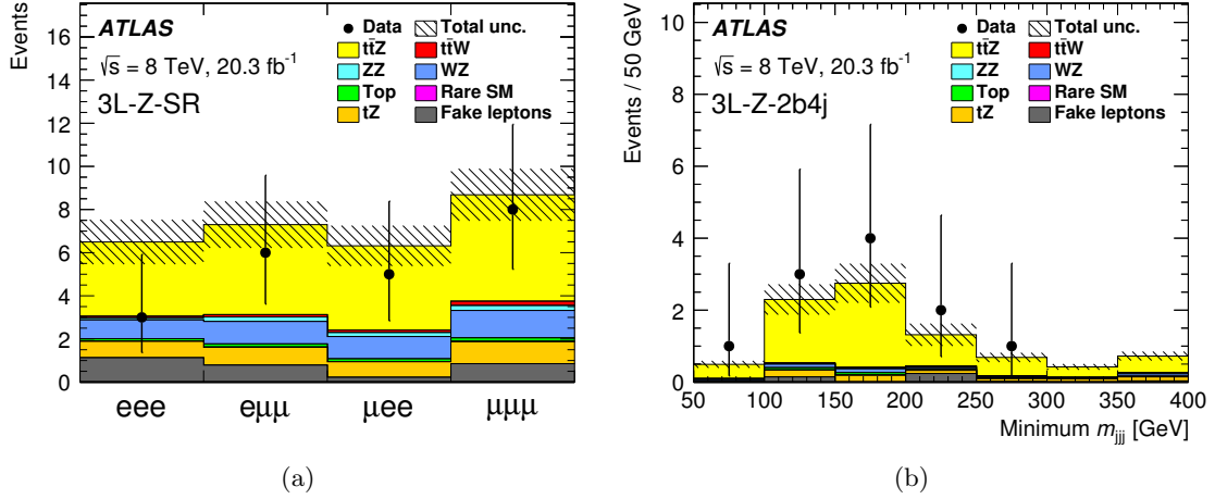
Figure 7. (a) Event yields in the trilepton channel summarising the signal regions with different lepton flavour combinations and (b) the minimum three-jet invariant mass for events in the 3ℓ-Z-2b4j signal region. “Rare SM” contains small background contributions consisting of the WWW , WWZ , H \rightarrow ZZ and t\bar{t}WW processes. The distributions are shown before the fit. The hatched area corresponds to the total uncertainty on the predicted yields. The last bin in (b) includes the overflow.
