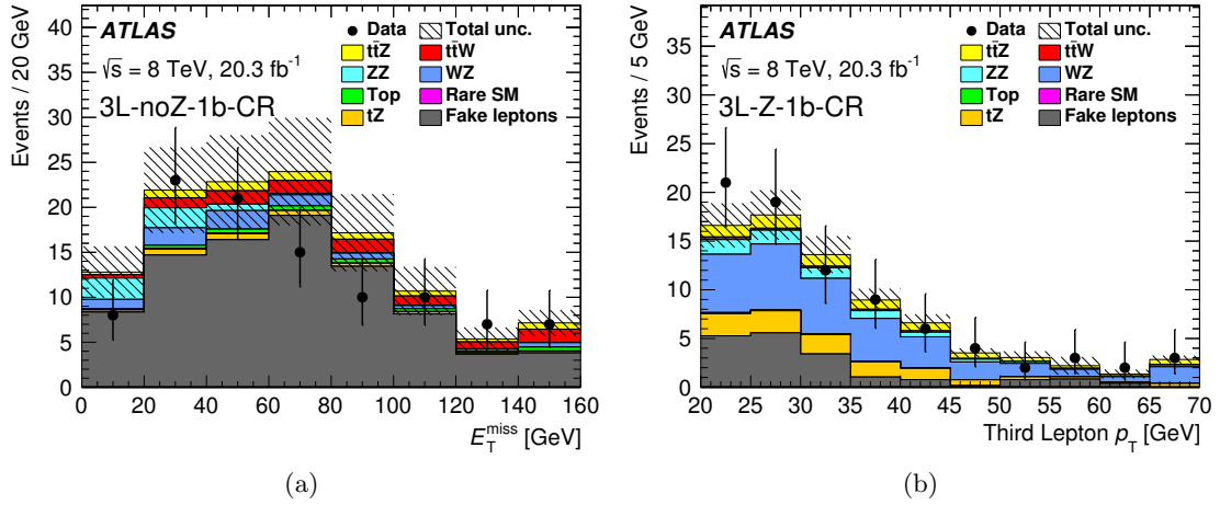
Figure 6. Distributions of (a) E_T^{\text{miss}} in the 3\ell\text{-noZ-1b} region and (b) third-lepton p_T in the 3\ell\text{-Z-1b} region. “Rare SM” contains small background contributions consisting of the WWW , WWZ , H \rightarrow ZZ and t\bar{t}WW processes. The hatched area corresponds to the total uncertainty on the predicted yields. The distributions are shown before the fit. The last bin in each histogram includes the overflow.
