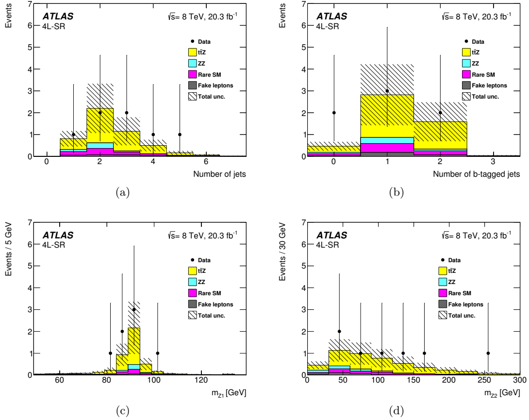
Figure 9. Distributions of (a) number of jets, (b) number of b -tagged jets, invariant mass of the (c) Z_1 and (d) Z_2 dilepton pair for the tetralepton signal region selection. The distributions are shown before the fit. The distributions of the seven observed events are compared to expectation. The hatched area corresponds to the total uncertainty on the predicted yields. “Rare SM” contains small background contributions mainly consisting of the WtZ and t\bar{t}H processes.
