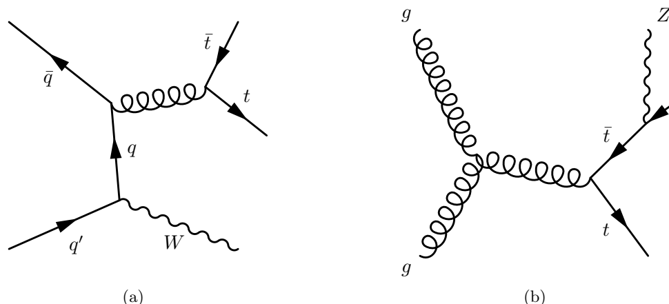
Figure 1. Example leading-order Feynman diagrams for (a) t\bar{t}W and (b) t\bar{t}Z production.
