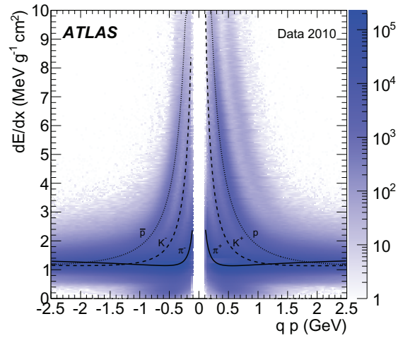
Figure A.8: Greyscale-printing version of Figure 1 (left): Distribution of dE/dx versus charge times momentum for minimum bias collisions in a data sample from 2010. With tracks reconstructed for p_T > 100 MeV this sample is more suitable for the calibration of the Bethe-Bloch function than 2011 data in which tracks had a cutoff of p_T = 400 MeV. The distribution of the most probable value for pions (solid), kaons (dashed) and protons (dotted) are superimposed. The band due to deuterons is clearly visible.
