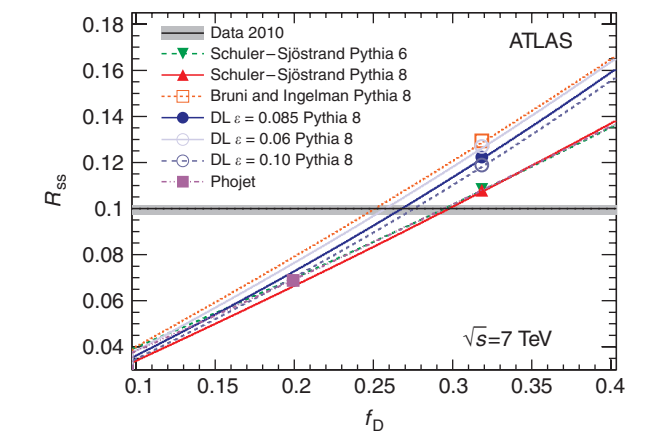
Figure 1 | Dependence of the fraction of single-sided events ( R_{ss} ) on the relative diffractive contribution ( f_D ). The ratio of the single-sided to inclusive event sample R_{ss} as a function of the fractional contribution of diffractive events, f_D , to the inelastic cross-section. The data value for R_{ss} is shown as the horizontal line with its systematic uncertainties (grey band). Also shown are predictions of several models as a function of an assumed value of f_D . For all three DL predictions, the \alpha' value is 0.25\text{ GeV}^{-2} . The default f_D values are indicated by the markers; they are 32.2% for all models except Phojet that uses 20.2%.
