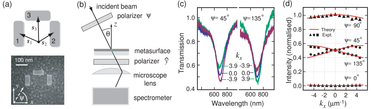
Figure 1. Experiment to measure asymmetric response of metasurface to in-plane wave vector k_x . (a) The configuration of metal rods in the unit cell showing the in-plane coordinates, an SEM image of a WB structure during fabrication and the orientation of the first polarizer. This structure is repeated over the sample surface with a period of 400 nm in both directions; (b) The experiment configuration showing the incident angle \theta , the first polarizer set to angle \psi and the second polarizer aligned with the \hat{y} axis; (c) Experimental spectra from the metasurface for different spatial frequencies k_x and polarizer settings \psi showing the asymmetric response; (d) Comparison between theory (solid lines) and experiment (points) (Figure adapted from Ref. 5 )
