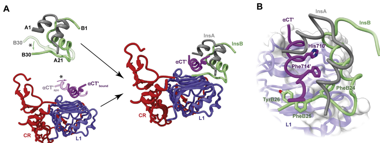
Figure 3: Insulin's engagement with its primary binding site on the receptor. (A) Schematic diagram illustrating both the folding out of the B-chain C-terminal region of insulin from the hormone's core (asterisk, top left), the reconfiguration upon insulin binding of the \alpha CT' helix on the L1- \beta_2 surface (asterisk, bottom left), and insulin's engagement with the L1+ \alpha CT' tandem element (right). (B) Detail of the packing of \alpha CT' residues His710' and Phe714' into the hormone's core as well as the reconfiguration of the three aromatic residues PheB24, PheB25, and TyrB26 within insulin's B-chain C-terminal region. Panels are based on PDB 1MSO [32], PDB 4ZX8 [95] and PDB 6VEP [16].
