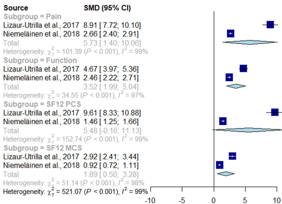
Figure 2. Forest plot of change in patient-reported pain, function, and quality of life (physical health and mental health) following primary total knee replacement (TKR), assessed using standardised mean differences.
